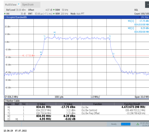
1-N26-824-849--15-5-M-9-CP-256QAM-Outer_Full-2 5@0-Ant0-4.473-4.950-≤5-PASS
