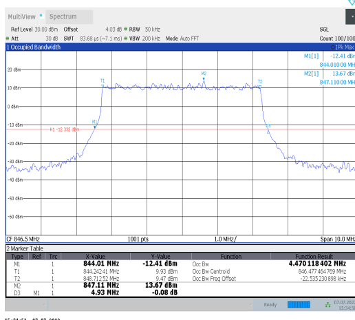
1-N26-824-849--15-5-H-1-DFT-QPSK-Outer_Full-25 @0-Ant0-4.47-4.930-≤5-PASS
