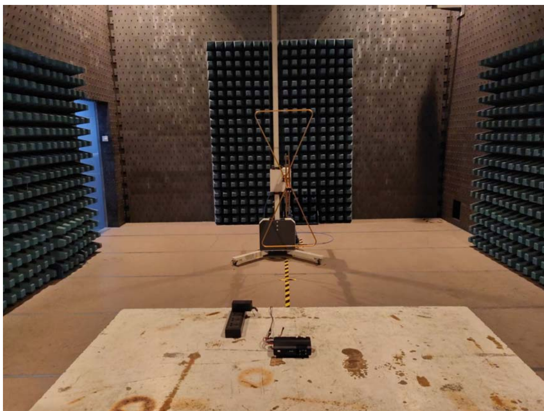
PCB Setup photo
