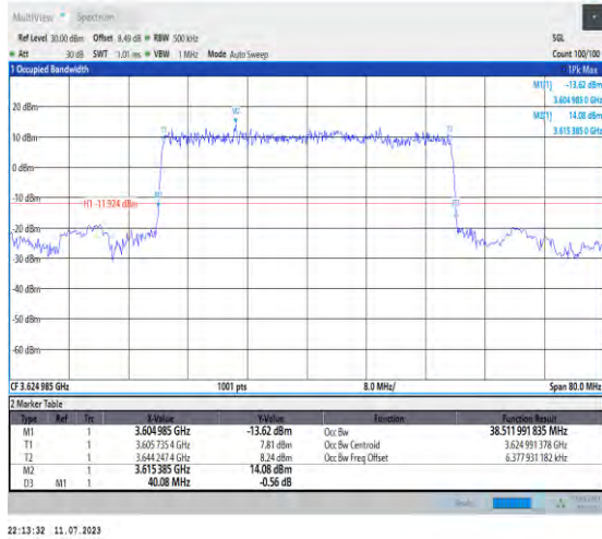
1-N48-PC3-30-40-M-2-DFT-PI2BPSK-Outter_Full-100 @0-Ant3-38.512-40.080-≤40-PASS
