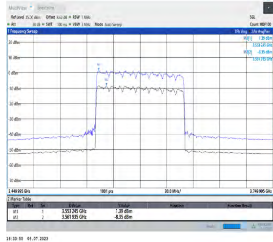
1-N48-PC3-30-100-L-2-CP-256QAM-Outter_Full-273 @0-Ant3-9.74-19.6%-7.08-2.66-PASS-≤13
