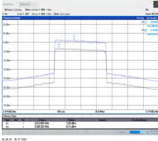
1-N48-PC3-30-100-M-1-DFT-256QAM-Outter_Full-51 @0-Ant3-9.45-19.6%-7.08-2.37-PASS-≤13
