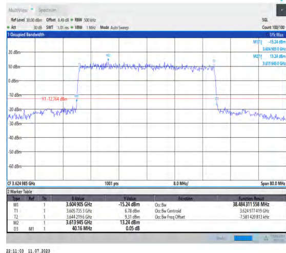
1-N48-PC3-30-40-M-1-DFT-QPSK-Outer_Full-100@0 -Ant3-38.484-40.160-≤40-PASS
