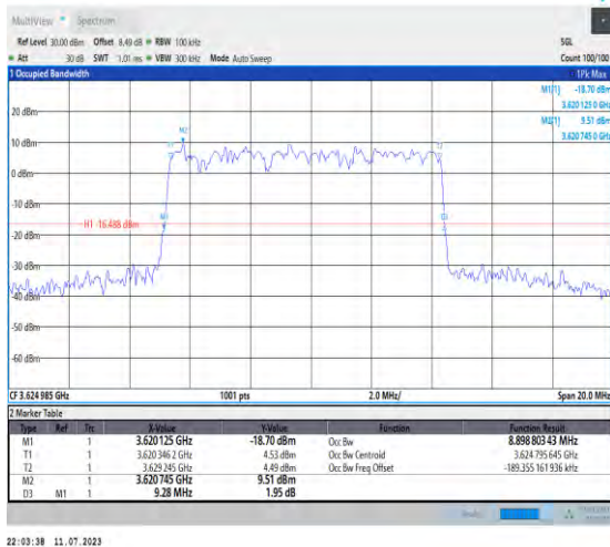
1-N48-PC3-30-10-M-5-DFT-256QAM-Outer_Full-24 @0-Ant3-8.899-9.280≤10-PASS
