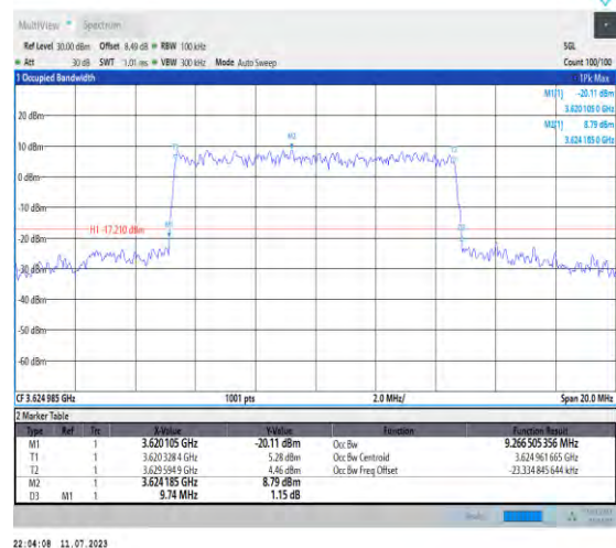
1-N48-PC3-30-10-M-8-CP-64QAM-Outer_Full-24@0 -Ant3-9.267-9.740≤10-PASS
