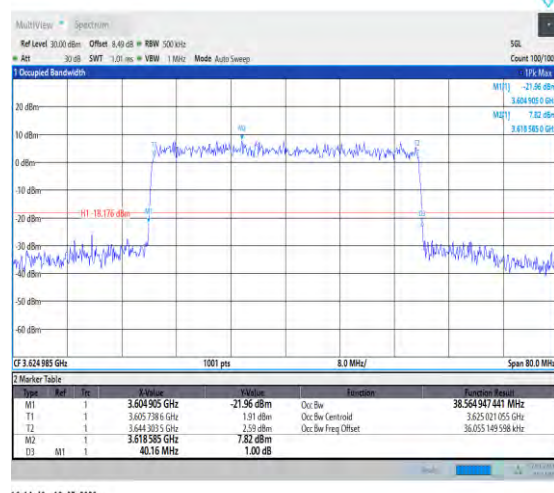
1-N48-PC3-30-40-M-9-CP-256QAM-Outter_Full-106@0-Ant3-38.565-40.160-≤40-PASS
