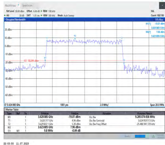
1-N48-PC3-30-10-M-6-CP-QPSK-Outer_Full-24@0- Ant3-9.285-9.800≤10-PASS
