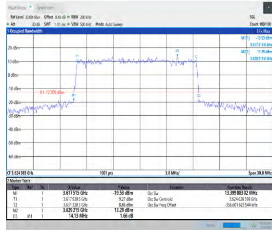
1-N48-PC3-30-15-M-1-DFT-QPSK-Outer_Full-36@0 Ant3-13.4-14.130-≤30-PASS
