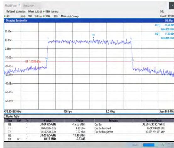
1-N48-PC3-30-40-M-7-CP-16QAM-Outter_Full-106@0-Ant3-38.561-40.160-≤40-PASS
