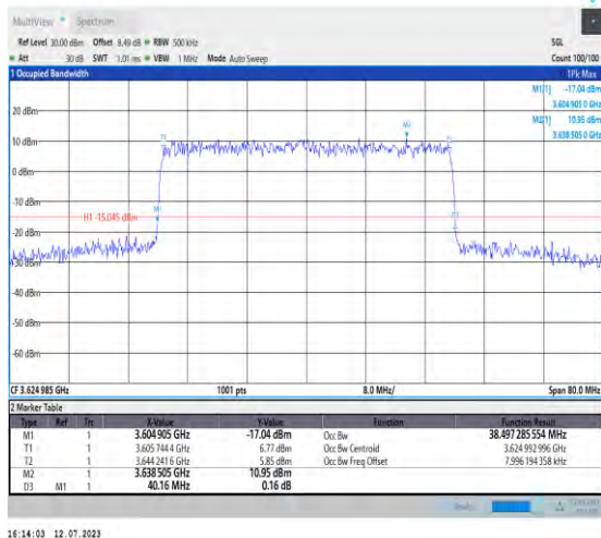
1-N48-PC3-30-40-M-4-DFT-64QAM-Outter_Full-100 @0-Ant3-38.497-40.160-≤40-PASS
