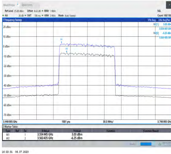
1-N48-PC3-30-100-L-1-DFT-256QAM-Outter_Full-51 @0-Ant3-9.28-19.6%-7.08-2.20-PASS-≤13
