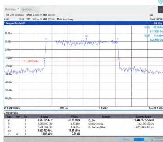
1-N48-PC3-30-15-M-3-DFT-16QAM-Outer_Full-36 @0Ant3-13.445-14.070-≤30-PASS
