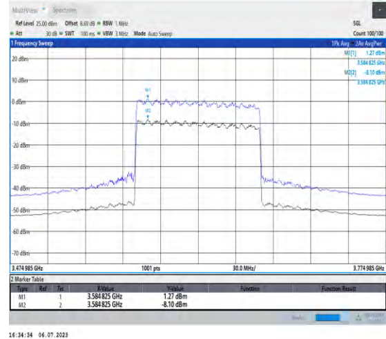
1-N48-PC3-30-100-M-2-CP-256QAM-Outter_Full-273 @0-Ant3-9.37-19.6%-7.08-2.29-PASS-≤13
