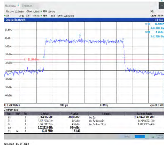
1-N48-PC3-30-40-M-5-DFT-256QAM-Outter_Full-100 0@0-Ant3-38.47-40.160-≤40-PASS
