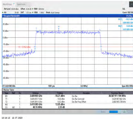
1-N48-PC3-30-40-M-6-CP-QPSK-Outter_Full-106@0 -Ant3-38.588-40.160-≤40-PASS
