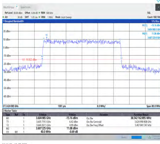
1-N48-PC3-30-40-M-8-CP-64QAM-Outter_Full-106@0-Ant3-38.542-40.000-≤40-PASS
