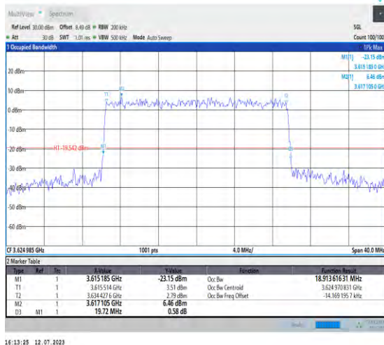
1-N48-PC3-30-20-M-9-CP-256QAM-Outer_Full-51@0 -Ant3-18.914-19.720-≤20-PASS
