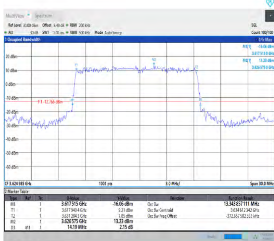
1-N48-PC3-30-15-M-2-DFT-PI2BPSK-Outer_Full-36 @0Ant3-13.344-14.190-≤30-PASS
