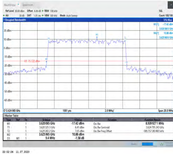
1-N48-PC3-30-10-M-1-DFT-QPSK-Outter_Full-24@0 -Ant3-8.94-9.400-≤10-PASS
