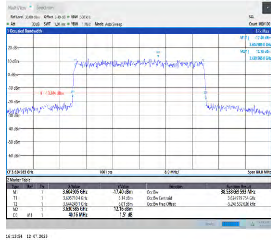
1-N48-PC3-30-40-M-3-DFT-16QAM-Outter_Full-100 @0-Ant3-38.539-40.160-≤40-PASS
