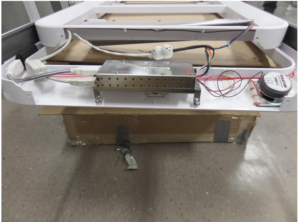
Photograph 33. NP10 top view cellular modem Bluetooth
