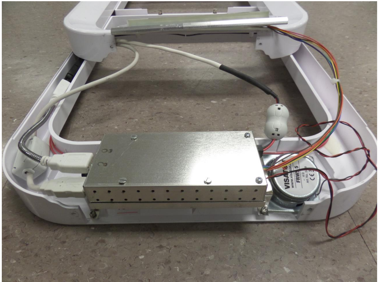
Photograph 34. NP20 top side view Cellular modem Bluetooth
