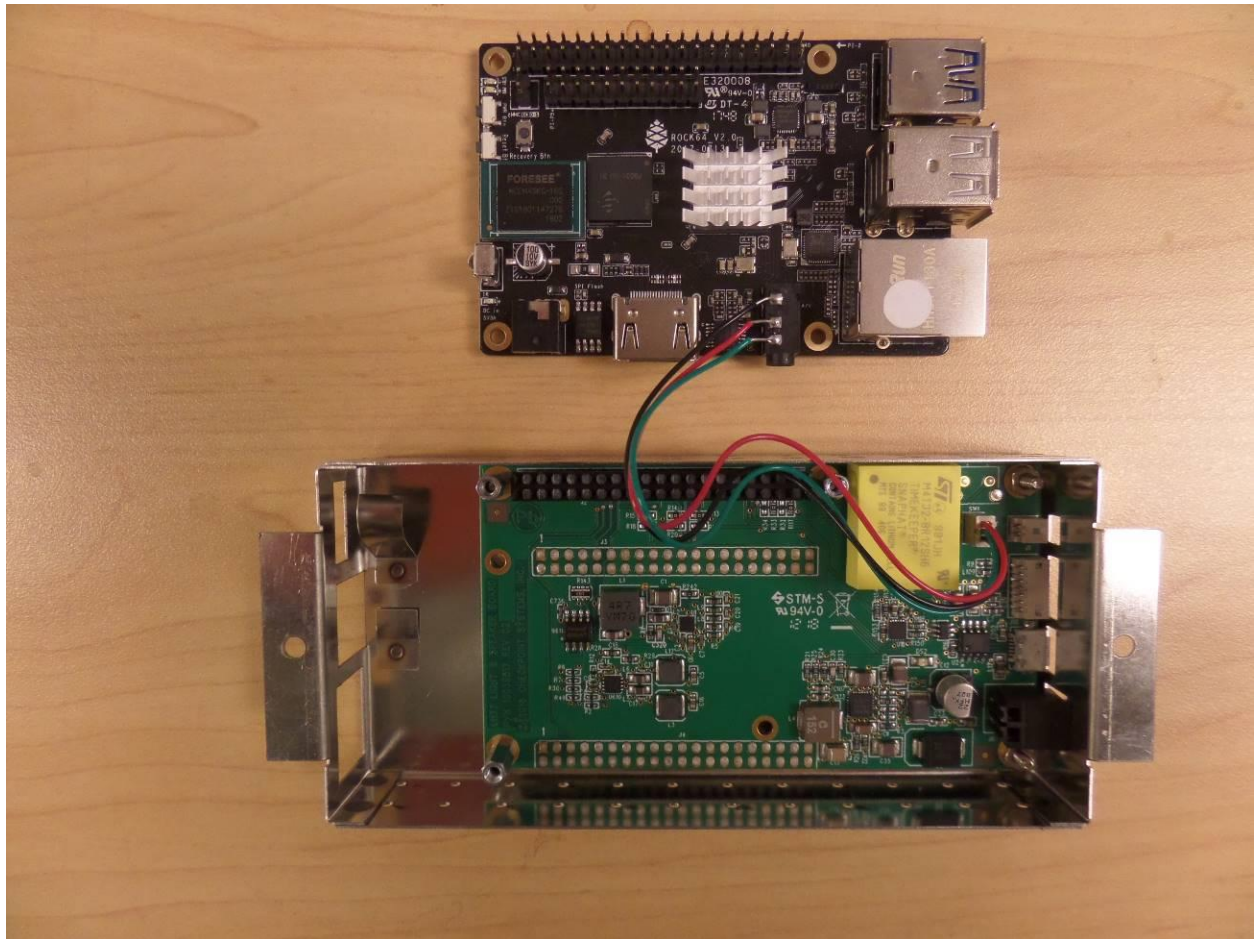
Photograph 3. A1177 lt&spkr Rock64 boards split view
