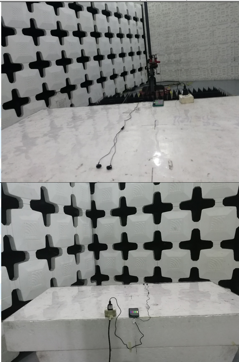
Radiated emission Test Setup (Above 1 GHz)
