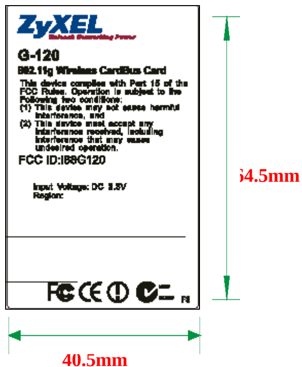
FCC ID Label Location
