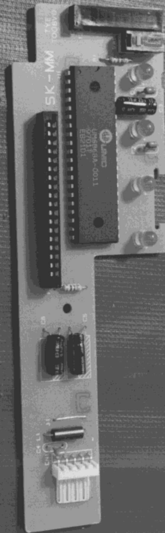
FCC ID: KU6SG-2000 PHOTO 4. EUT COMPONENT SIDE VIEW
