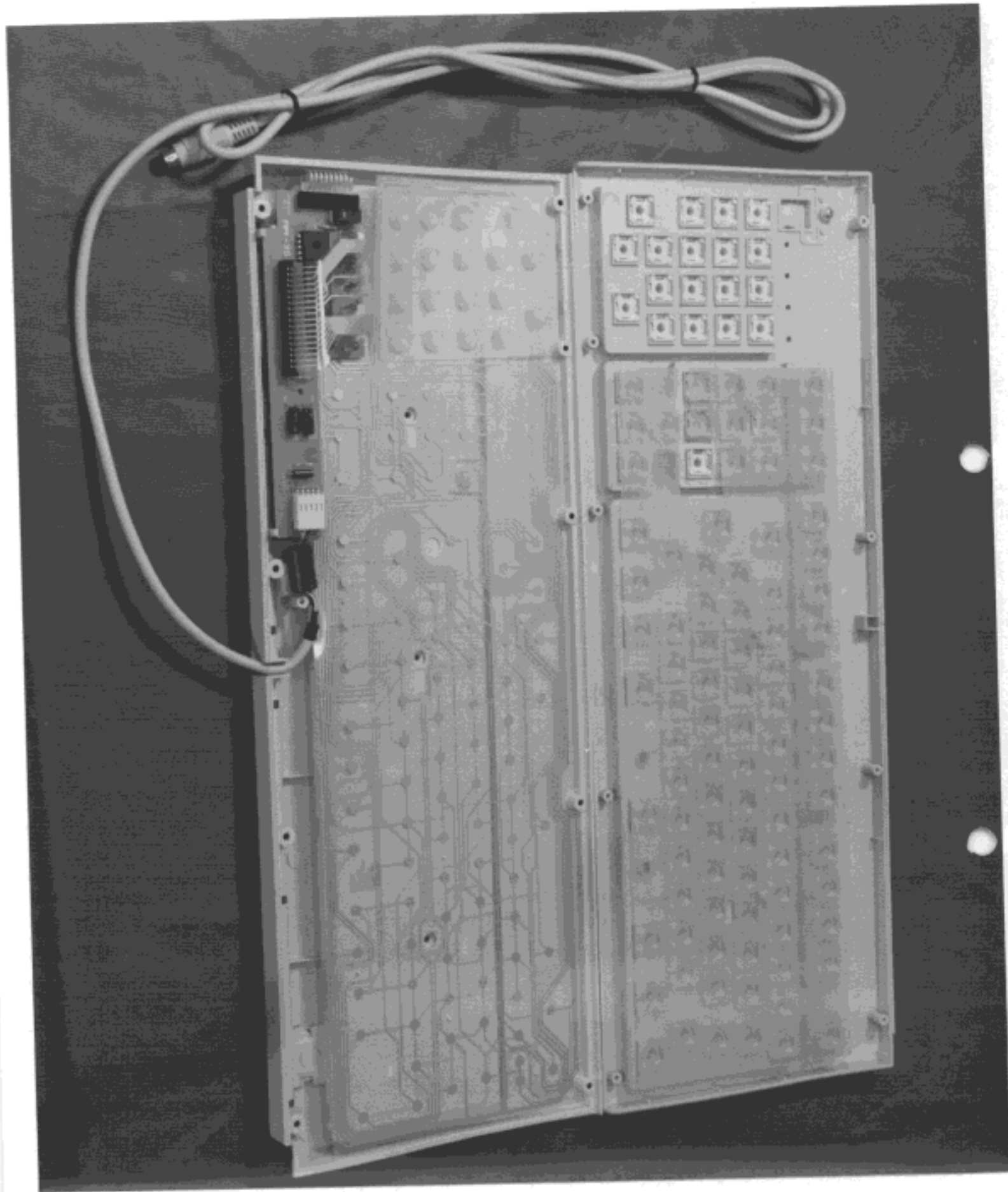
FCC ID: KU6SG-2000 PHOTO 3. EUT INSIDE VIEW
