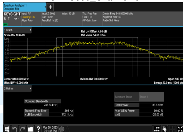
EGPRS850 Channel251
