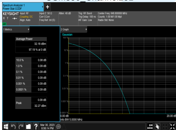
GPRS850 Channel251
