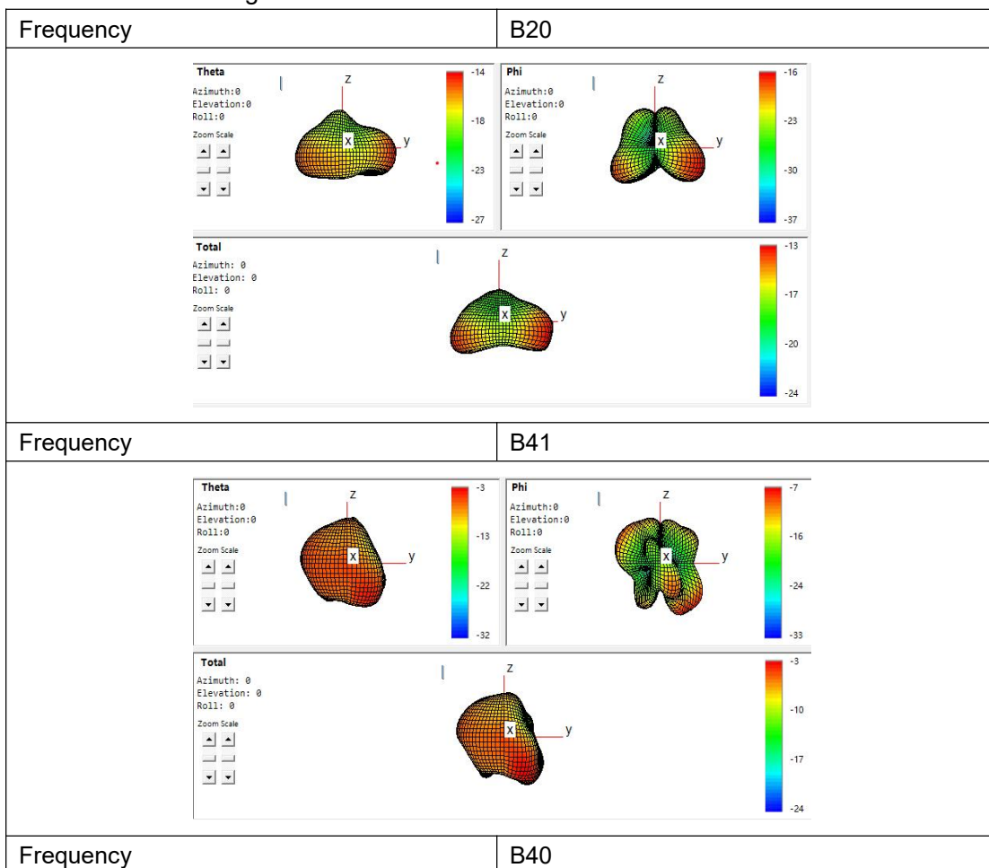
ANT2 directional diagram
