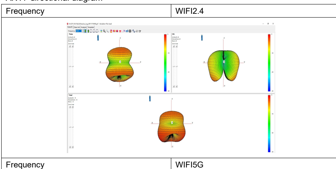
ANT7 directional diagram
