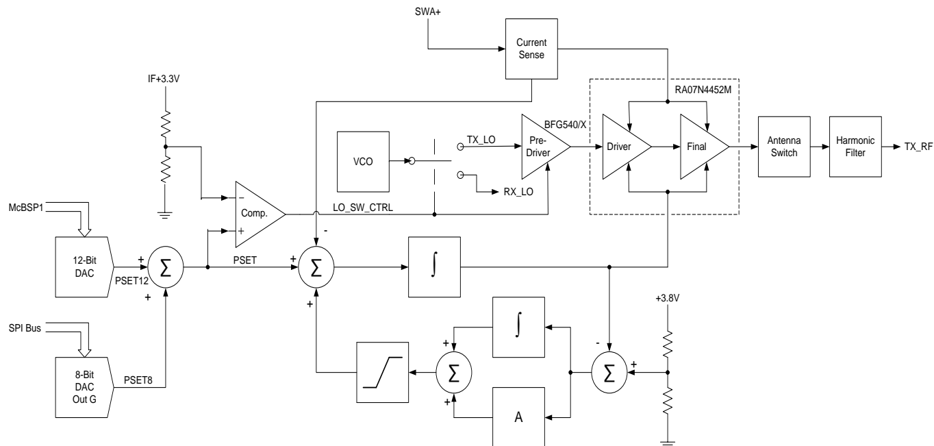
Figure 2 – Transmitter with Changes to Support Emissions Designator 8K10F1W
