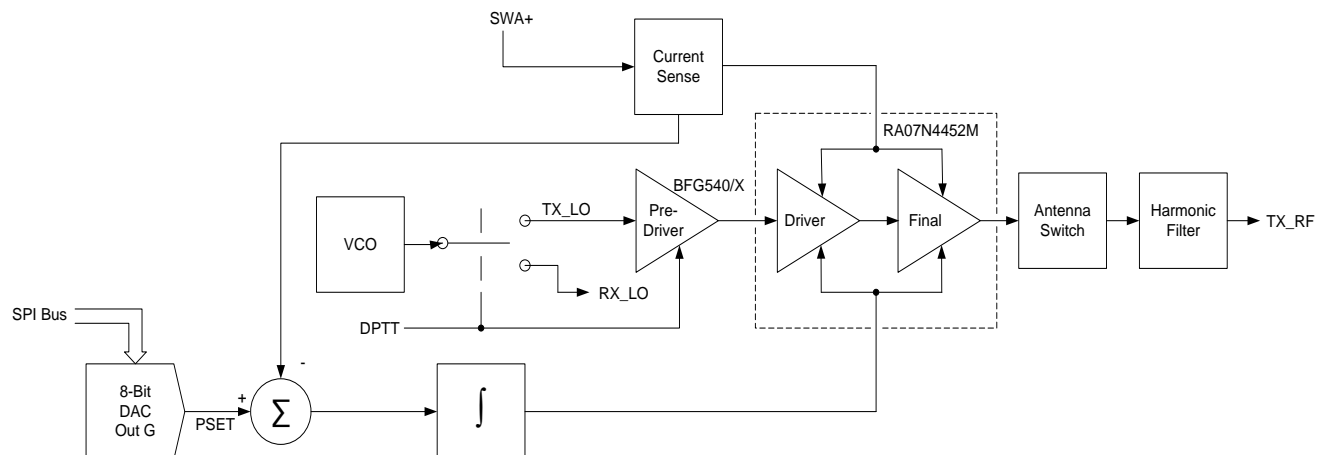
Figure 1 – Transmitter at Type Acceptance Grant
