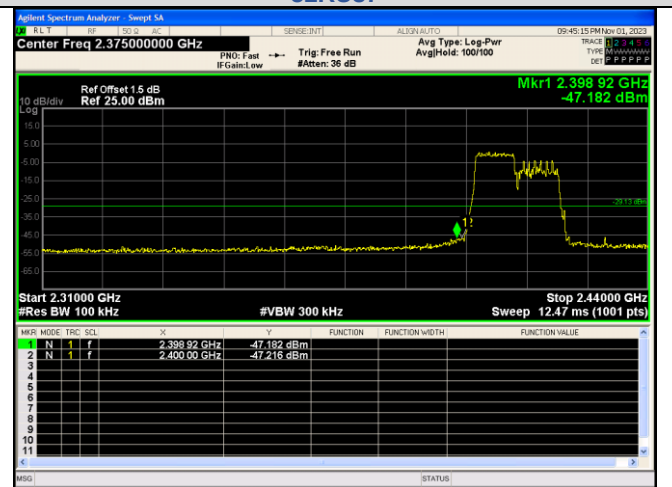
Out Of Band Emission IEEE 802.11ax_Channel 3_40MHz_Antenna 0_RU&Index 106RU53
