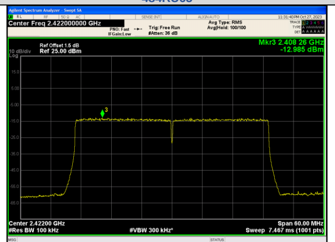
In-Band Reference Level IEEE 802.11ax_Channel 3_40MHz_Antenna 1_RU&Index 484RU65
