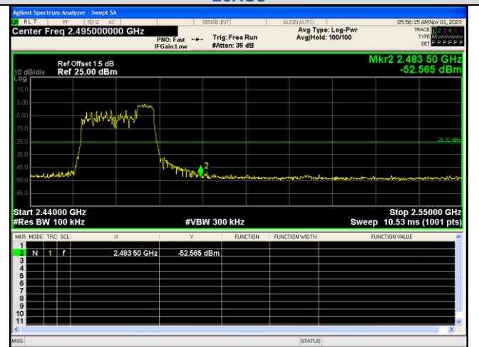
Out Of Band Emission IEEE 802.11ax_Channel 11_20MHz_Antenna 0_RU&Index 52RU40
