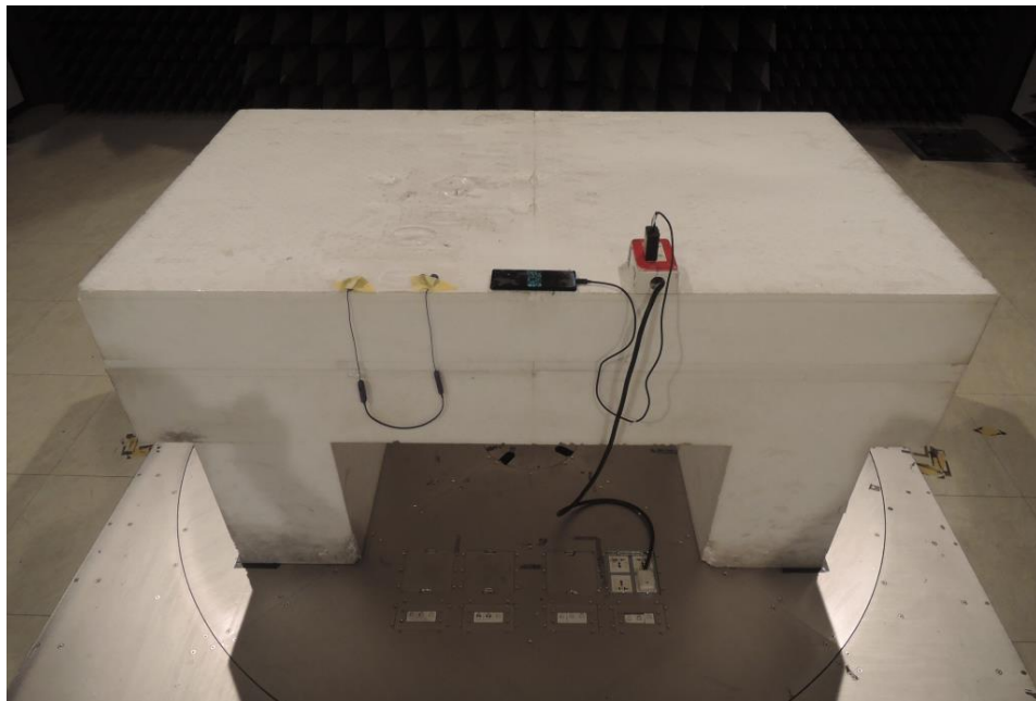
Rear View
