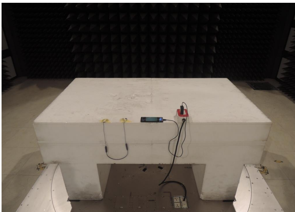
Rear View
