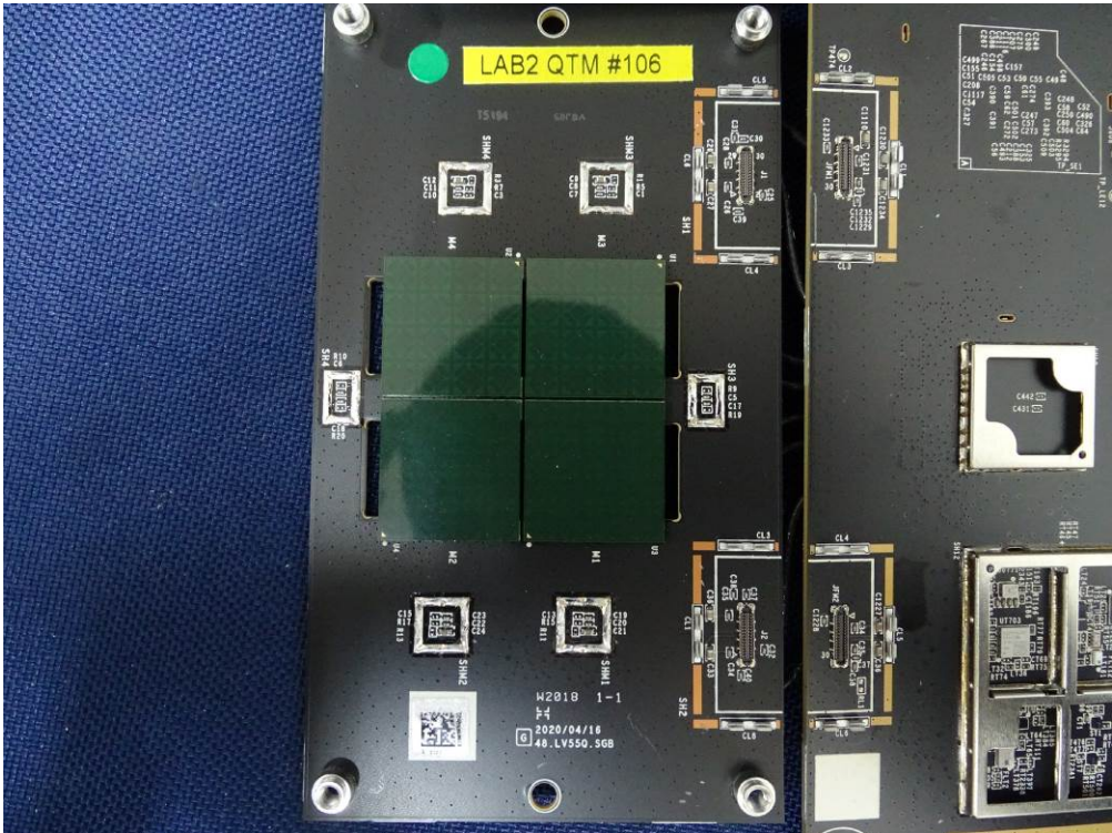
(89) EUT Photo
