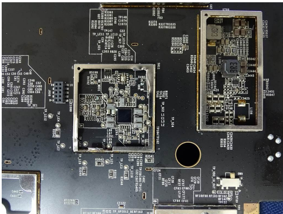
(79) EUT Photo
