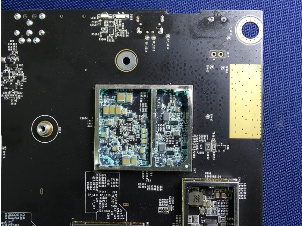
(73) EUT Photo
