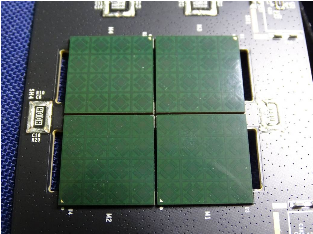
(90) EUT Photo
