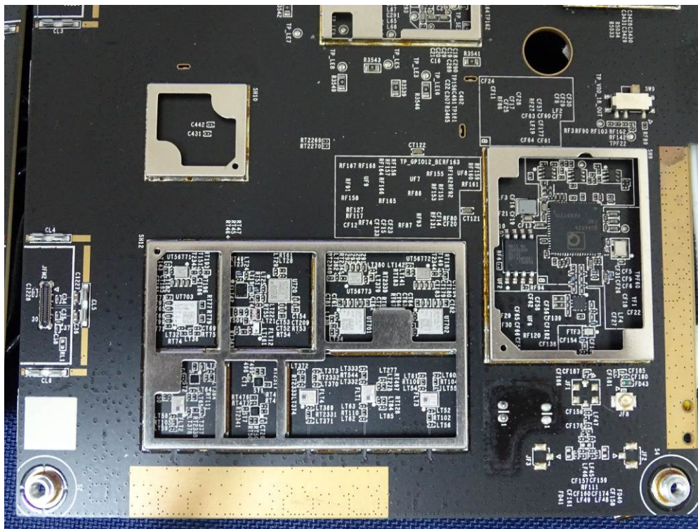
(80) EUT Photo
