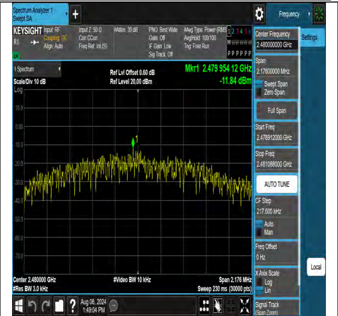
BLE_2M-Ant2-2480-PASS
