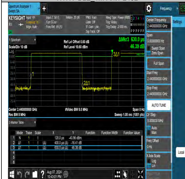
NTVN-BLE_1M-Ant1-2440
