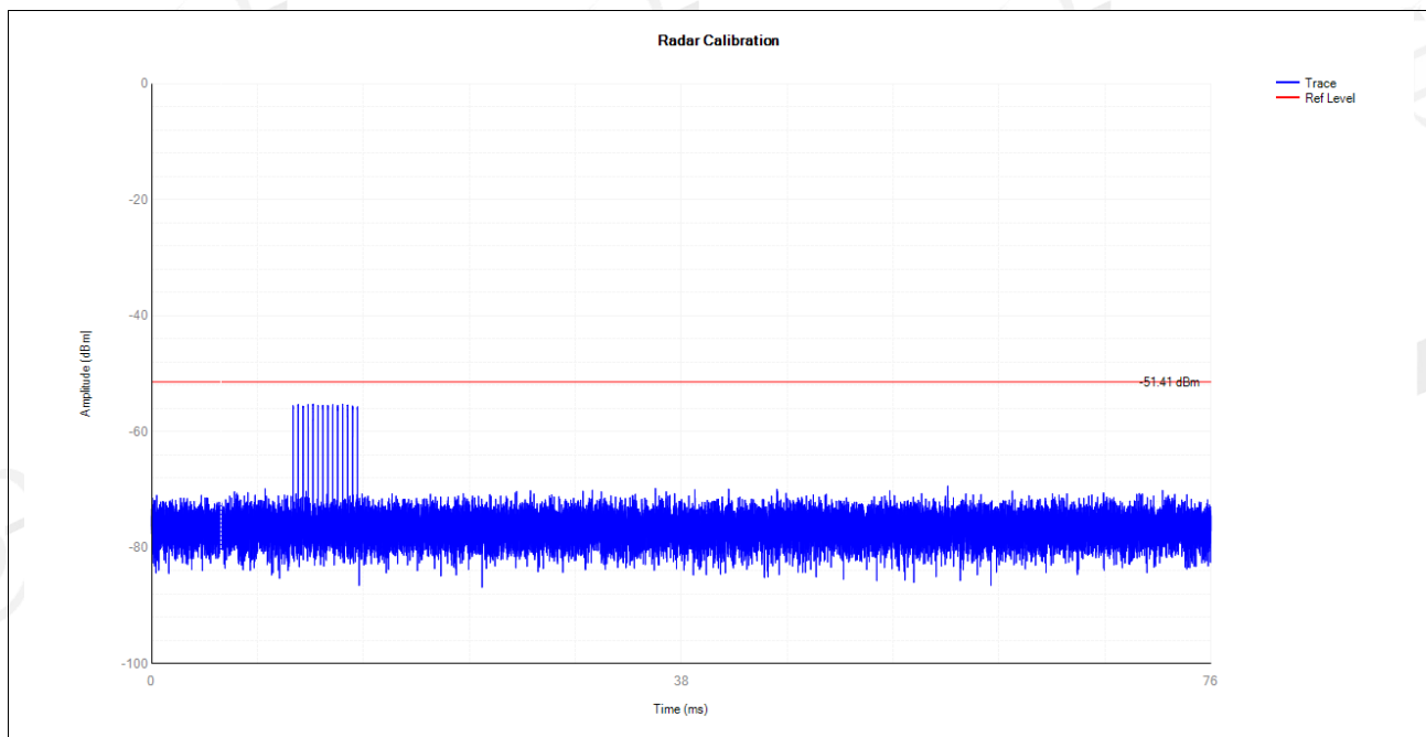
5310MHz DFS_FCC_T5000
