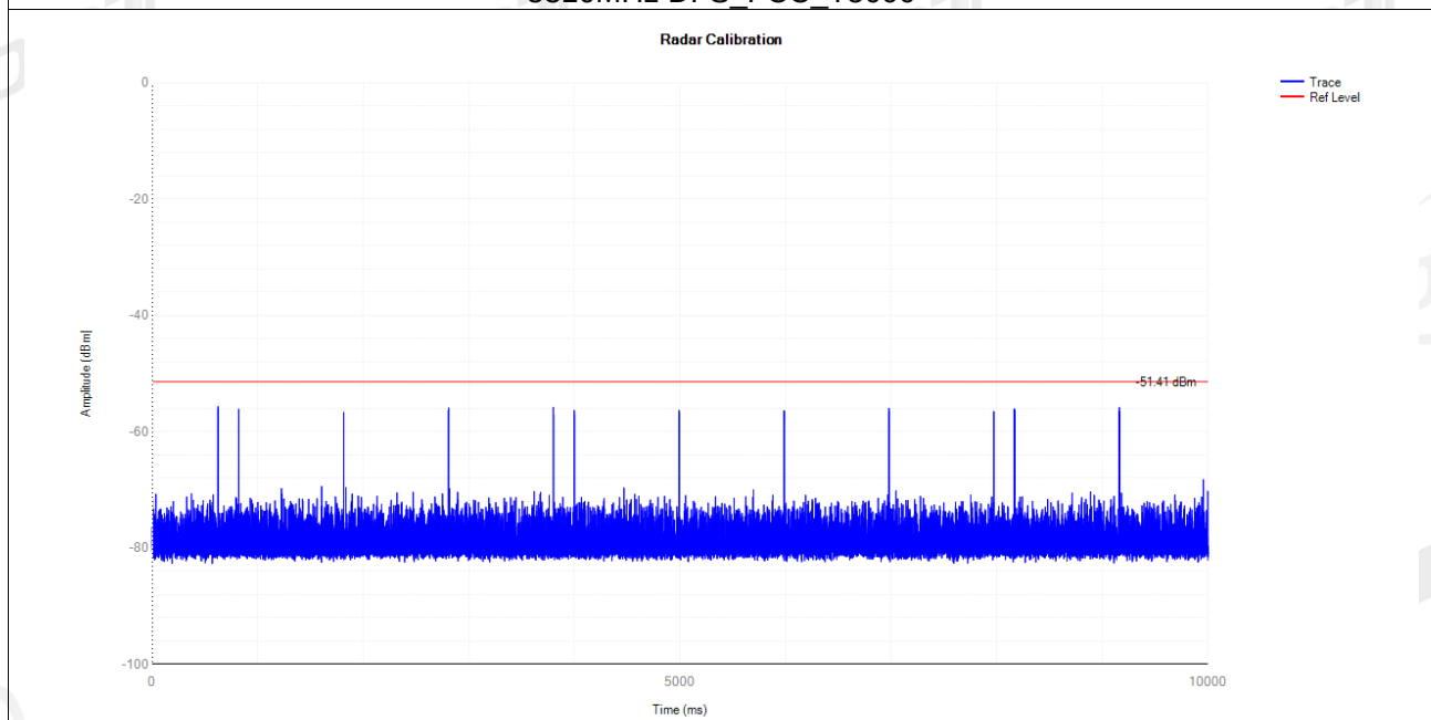
5310MHz DFS_FCC_T6000
