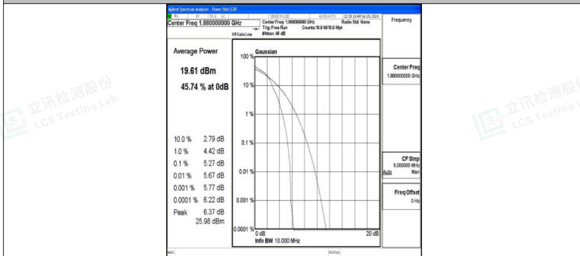
Band2-10MHz-16QAM-18900-1RB#0-PASS
