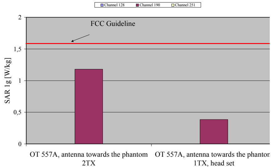
Fig. 10: The measured SAR values in body-worn configuration for the Alcatel One Touch 557A for GSM 850 (1 TX and 2 TX slots, gap = 20 mm) in comparison to the FCC exposure limit.
