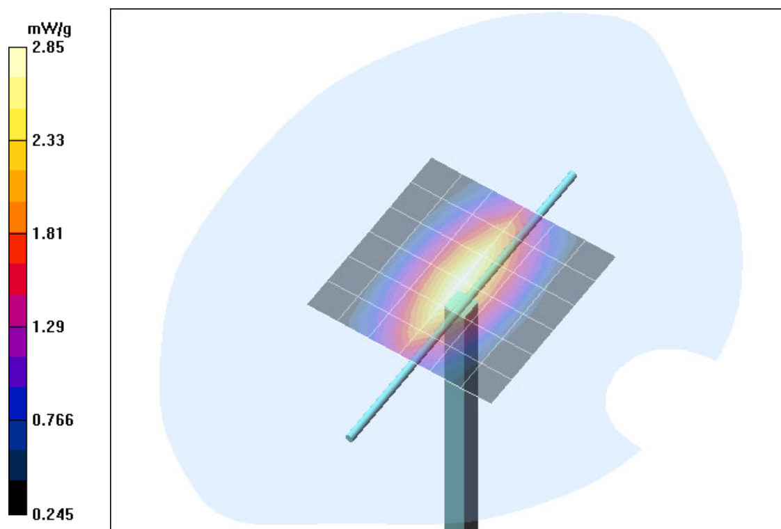
Fig. 13: Validation measurement 835 MHz body (July 15, 2004), coarse grid. Ambient Temperature: 21.5° C, Liquid Temperature: 20.5° C.
