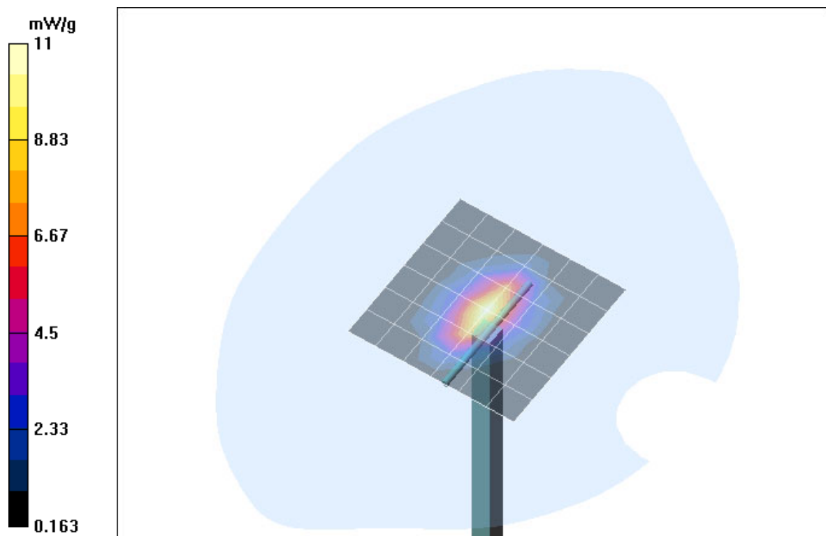
Fig. 14: Validation measurement 1900 MHz Head (July 06, 2004), coarse grid. Ambient Temperature: 20.8° C, Liquid Temperature: 20.3 C.
