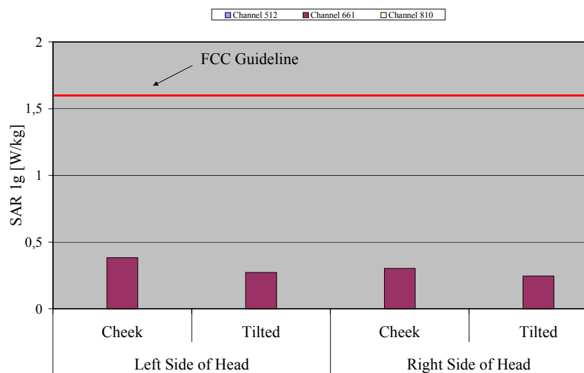
Fig. 9: The measured head phantom SAR values for the Alcatel One Touch 557A for PCS 1900 in comparison to the FCC exposure limit.
