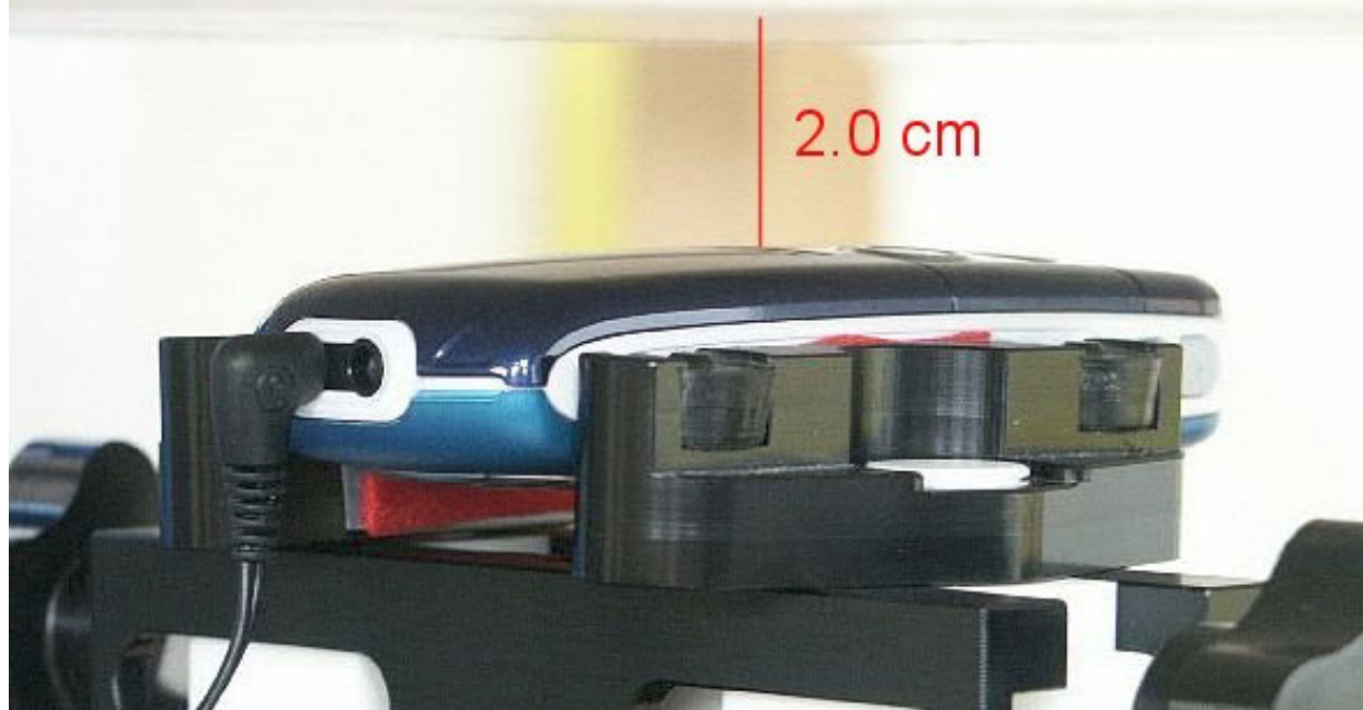
Fig. 25: Body worn configuration, GSM mode (1 TX slot) with headset, antenna towards the phantom.
