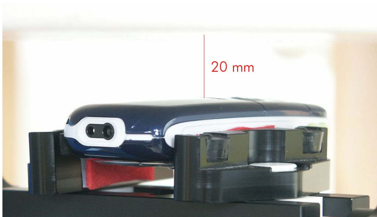
Fig. 24: Body worn configuration, GPRS mode (2 TX slots), antenna towards the phantom.
