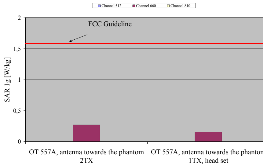
Fig. 11: The measured SAR values in body-worn configuration for the Alcatel One Touch 557A for PCS 1900 (1 TX and 2 TX slots, gap = 20 mm) in comparison to the FCC exposure limit.
