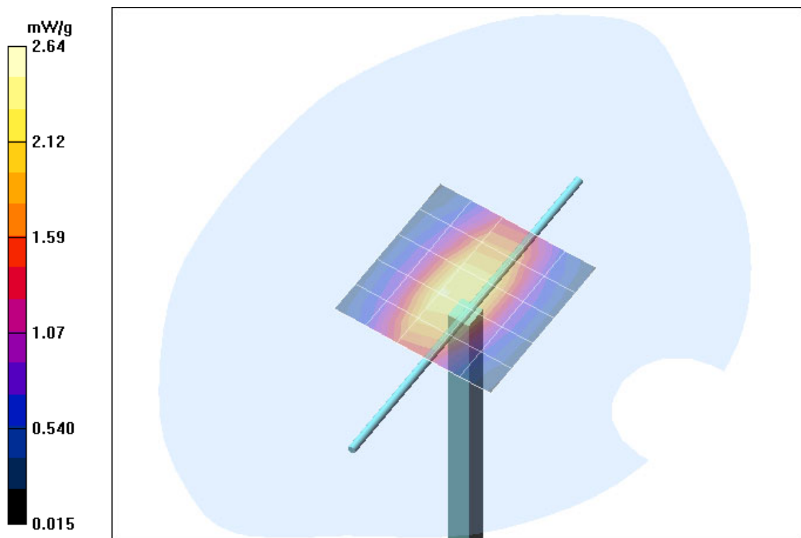
Fig. 12: Validation measurement 835 MHz Head (July 05, 2004), coarse grid. Ambient Temperature: 21.1° C, Liquid Temperature: 20.5 C.
