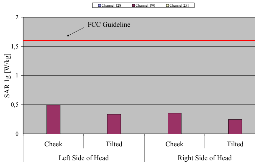
Fig. 8: The measured head phantom SAR values for the Alcatel One Touch 557A for GSM 850 in comparison to the FCC exposure limit.
