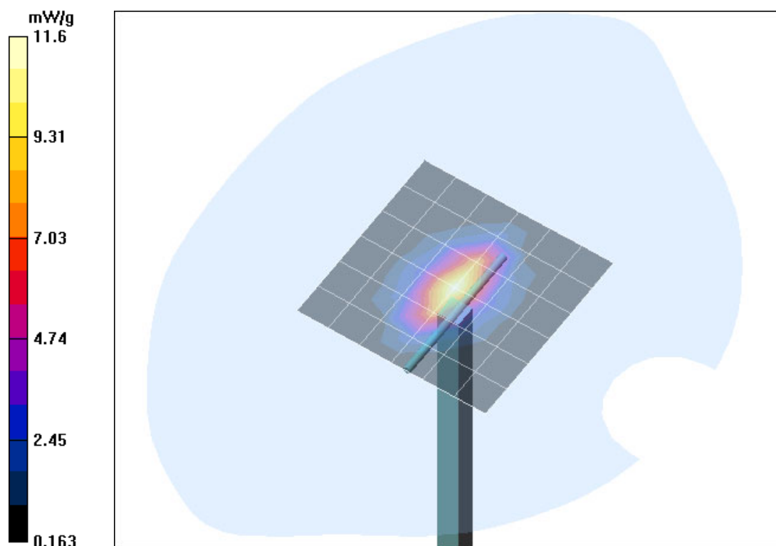
Fig. 15: Validation measurement 1900 MHz body (July 08, 2004), coarse grid. Ambient Temperature: 21.5° C, Liquid Temperature: 20.5° C.
