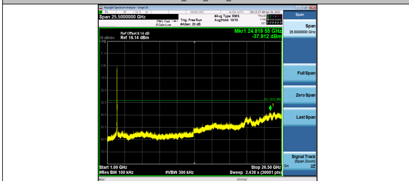
11N40SISO_Ant1_2437_0-Reference
