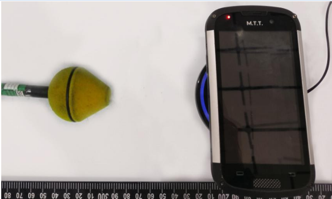
H-field Test Setup Photo
