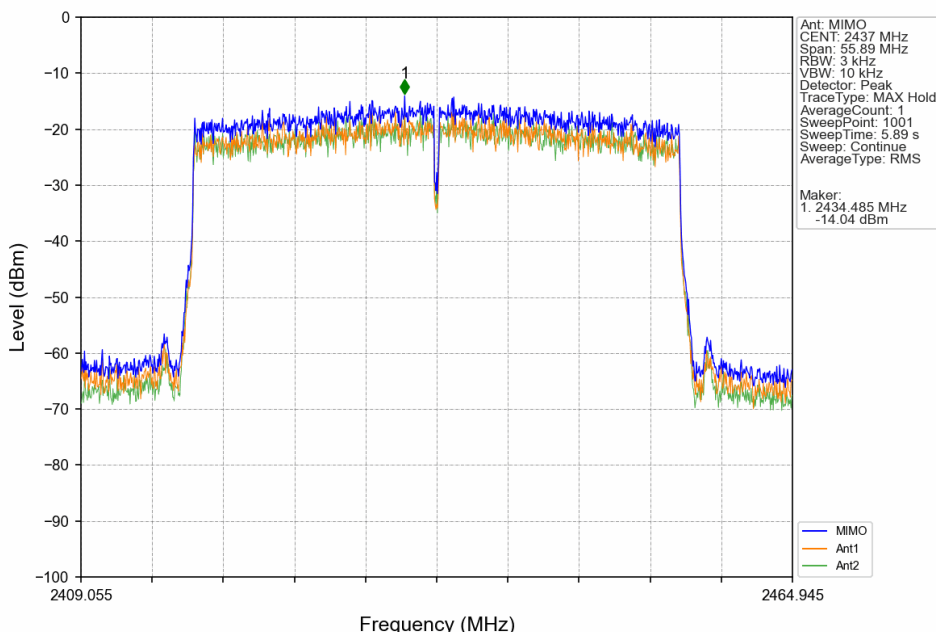
802.11ax(HEW40)_MCH_2437MHz_RU484_Left_MIMO_NTNV
