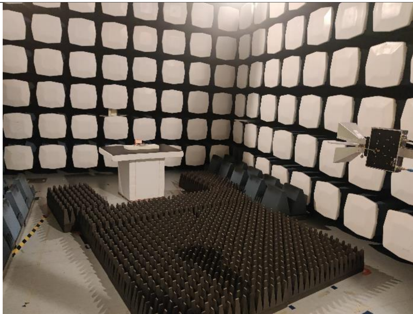
Picture 9, Radiated Emissions, common setup, 1 – 18 GHz
