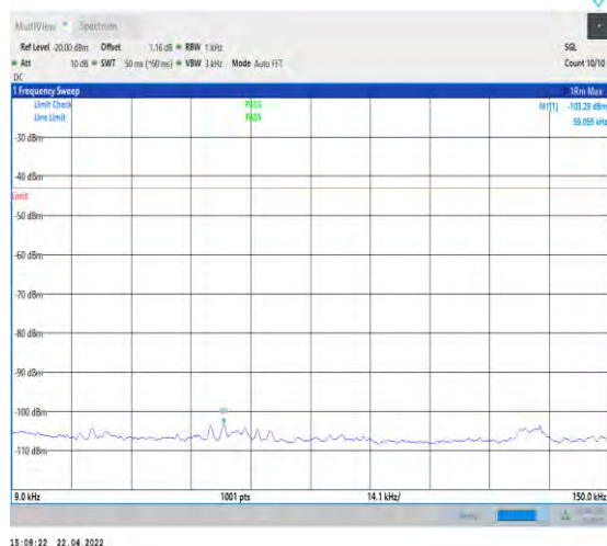
1-N25--15-40-H-1-DFT-PI2BPSK-Inner_1RB_Left-1 @1-0.009-0.15-Ant0--103.29--43-PASS
