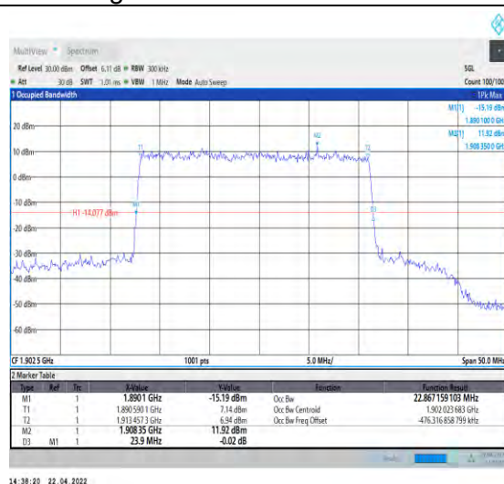
1-N25--15-25-H-4-DFT-64QAM-Outer_Full-128@0-A nt0-22.867-23.900-<25-PASS
