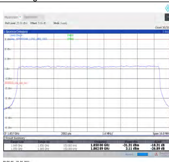
1-N25--15-15-L-3-DFT-PI2BPSK-Outer_Full-75@0 -Ant0-seegraph-PASS-see graph
