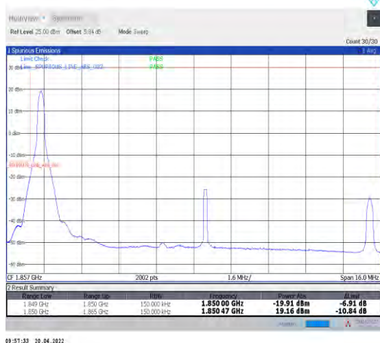
1-N25--15-15-L-4-CP-QPSK-Edge_1RB_Left-1@0-Ant 0-seegraph-PASS-see graph
