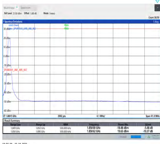
1-N25--15-40-L-4-CP-QPSK-Edge_1RB_Left-1@0-Ant0-seegraph-PASS-see graph
