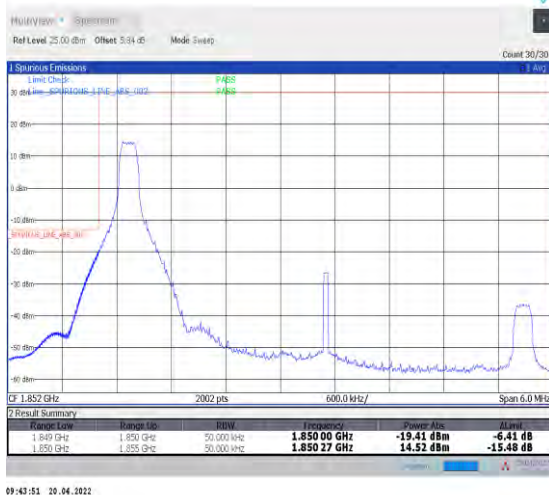
1-N25--15-5-L-4-CP-QPSK-Edge_1RB_Left-1@0-Ant0-seegraph-PASS-see graph
