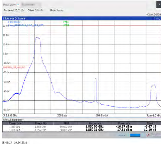
1-N25--15-5-L-1-DFT-PI2BPSK-Edge_1RB_Left-1@0-Ant0-seegraph-PASS-see graph
