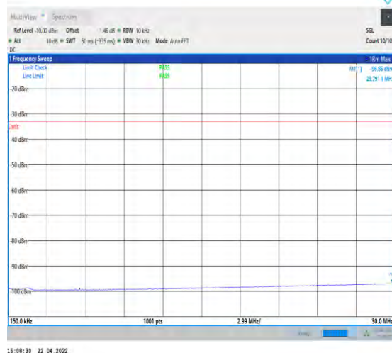
1-N25--15-40-H-1-DFT-PI2BPSK-Inner_1RB_Left-1 @1-0.15-30-Ant0--96.86--33-PASS
