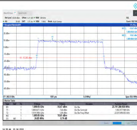
1-N25--15-25-H-6-CP-QPSK-Outer_Full-133@0-Ant 0-23.741-24.850-<25-PASS
