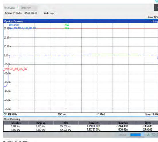
1-N25--15-40-L-6-CP-QPSK-Outer_Full-216@0-Ant0-seegraph-PASS-see graph
