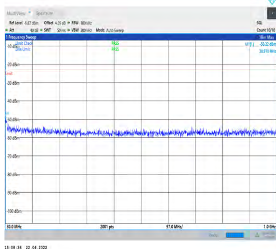
1-N25--15-40-H-1-DFT-PI2BPSK-Inner_1RB_Left-1 @1-30-1000-Ant0--50.22--23-PASS
