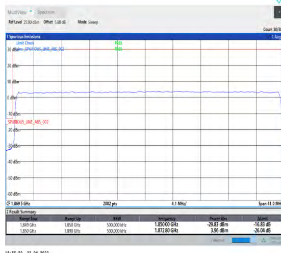
1-N25--15-40-L-3-DFT-PI2BPSK-Outer_Full-216@0-Ant0-seegraph-PASS-see graph
