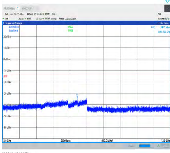
1-N25--15-40-M-1-DFT-PI2BPSK-Inner_1RB_Left-1 @1-3000-12000-Ant0--34.32--13-PASS
