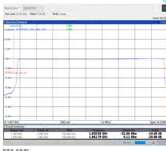
1-N25--15-15-L-6-CP-QPSK-Outer_Full-79@0-Ant 0-seegraph-PASS-see graph
