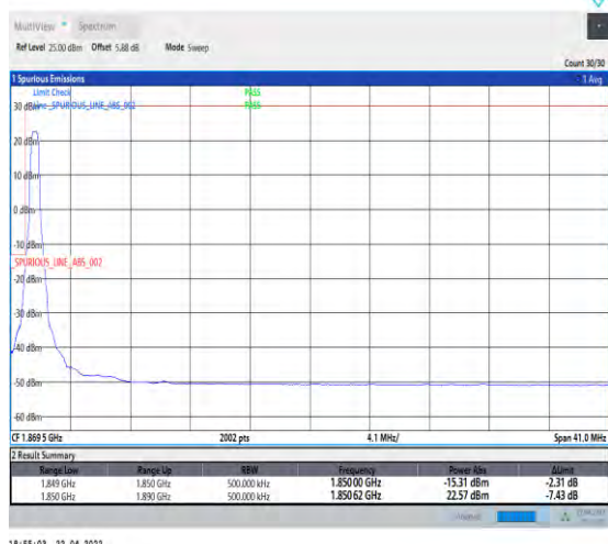
1-N25--15-40-L-1-DFT-PI2BPSK-Edge_1RB_Left-1@0-Ant0-seegraph-PASS-see graph
