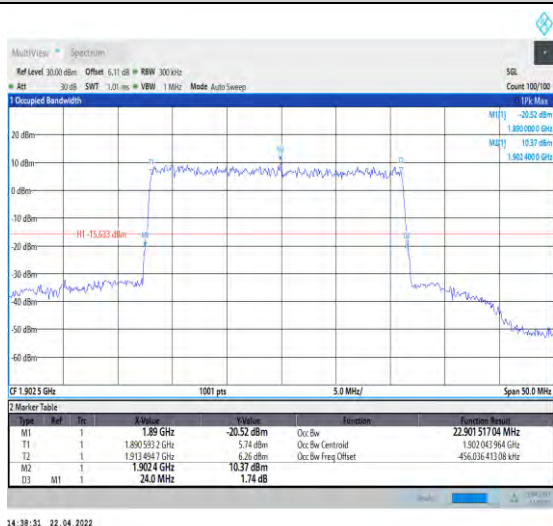
1-N25--15-25-H-5-DFT-256QAM-Outer_Full-128@0-A Ant0-22.902-24.000-<25-PASS
