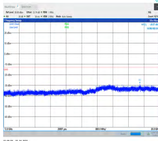
1-N25--15-40-H-1-DFT-PI2BPSK-Inner_1RB_Left-1 @1-12000-20000-Ant0--28.37--13-PASS
