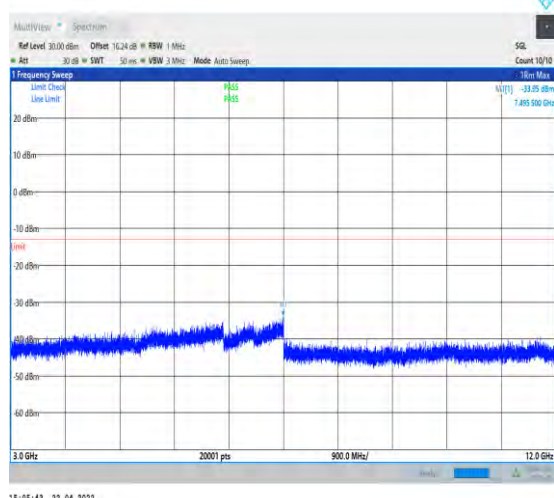
1-N25--15-40-L-1-DFT-PI2BPSK-Inner_1RB_Left-1 @1-3000-12000-Ant0--33.95--13-PASS
