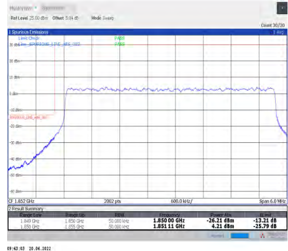
1-N25--15-5-L-3-DFT-PI2BPSK-Outer_Full-25@0-Ant0-seegraph-PASS-see graph
