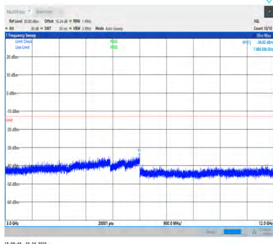
1-N25--15-40-H-1-DFT-PI2BPSK-Inner_1RB_Left-1 @1-3000-12000-Ant0--34.82--13-PASS
