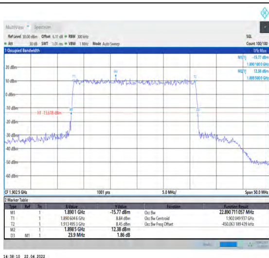
1-N25--15-25-H-3-DFT-16QAM-Outer_Full-128@0-A nt0-22.891-23.900-<25-PASS
