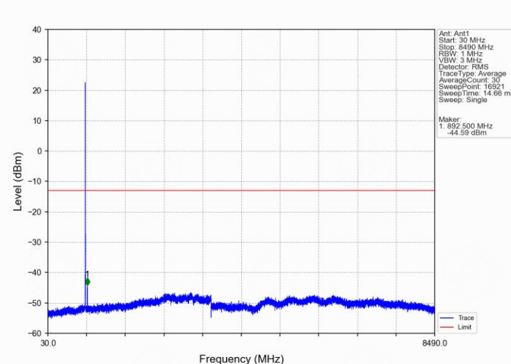
Band5 3MHz QPSK HCH 847.5MHz RB 1 0 NTN
