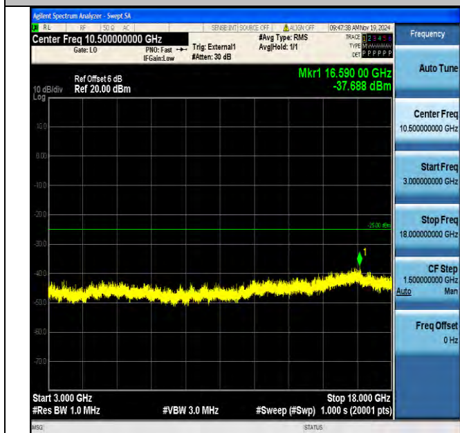
Band38_15MHz_16QAM_38000_1RB#0_3000~18000_3000~18000
