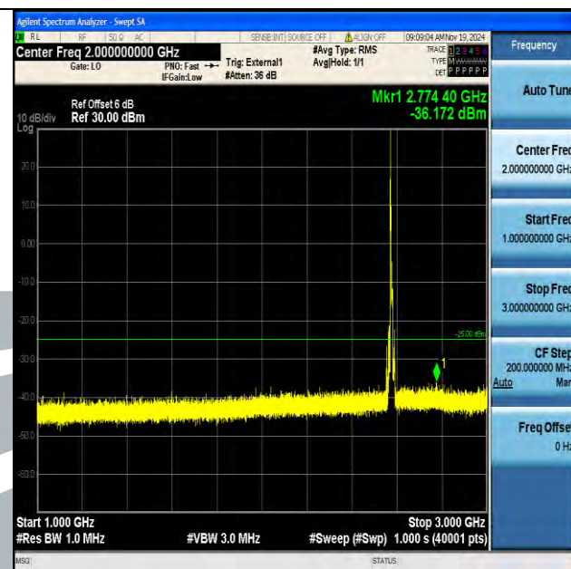
Band38_10MHz_16QAM_37800_1RB#0_1000~3000_1000~3000
