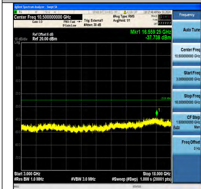
Band38_20MHz_16QAM_37850_1RB#0_3000~18000_3000~18000
