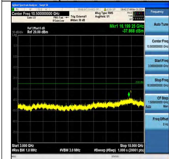
Band38_15MHz_QPSK_37825_1RB#0_3000~18000_3000~18000
