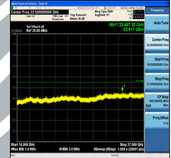
Band38_5MHz_QPSK_37775_1RB#0_18000~27000_18000~27000
