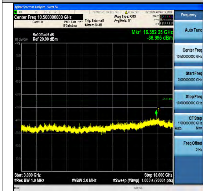
Band38_10MHz_16QAM_37800_1RB#0_3000~18000_3000~18000
