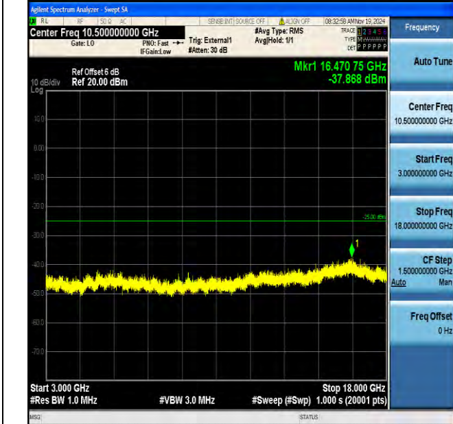
Band38_5MHz_QPSK_37775_1RB#0_3000~18000_3000~18000
