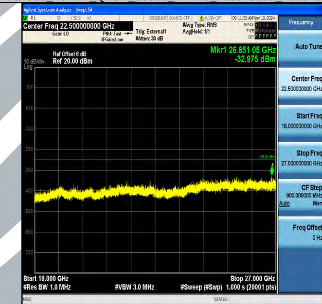
Band38_10MHz_QPSK_38000_1RB#0_18000~27000_18000~27000
