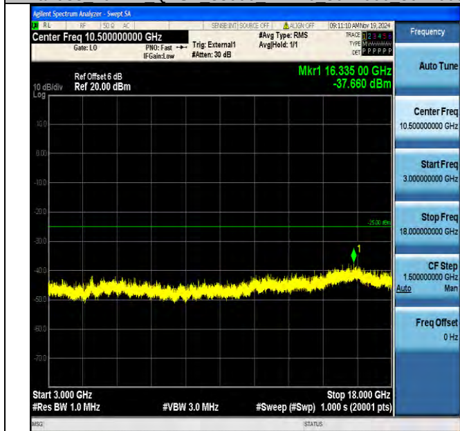
Band38_10MHz_QPSK_38000_1RB#0_3000~18000_3000~18000
