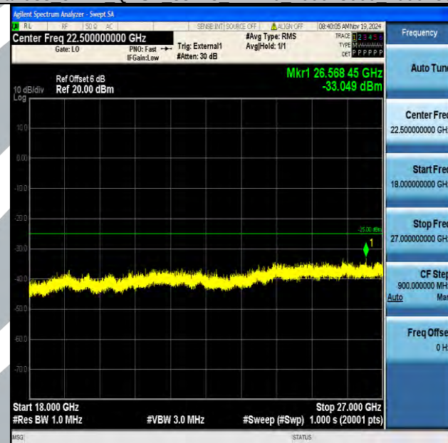
Band38_5MHz_QPSK_38225_1RB#0_18000~27000_18000~27000
