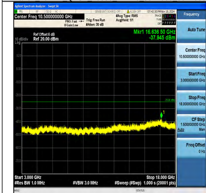
Band7_20MHz_QPSK_20850_1RB#0_3000~18000_3000~18000
