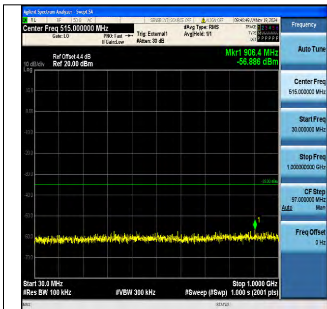
Band38_15MHz_16QAM_38000_1RB#0_30~1000_30~1000
