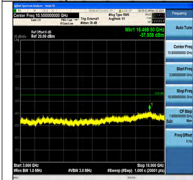
Band38_5MHz_QPSK_38225_1RB#0_3000~18000_3000~18000
