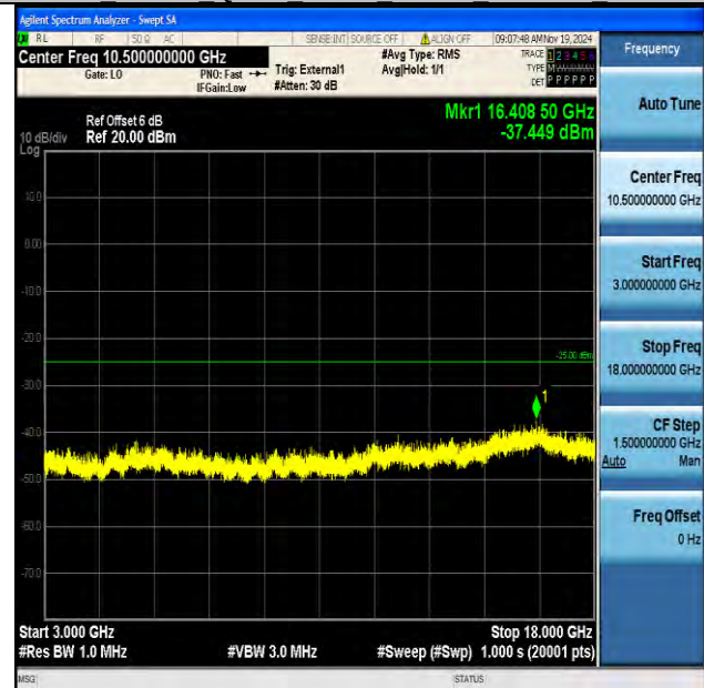
Band38_10MHz_QPSK_37800_1RB#0_3000~18000_3000~18000
