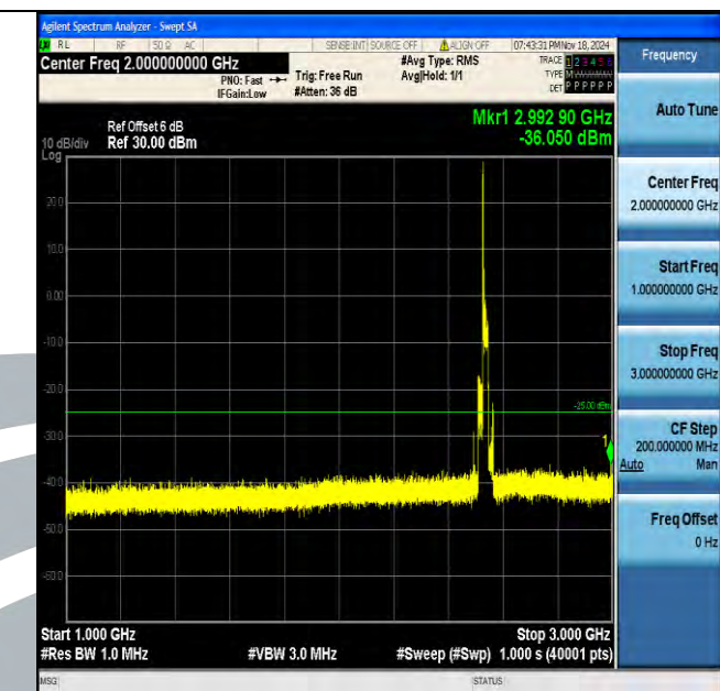
Band7_20MHz_QPSK_21100_1RB#0_1000~3000_1000~3000
