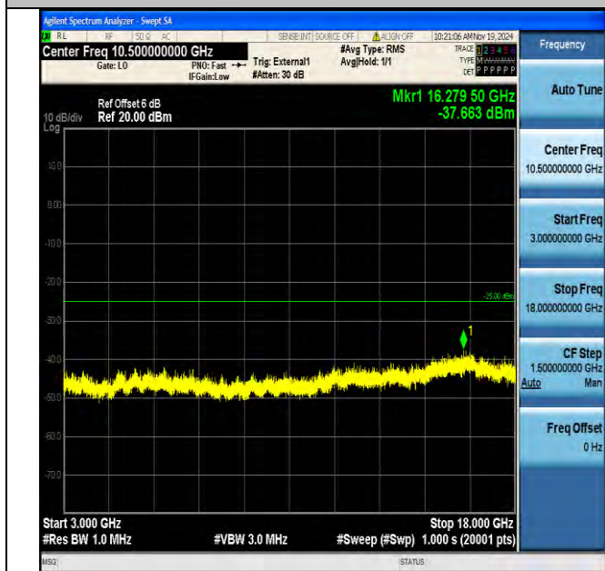
Band38_20MHz_16QAM_38000_1RB#0_3000~18000_3000~18000
