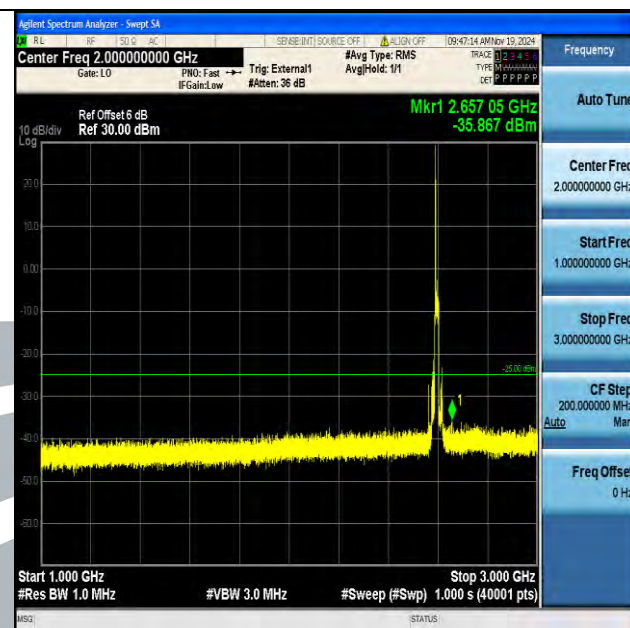
Band38_15MHz_16QAM_38000_1RB#0_1000~3000_1000~3000
