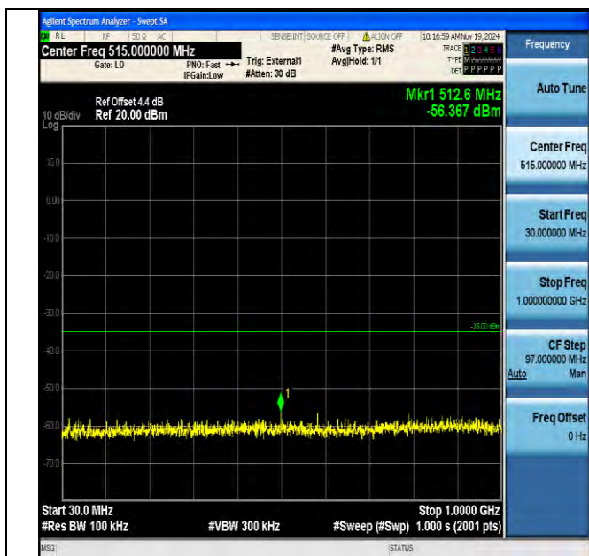
Band38_20MHz_16QAM_37850_1RB#0_30~1000_30~1000
