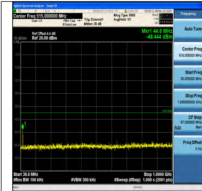
Band38_15MHz_16QAM_38175_1RB#0_30~1000_30~1000
