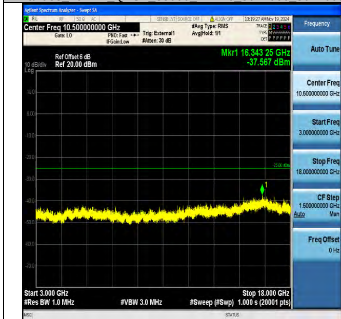
Band38_20MHz_QPSK_38000_1RB#0_3000~18000_3000~18000
