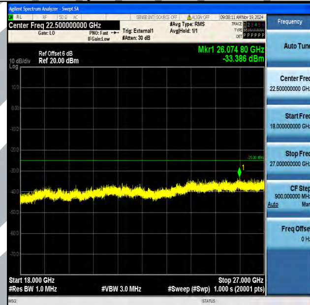
Band38_10MHz_QPSK_37800_1RB#0_18000~27000_18000~27000
