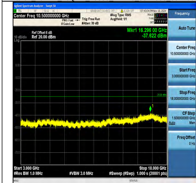
Band7_20MHz_16QAM_20850_1RB#0_3000~18000_3000~18000
