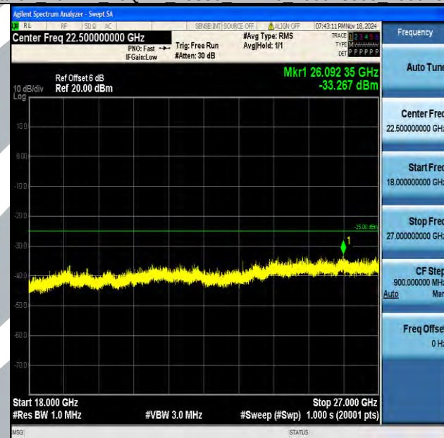
Band7_20MHz_16QAM_20850_1RB#0_18000~27000_18000~27000
