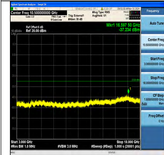
Band38_15MHz_16QAM_38175_1RB#0_3000~18000_3000~18000
