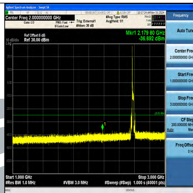
Band38_20MHz_16QAM_37850_1RB#0_1000~3000_1000~3000
