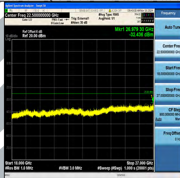
Band38_15MHz_QPSK_37825_1RB#0_18000~27000_18000~27000
