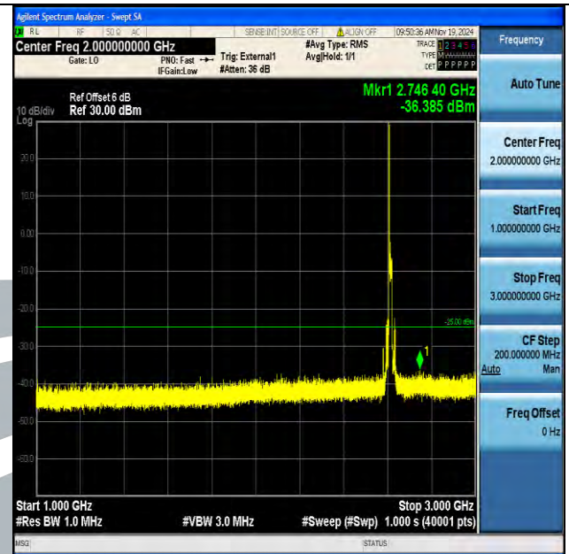
Band38_15MHz_16QAM_38175_1RB#0_1000~3000_1000~3000
