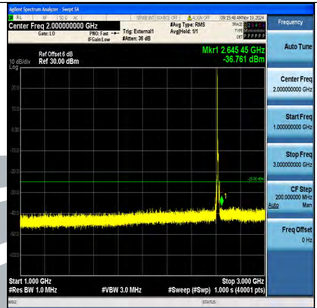
Band38_10MHz_16QAM_38200_1RB#0_1000~3000_1000~3000
