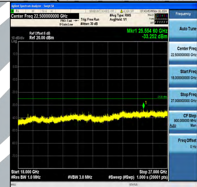
Band7_20MHz_QPSK_21100_1RB#0_18000~27000_18000~27000
