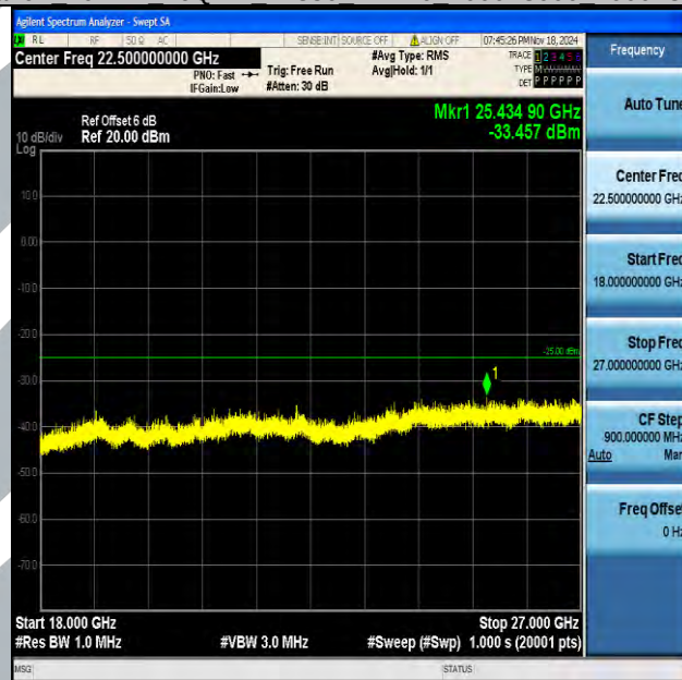
Band7_20MHz_16QAM_21350_1RB#0_18000~27000_18000~27000
