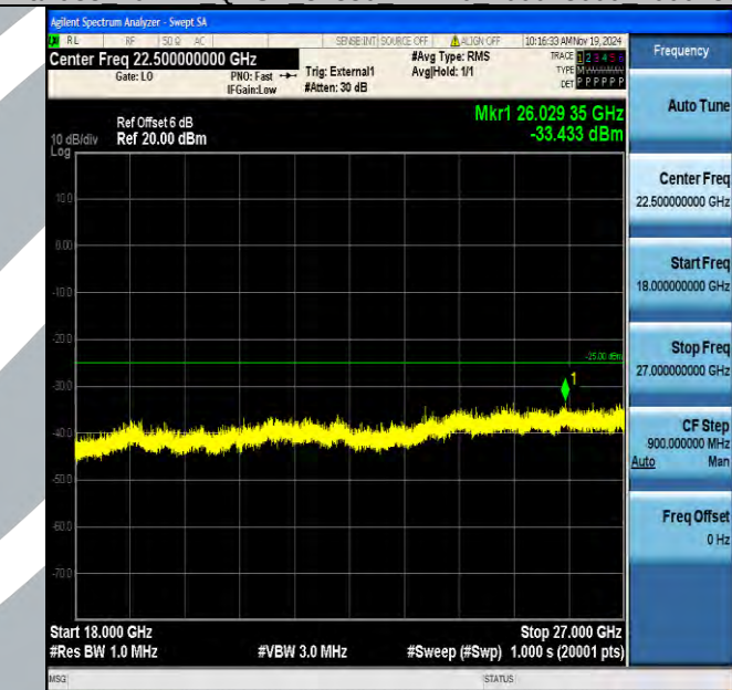
Band38_20MHz_QPSK_37850_1RB#0_18000~27000_18000~27000
