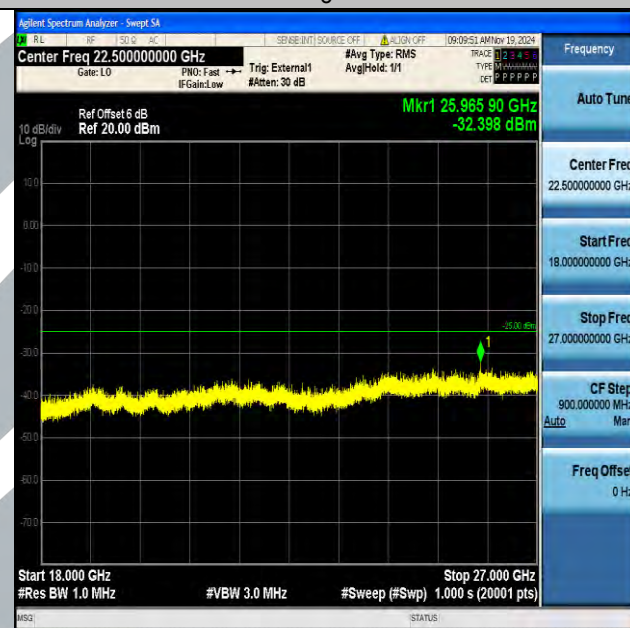
Band38_10MHz_16QAM_37800_1RB#0_18000~27000_18000~27000
