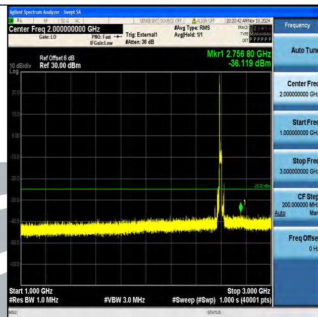
Band38_20MHz_16QAM_38000_1RB#0_1000~3000_1000~3000
