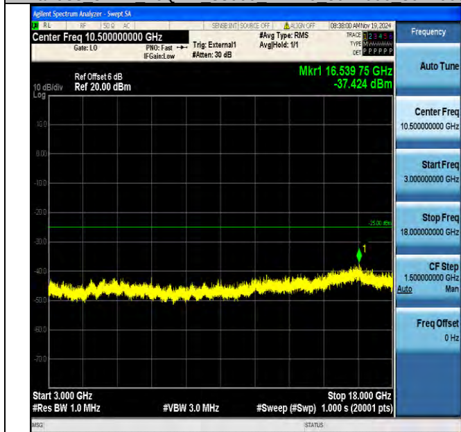
Band38_5MHz_16QAM_38000_1RB#0_3000~18000_3000~18000
