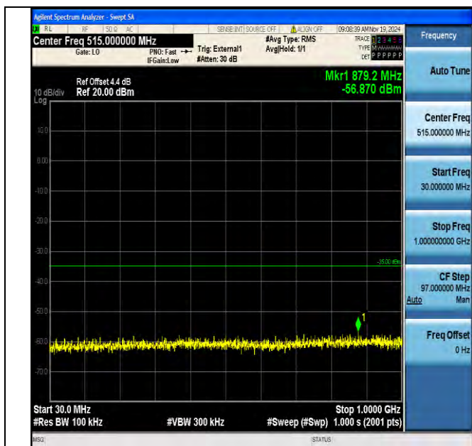
Band38_10MHz_16QAM_37800_1RB#0_30~1000_30~1000
