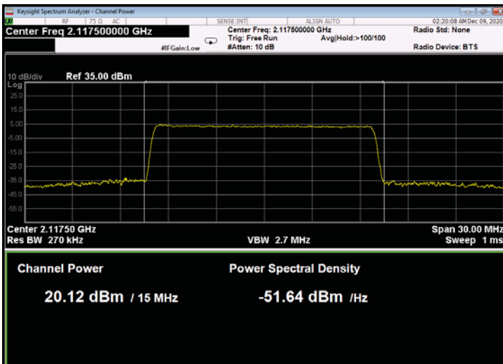
Figure 223: QPSK 15MHz B.W.; 2117.5MHz, 30kHz
