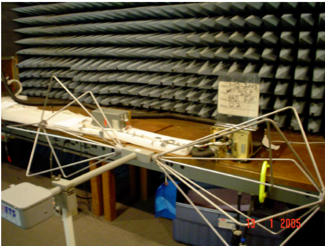
Figure G-5. Radiated Emission 25 MHz – 200 MHz
