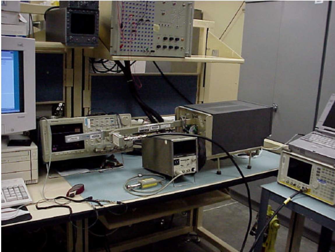
Figure G-1. Bench Test Setup - Occupied Bandwidth, Antenna Spurious, Power Line Stability
