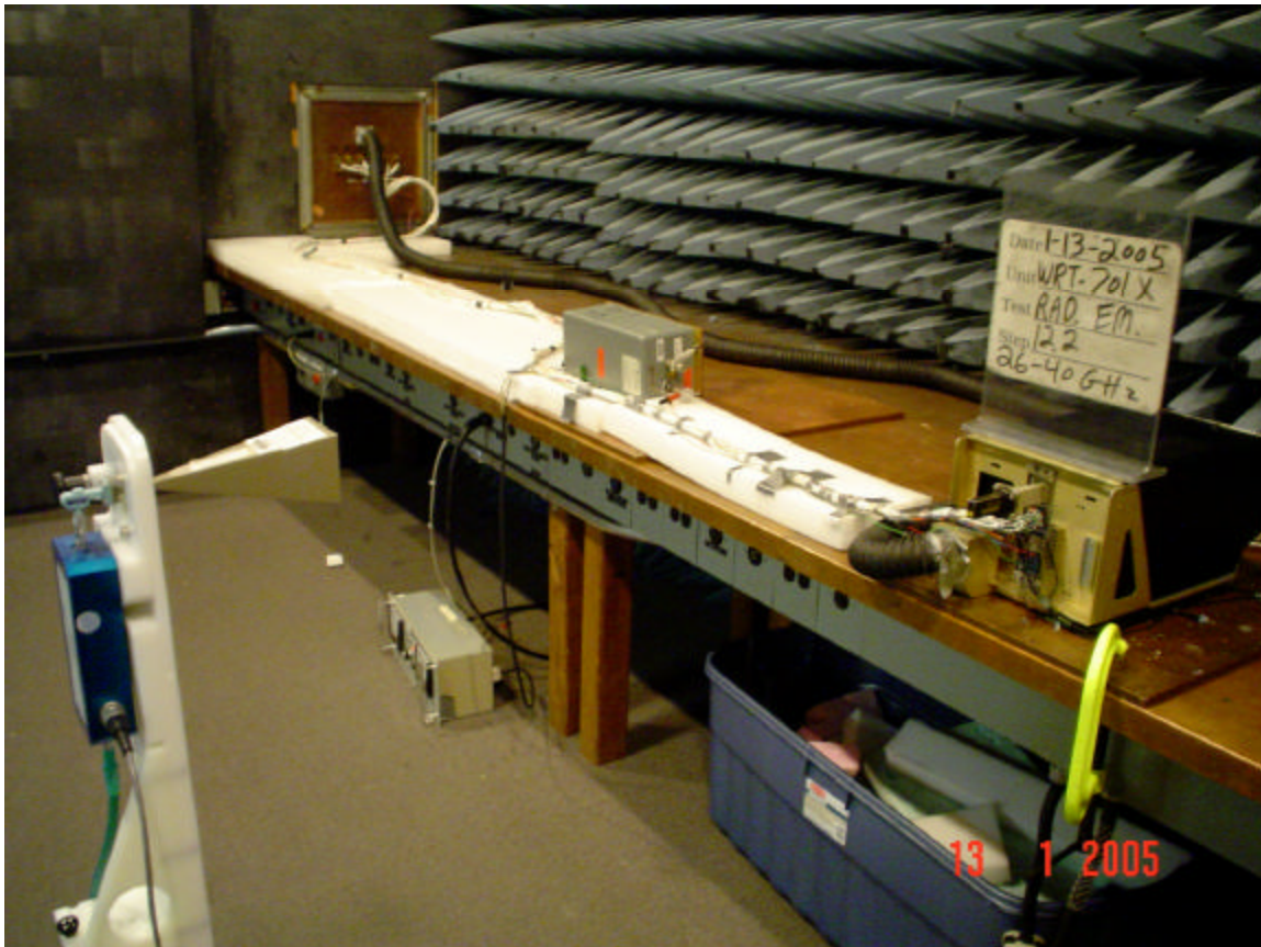
Figure G-9. Radiated Emission 26 GHz – 40 GHz
