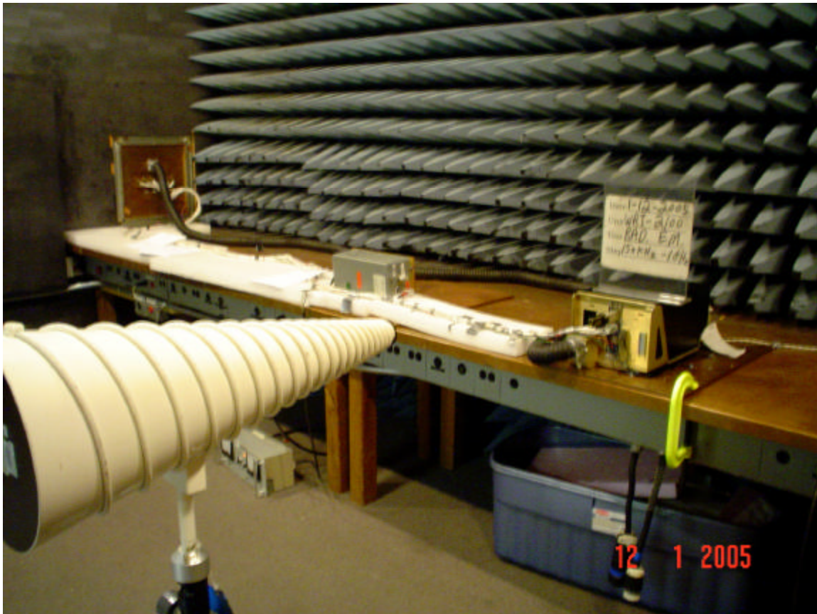
Figure G-6. Radiated Emission 200 MHz – 1 GHz
