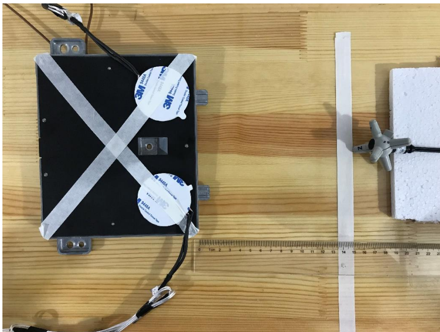
E-field Test Setup Photo Positon A Load2&3 (15cm)
