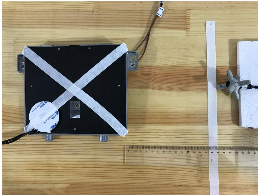
E-field Test Setup Photo Positon B Load1 (15cm)
