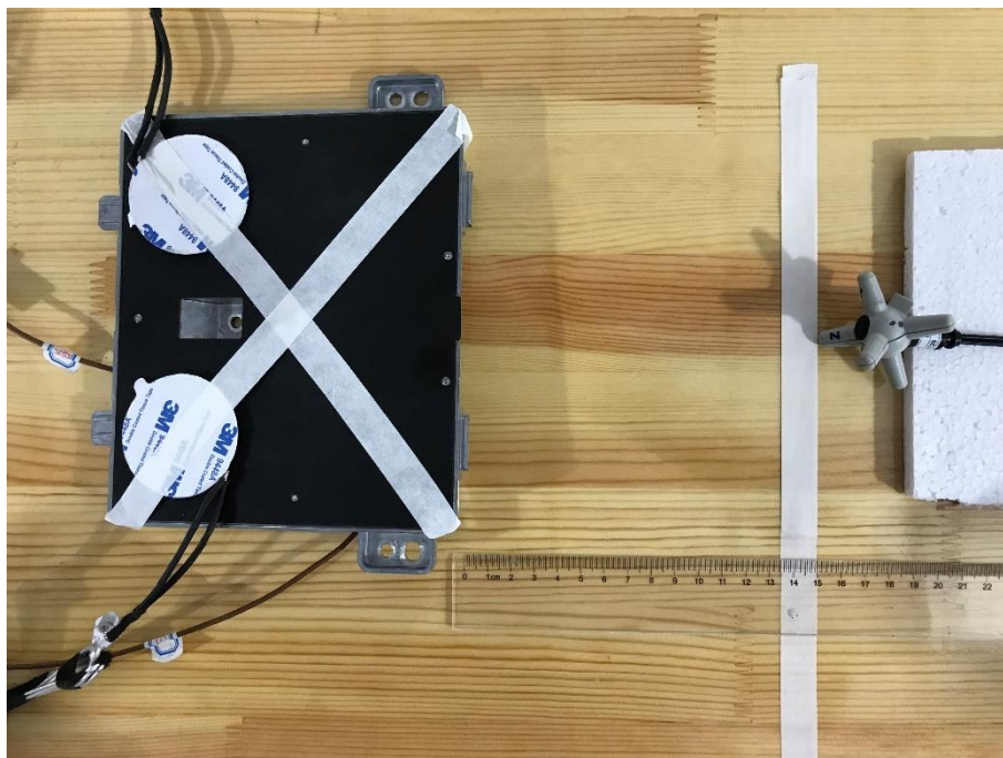
E-field Test Setup Photo Positon C Load2&amp;3 (15cm)
