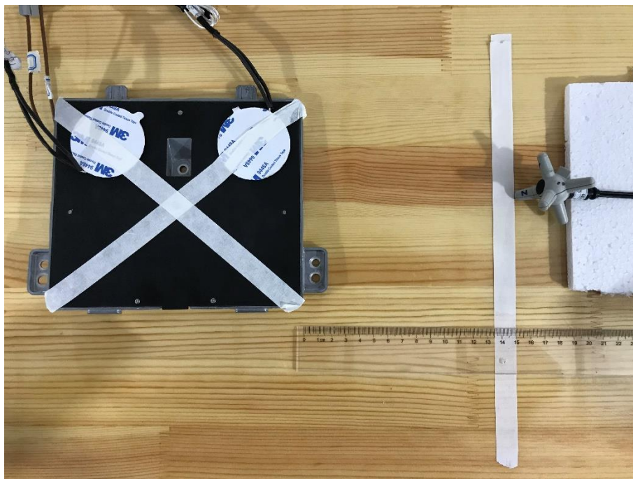
E-field Test Setup Photo Positon D Load2&amp;3 (15cm)
