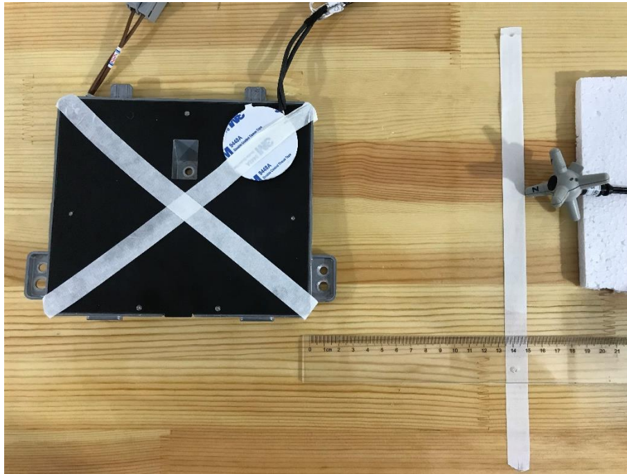
E-field Test Setup Photo Positon D Load1 (15cm)
