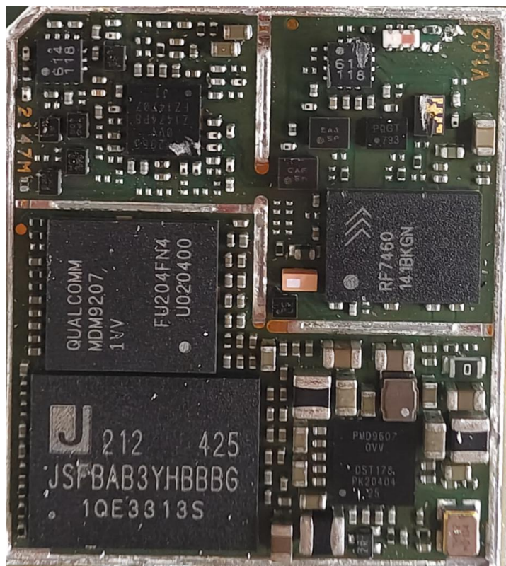
PCB front CHIPS detail
