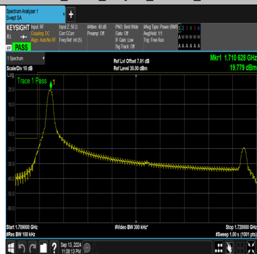
Band66_10MHz_16QAM_132022_1RB#0
