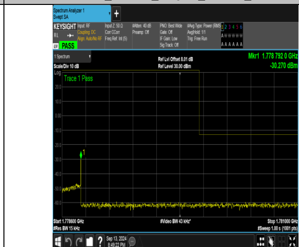
Band66_1.4MHz_16QAM_132665_6RB#0
