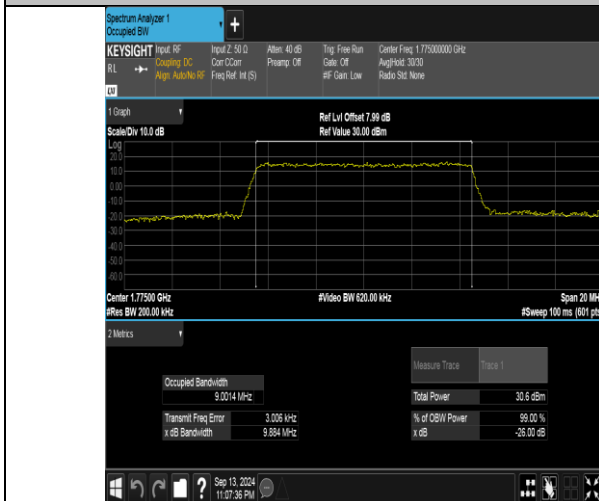
Band66-10MHz-QPSK-132622-50RB#0-PASS
