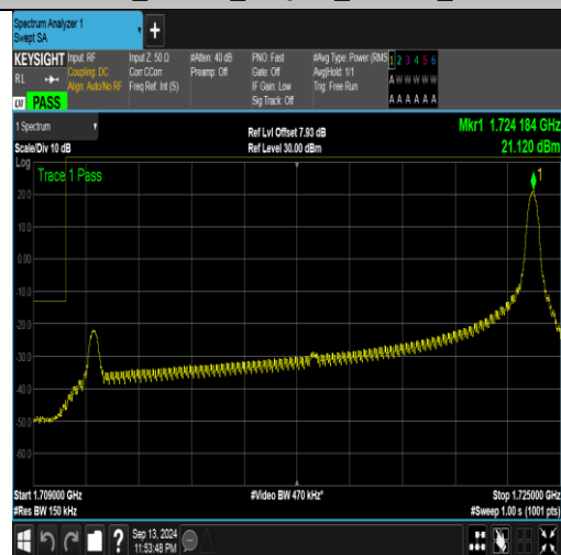
Band66_15MHz_16QAM_132047_1RB#74
