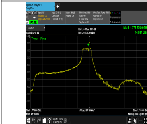
Band66_1.4MHz_QPSK_132665_1RB#5
