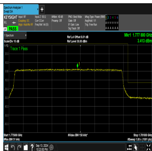
Band66_5MHz_16QAM_132647_25RB#0
