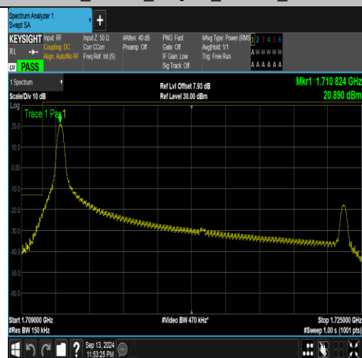
Band66_15MHz_16QAM_132047_1RB#0
