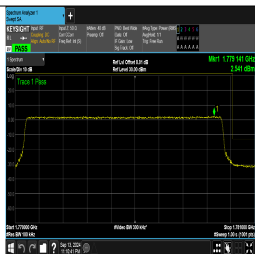
Band66_10MHz_16QAM_132622_50RB#0
