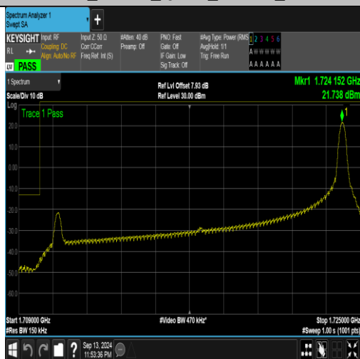
Band66_15MHz_QPSK_132047_1RB#74
