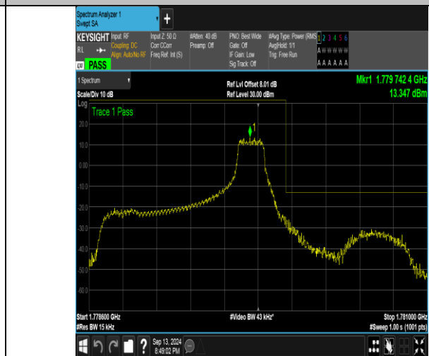
Band66_1.4MHz_16QAM_132665_1RB#5
