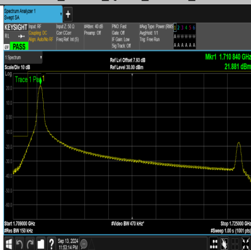
Band66_15MHz_QPSK_132047_1RB#0
