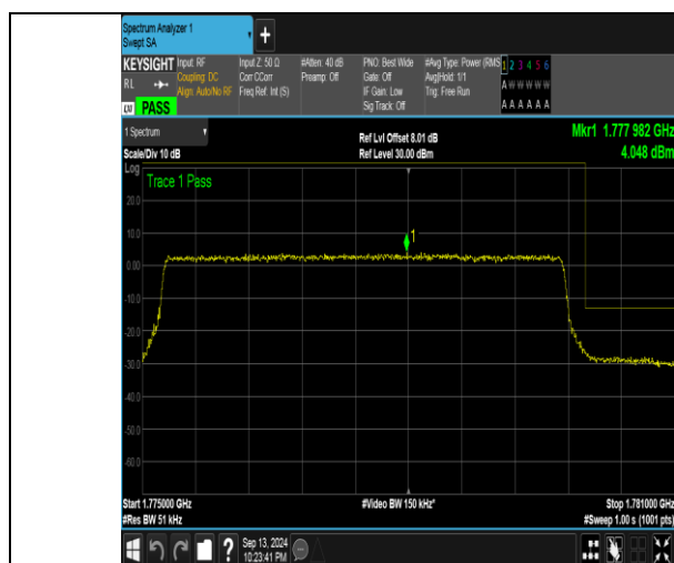
Band66_5MHz_QPSK_132647_25RB#0
