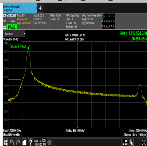
Band66_10MHz_QPSK_132022_1RB#0
