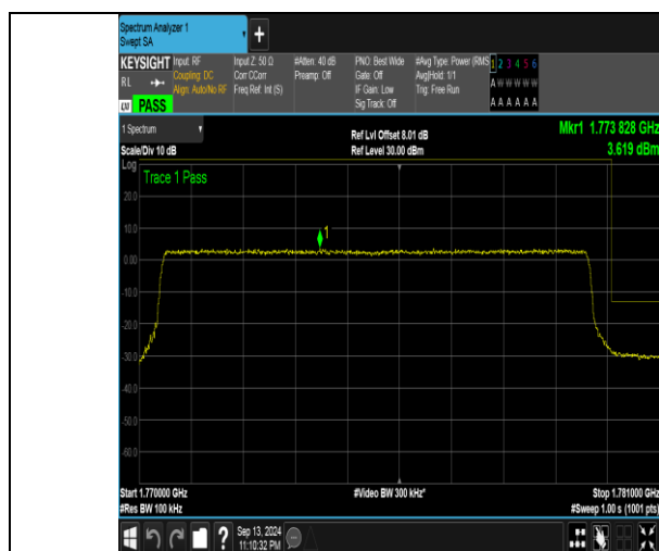
Band66_10MHz_QPSK_132622_50RB#0
