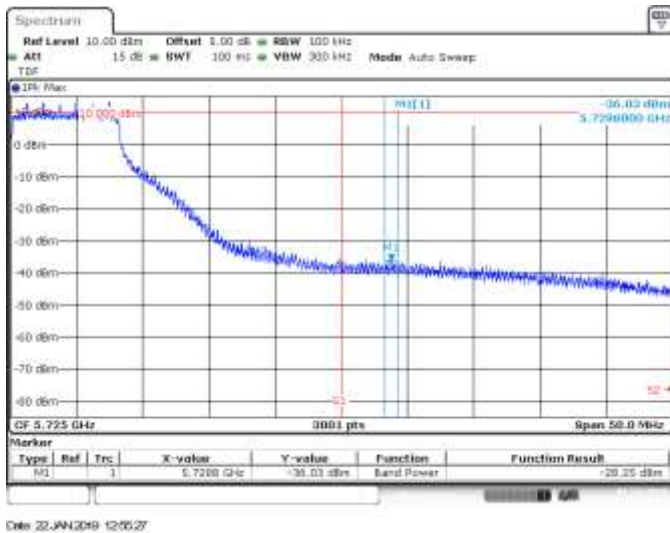
SISO A, 802.11a, 6Mbps, CH140, BE High Peak
