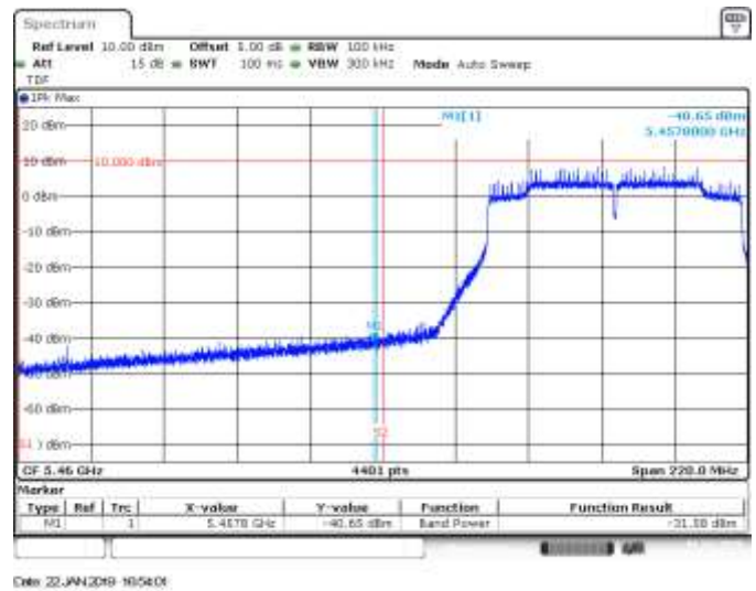
SISO A, 802.11ac80, VHT0, CH106, BE Low Peak (Restricted)
