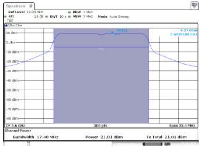
SISO B, CH120, 802.11a, 6Mbps
