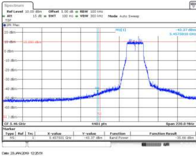
SISO B, 802.11ax20, HE0, CH100, BE Low Peak (Restricted)
