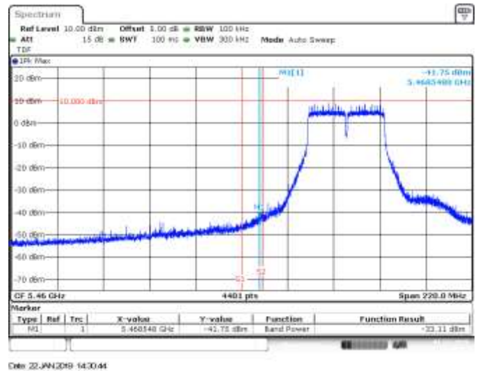
MIMO A, 802.11n40, HT8, CH102, BE Low Peak (Non Restricted)
