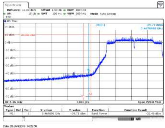
MIMO B, 802.11ac80, VHT0, CH106, BE Low Peak (Non Restricted)
