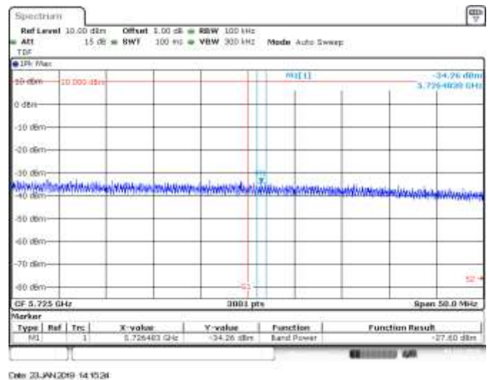
SISO B, 802.11ac80, VHT0, CH122, BE High Peak
