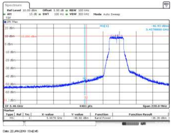
MIMO A, 802.11ax20, HE0, CH100, BE Low Peak (Restricted)
