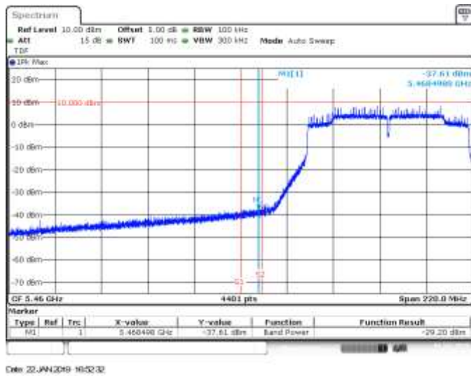
SISO A, 802.11ac80, VHT0, CH106, BE Low Peak (Non Restricted)
