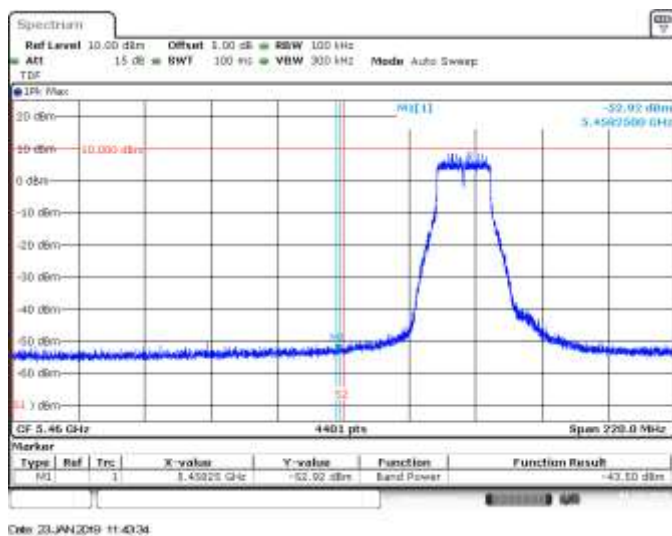
MIMO B, 802.11n20, HT8, CH100, BE Low Peak (Restricted)
