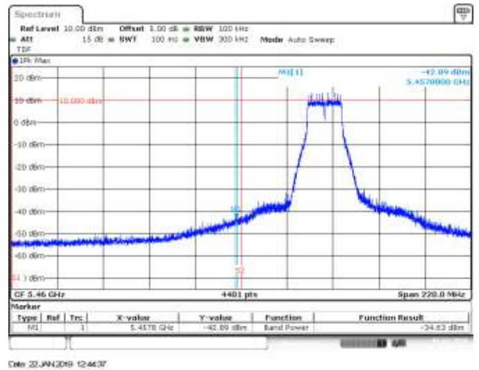
SISO A, 802.11a, 6Mbps, CH100, BE Low Peak (Restricted)
