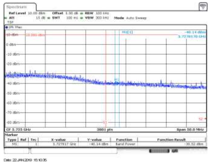
MIMO A, 802.11n40, HT8, CH134, BE High Peak
