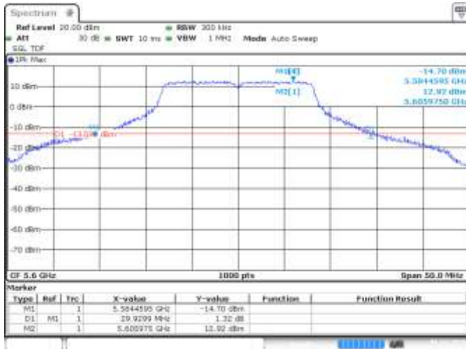
SISO A, CH120, 802.11a, 6Mbps, 26dB
