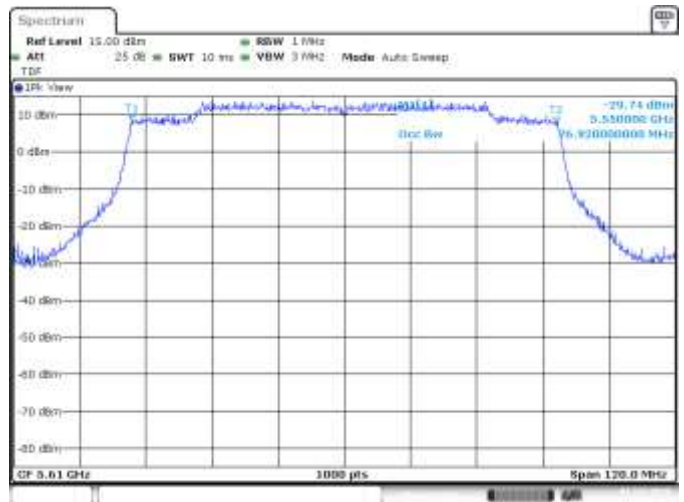
SISO B, CH122, 802.11ax80, HE0, 99%
