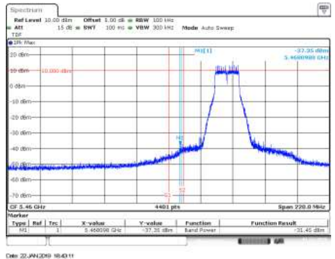
SISO B, 802.11a, 6Mbps, CH100, BE Low Peak (Non Restricted)
