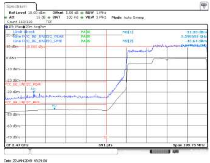
SISO A, 802.11ax160, HE0, CH114, BE Low RMS, Peak
