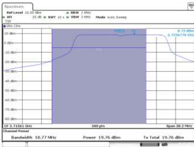
SISO A, 802.11n20, Overlapped CH144
