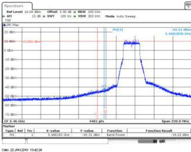
MIMO A, 802.11ax20, HE0, CH100, BE Low Peak (Non Restricted)
