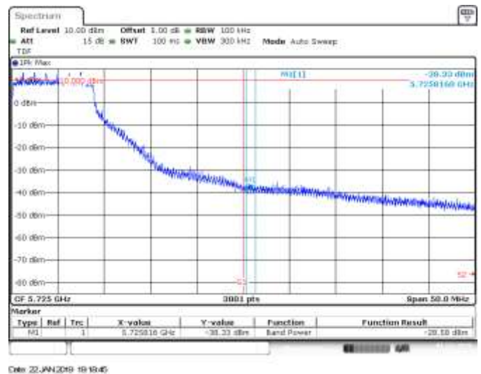
SISO B, 802.11n20, HT0, CH140, BE High Peak
