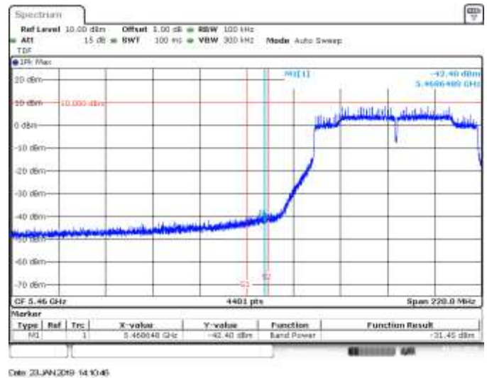
SISO B, 802.11ac80, VHT0, CH106, BE Low Peak (Non Restricted)
