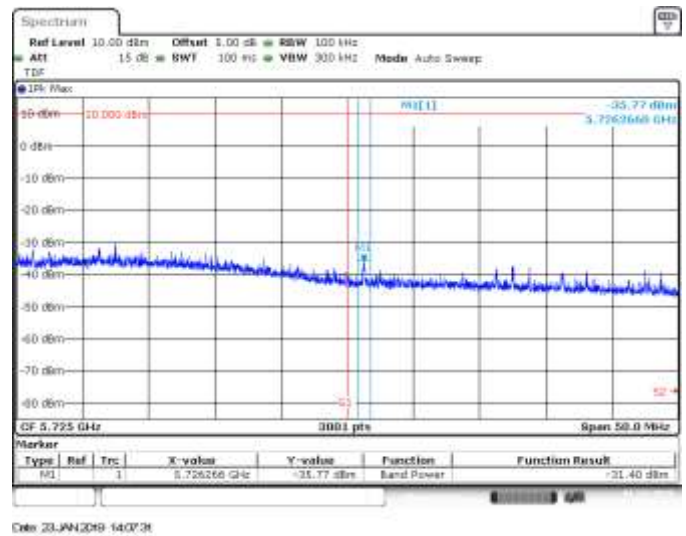
MIMO B, 802.11ax40, HE0, CH134, BE High Peak
