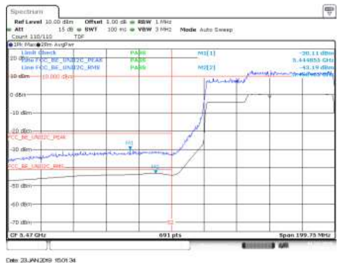
SISO B, 802.11ax160, HE0, CH114, BE Low RMS, Peak
