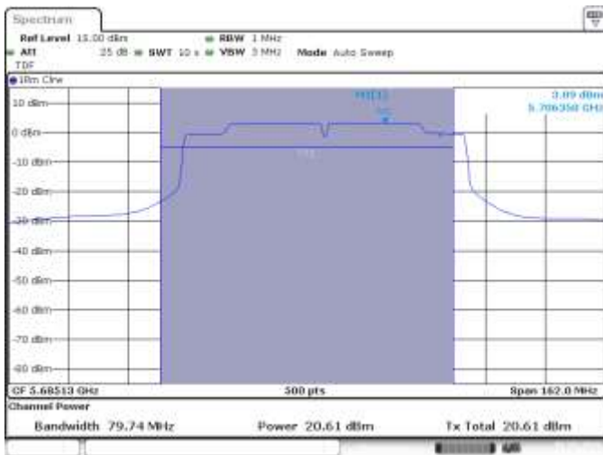
SISO A, 802.11ac80, Overlapped CH138
