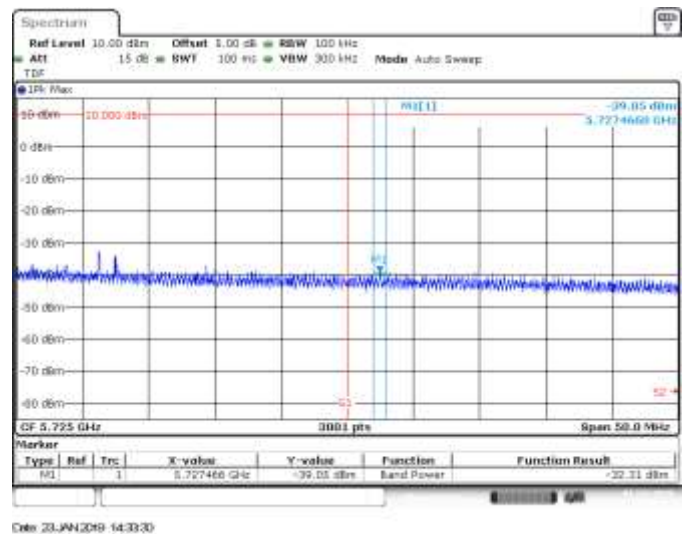
MIMO B, 802.11ac80, VHT0, CH122, BE High Peak
