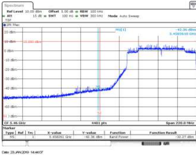
MIMO B, 802.11ax80, HE0, CH106, BE Low Peak (Restricted)
