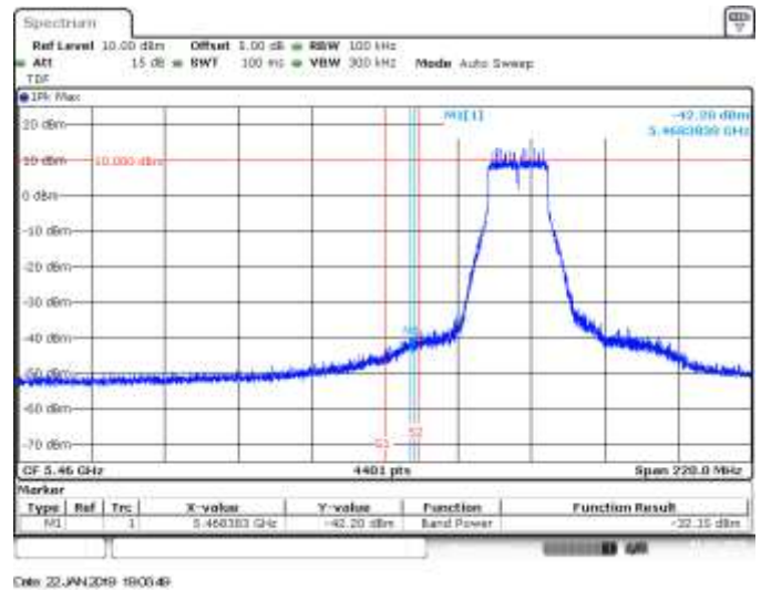
SISO B, 802.11n20, HT0, CH100, BE Low Peak (Non Restricted)
