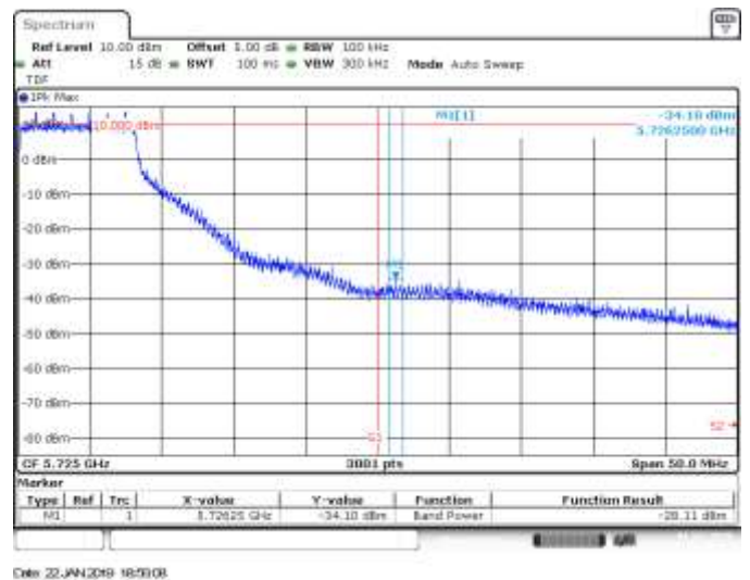
SISO B, 802.11a, 6Mbps, CH140, BE High Peak
