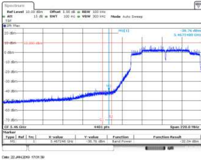
MIMO A, 802.11ac80, VHT0, CH106, BE Low Peak (Non Restricted)
