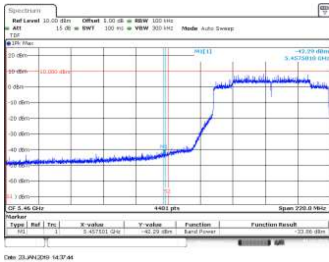
SISO B, 802.11ax80, HE0, CH106, BE Low Peak (Restricted)
