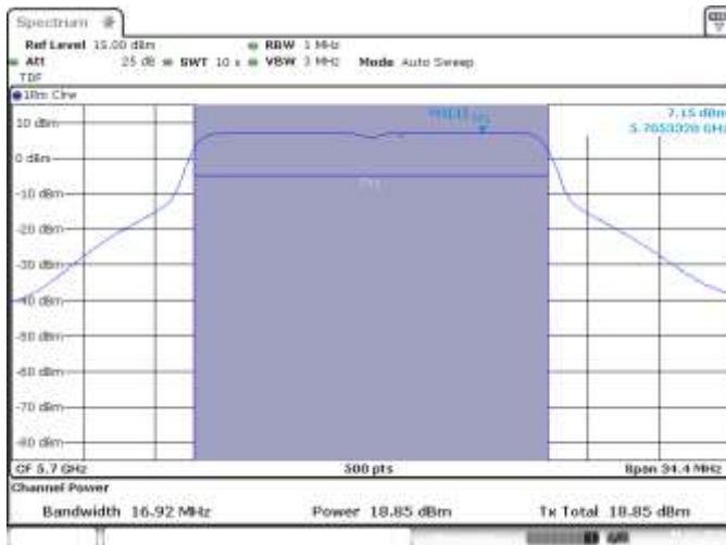
SISO A, CH140, 802.11a, 6Mbps
