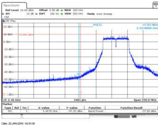
MIMO A, 802.11n40, HT8, CH102, BE Low Peak (Restricted)
