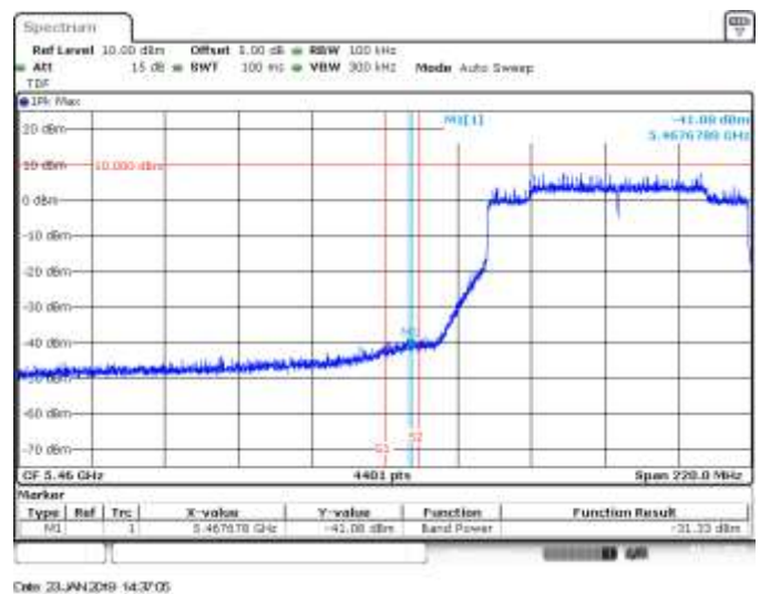
SISO B, 802.11ax80, HE0, CH106, BE Low Peak (Non Restricted)
