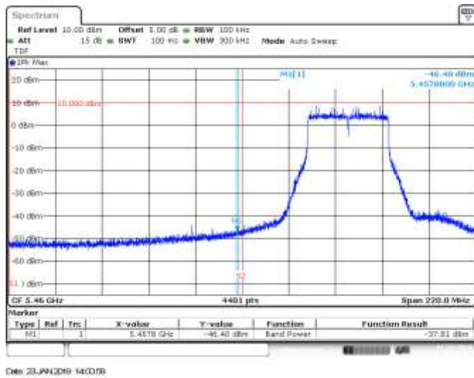
MIMO B, 802.11ax40, HE0, CH102, BE Low Peak (Restricted)
