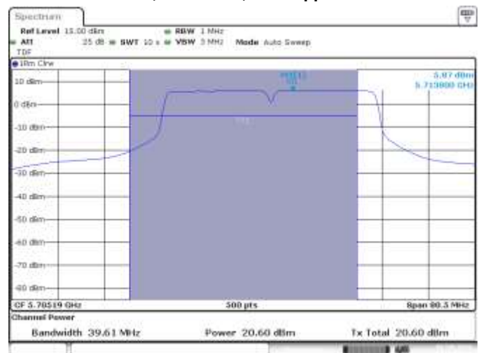
SISO B, 802.11n40, Overlapped CH142
