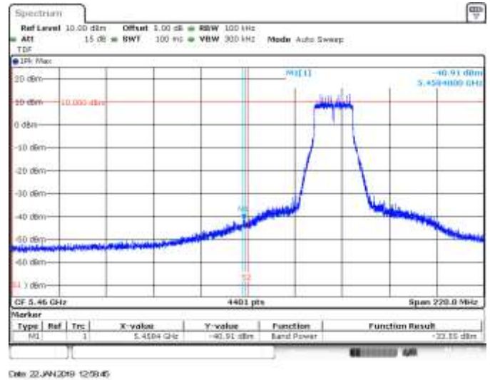
SISO A, 802.11n20, HT0, CH100, BE Low Peak (Restricted)
