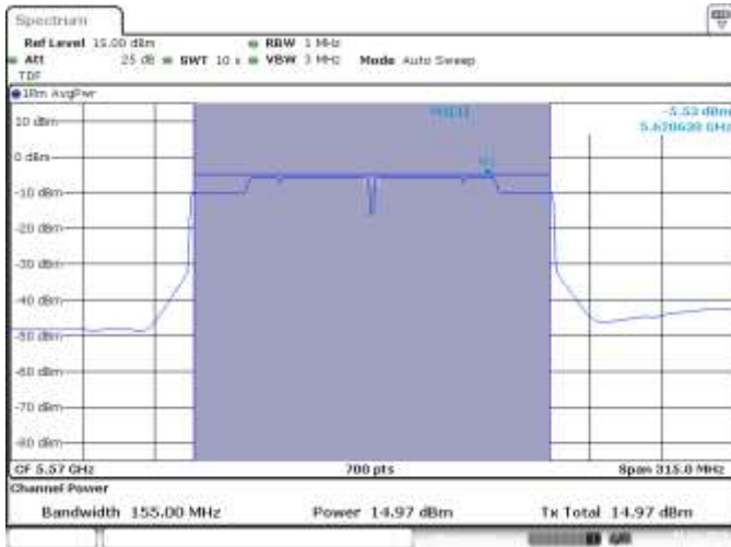
SISO A, CH114, 802.11ax160, HE0
