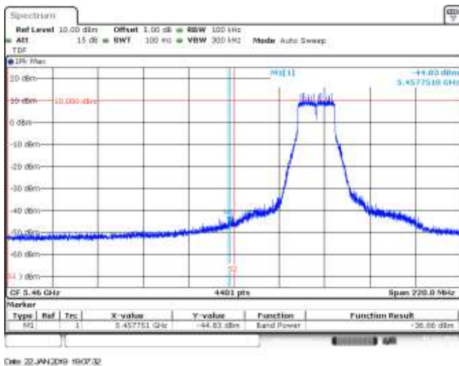
SISO B, 802.11n20, HT0, CH100, BE Low Peak (Restricted)
