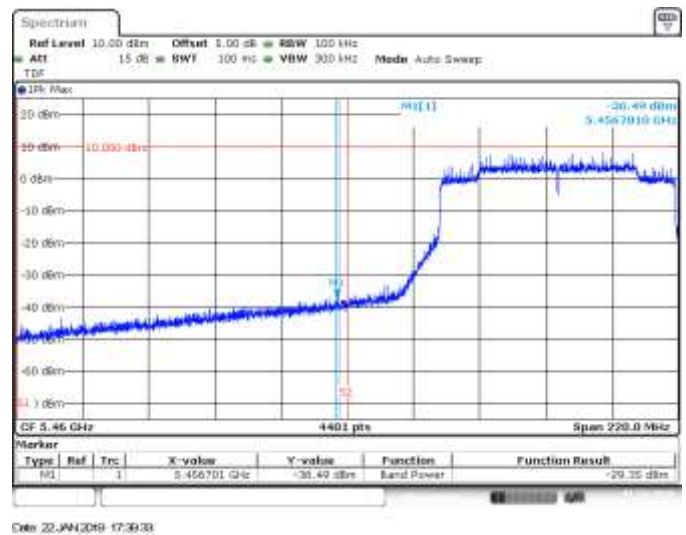
SISO A, 802.11ax80, HE0, CH106, BE Low Peak (Restricted)
