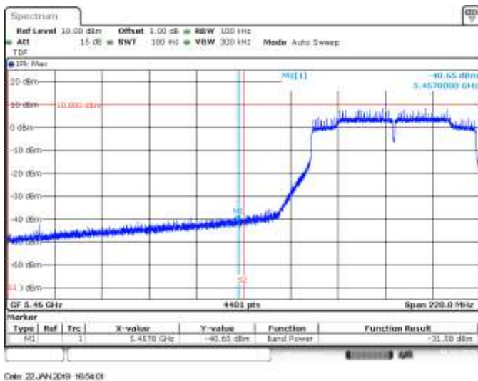
MIMO B, 802.11ac80, VHT0, CH106, BE Low Peak (Restricted)
