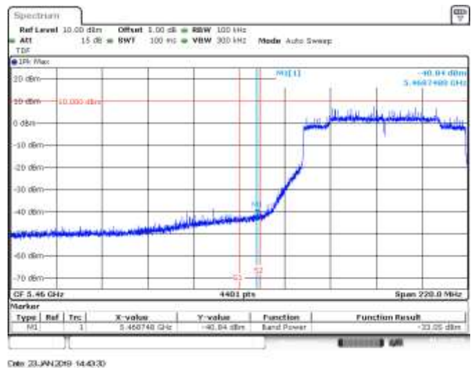
MIMO B, 802.11ax80, HE0, CH106, BE Low Peak (Non Restricted)
