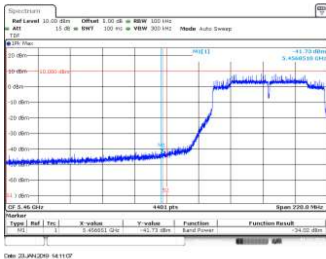
SISO B, 802.11ac80, VHT0, CH106, BE Low Peak (Restricted)
