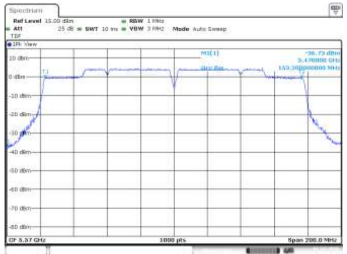
SISO B, CH114, 802.11ac160, VHT0, 99%
