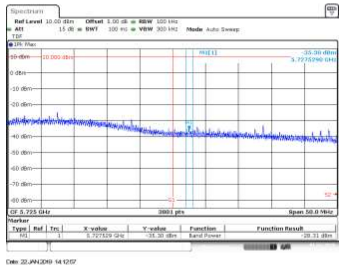
SISO A, 802.11n40, HT0, CH134, BE High Peak
