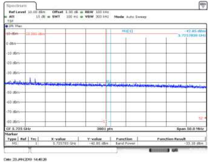
MIMO B, 802.11ax80, HE0, CH122, BE High Peak
