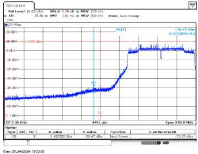
MIMO A, 802.11ac80, VHT0, CH106, BE Low Peak (Restricted)
