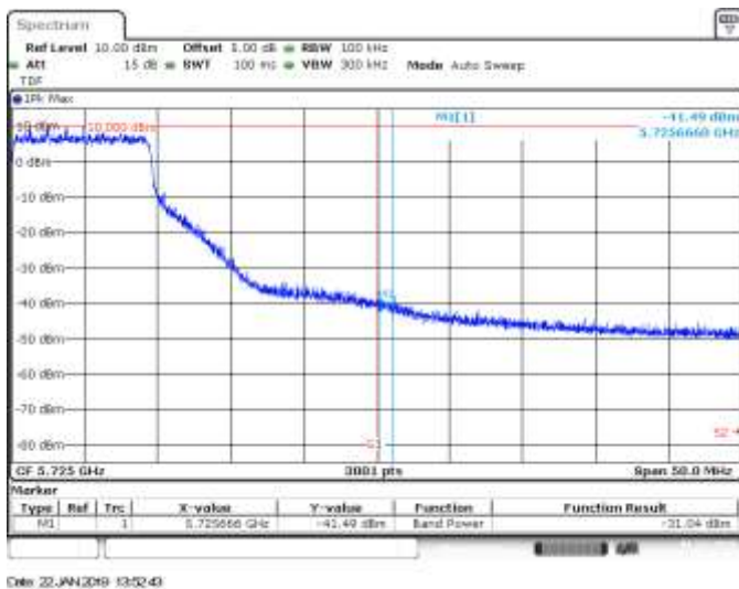
MIMO A, 802.11ax20, HE0, CH140, BE High Peak
