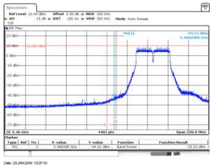
MIMO B, 802.11n20, HT8, CH102, BE Low Peak (Non Restricted)
