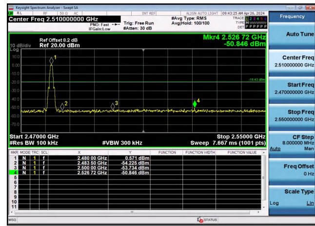
Right bandedge
