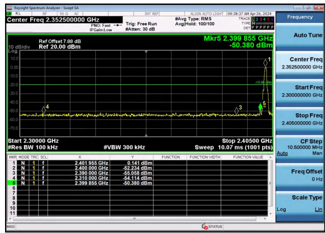
Left bandedge
