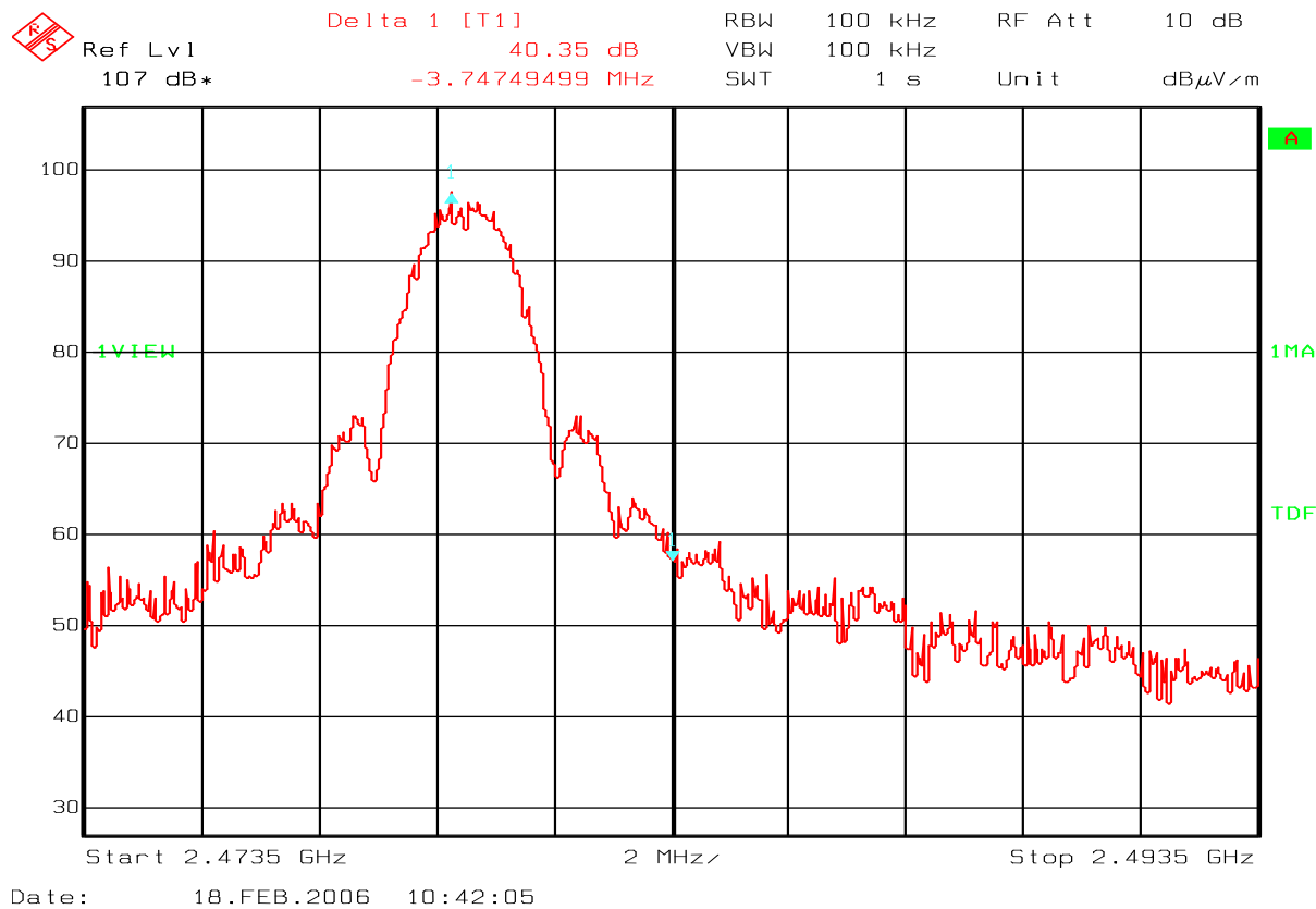
Fig. 9 – 13213-SRB – Ch26 – upper-band – field strength
