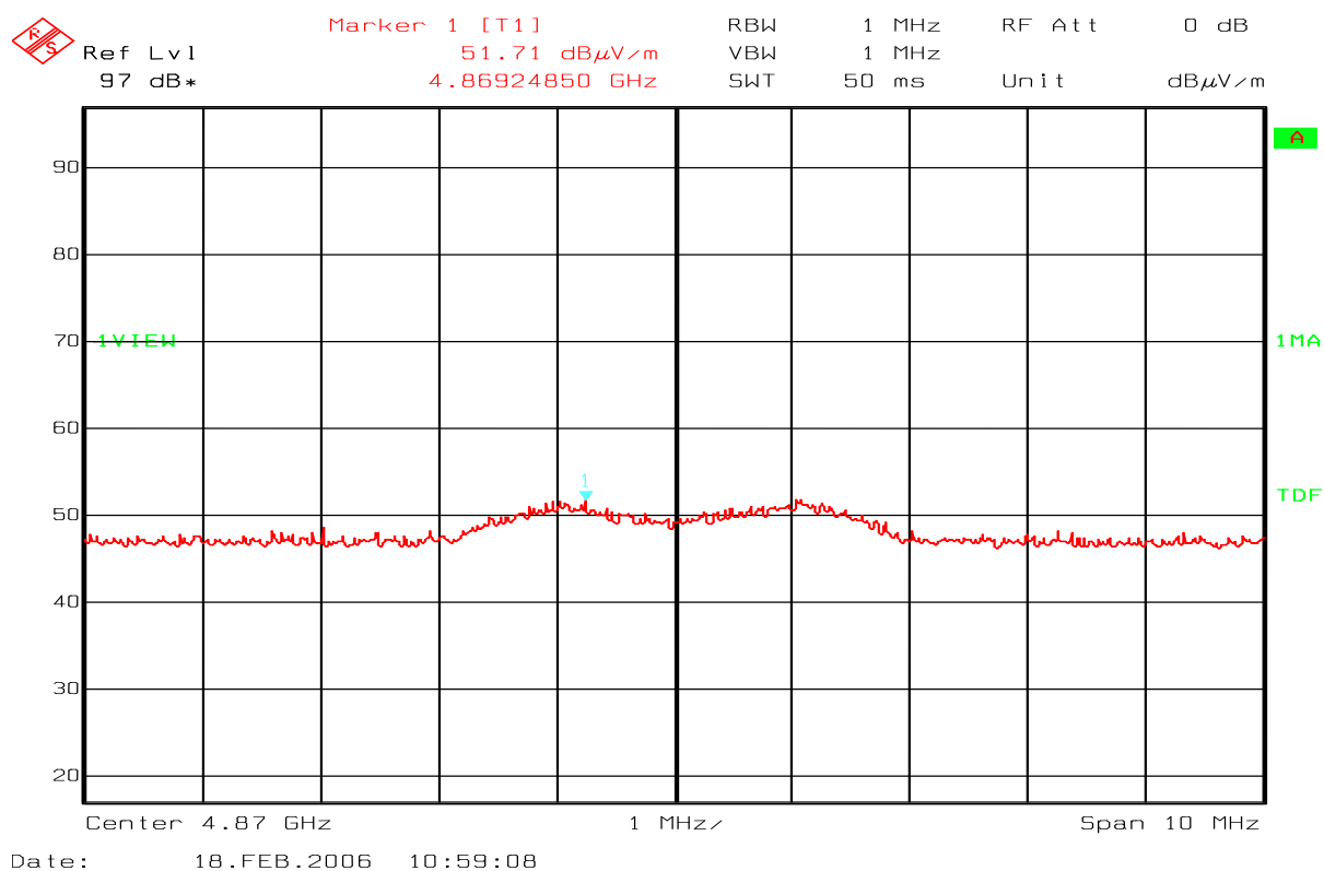
Fig. 17 – 13213 –SRB – Ch17 – 2 nd Harmonic
