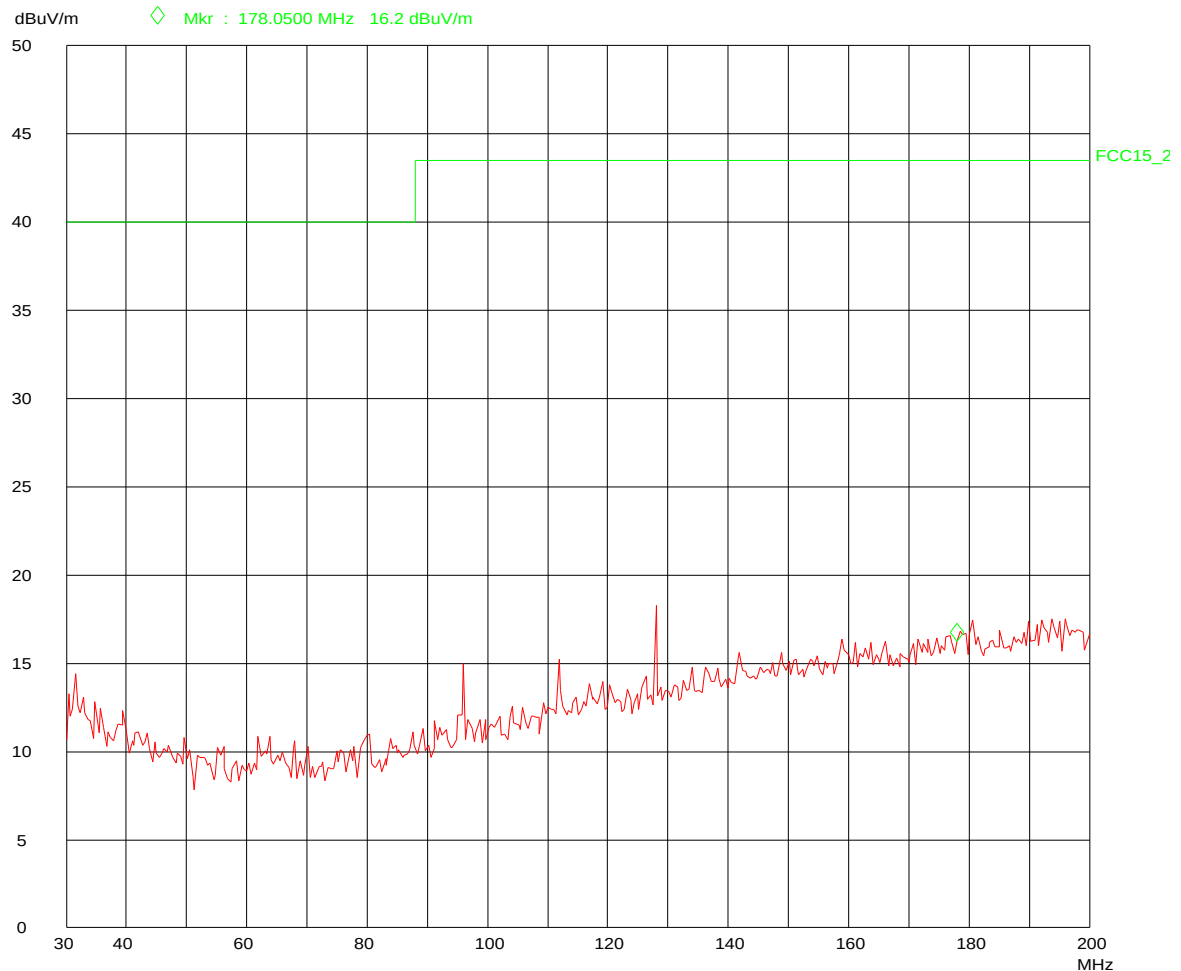
Fig 20 – 13213-SRB – HP – 30 – 200MHz
