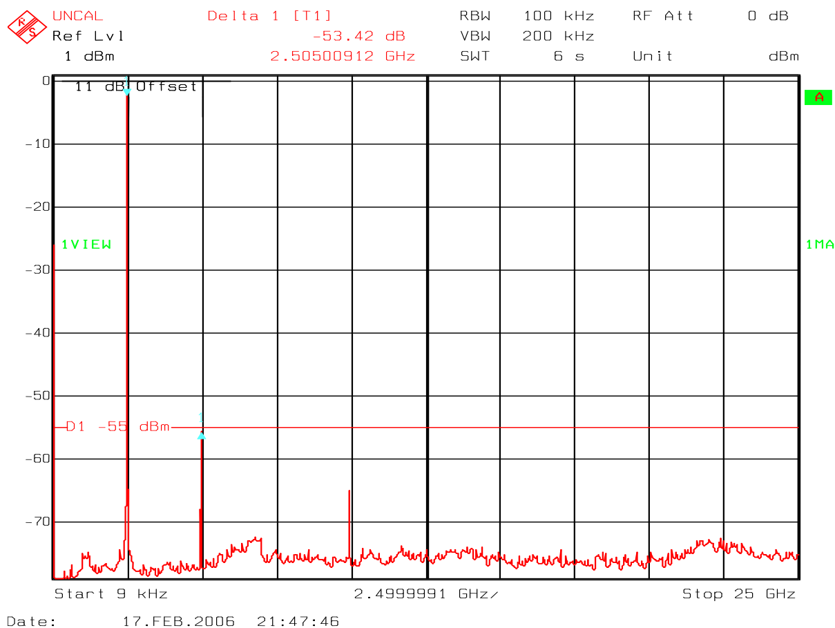
Fig. 13 – 13213-SRB - Ch26 – Conducted Spurious – 9kHz – 25GHz
