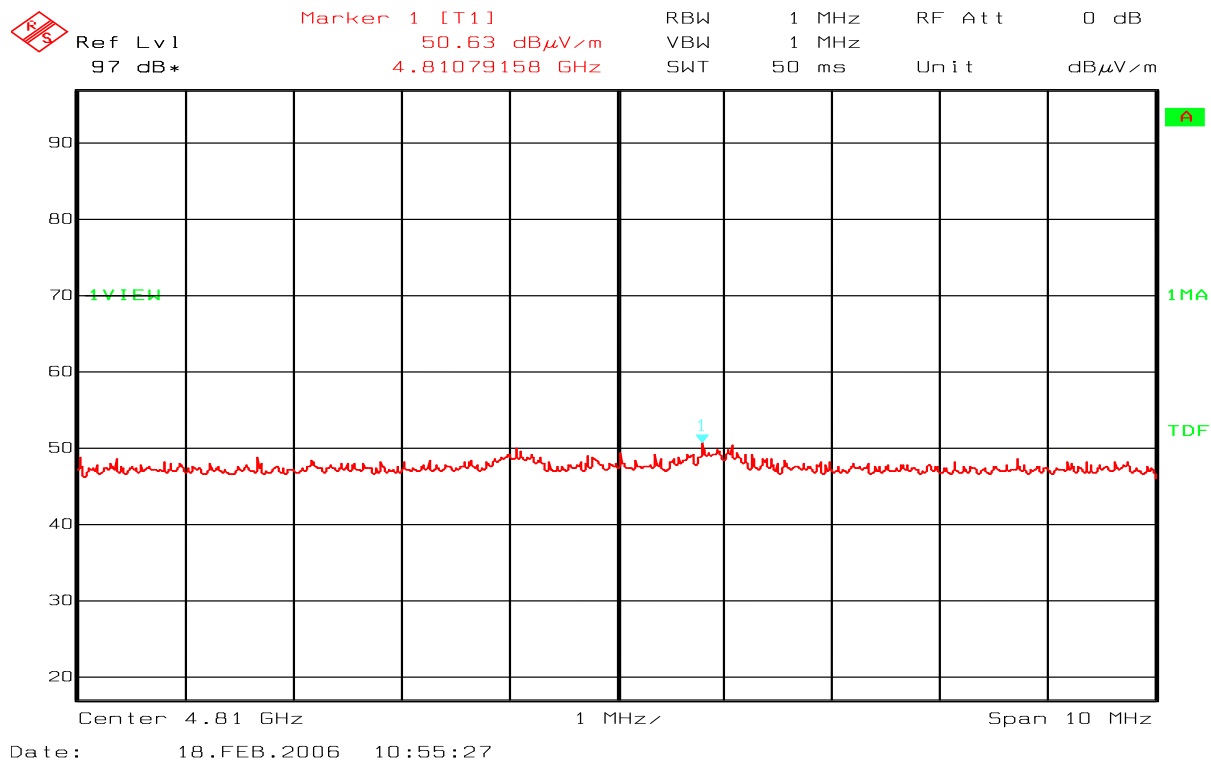
Fig. 16 – 13213 –SRB – Ch11 – 2 nd Harmonic
