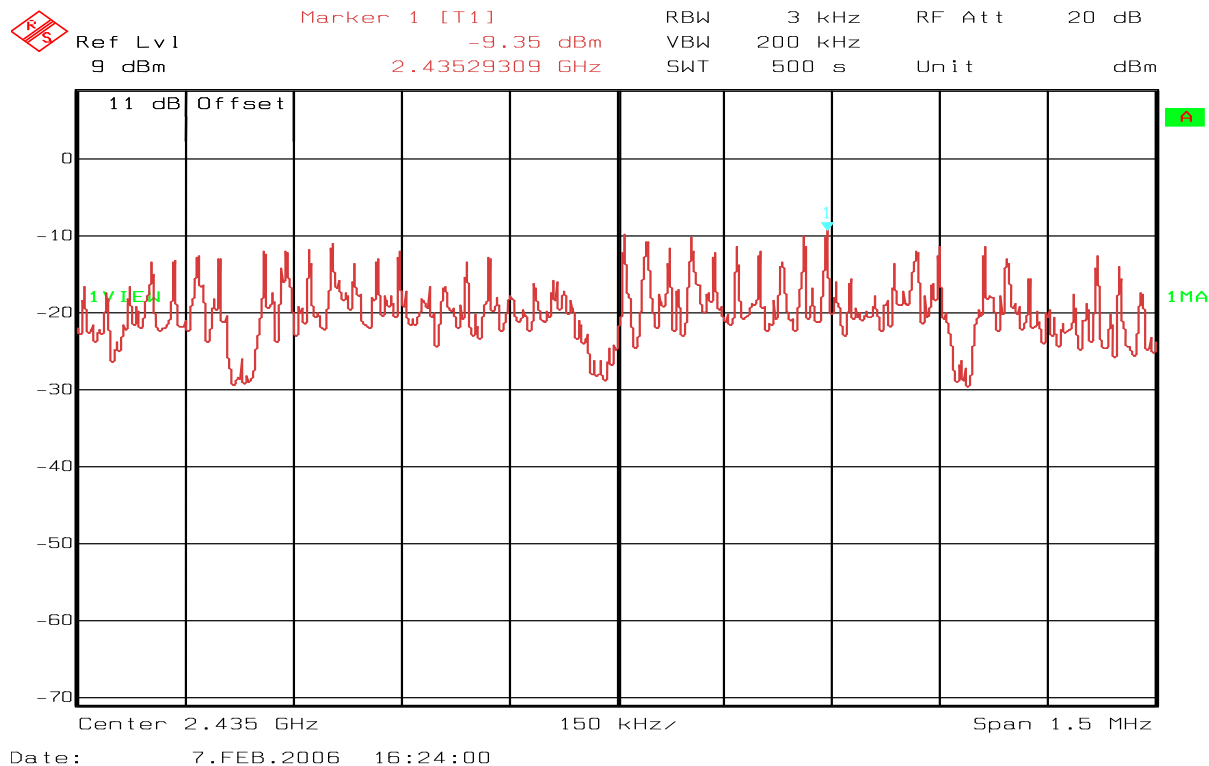
Fig 25- 13213-SRB – Ch17 – Power Density – Conducted measurement
