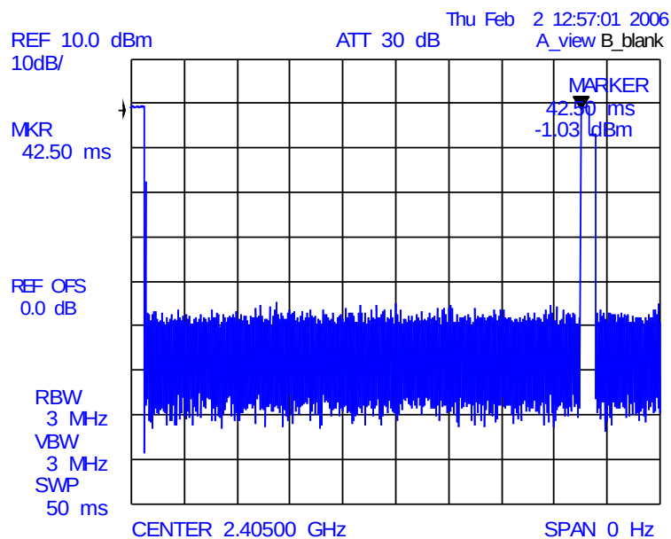
Fig 15 – 13213-SRB – Duty Cycle – OFF-time
