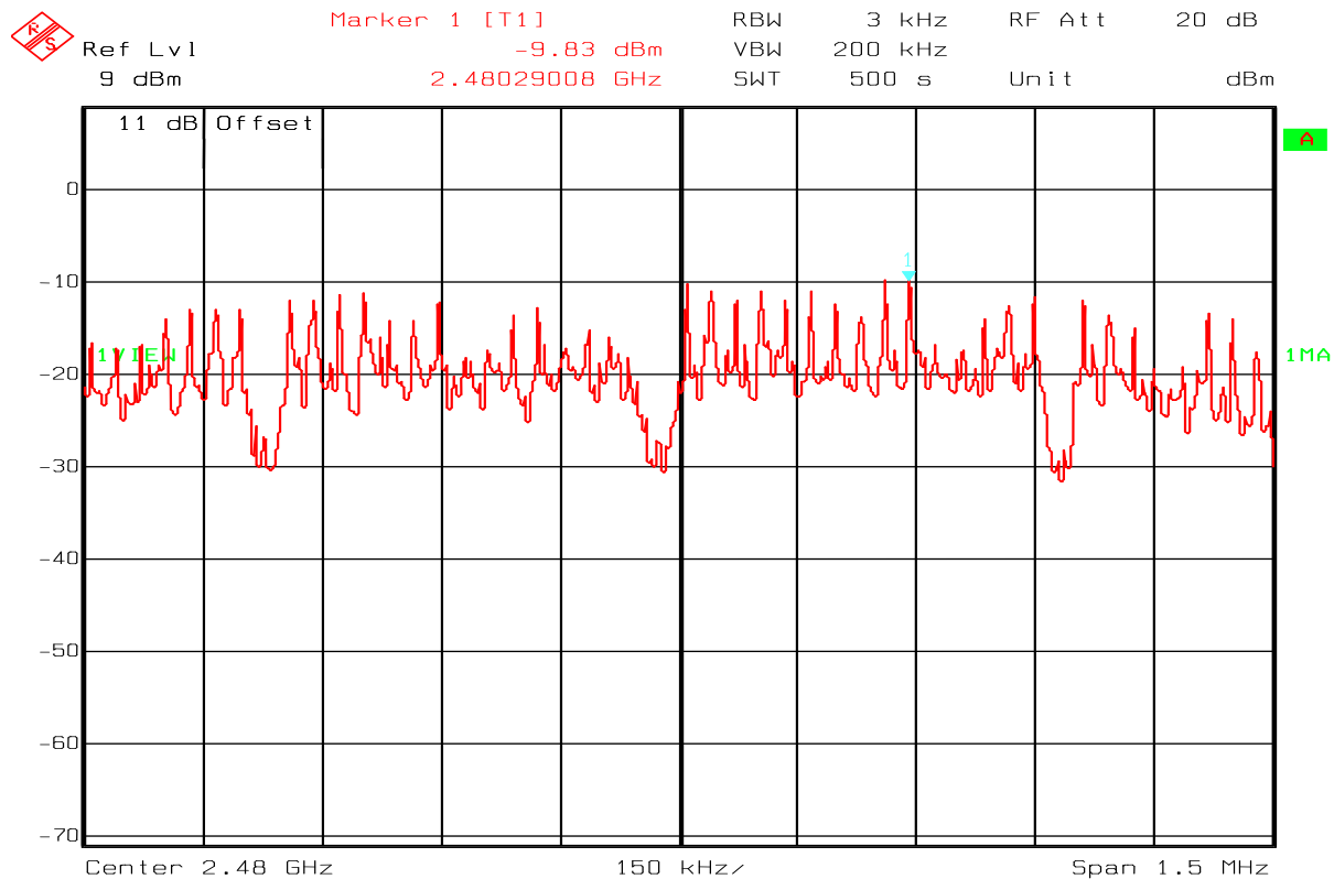
Fig 26- 13213-SRB – Ch26 – Power Density – Conducted measurement
