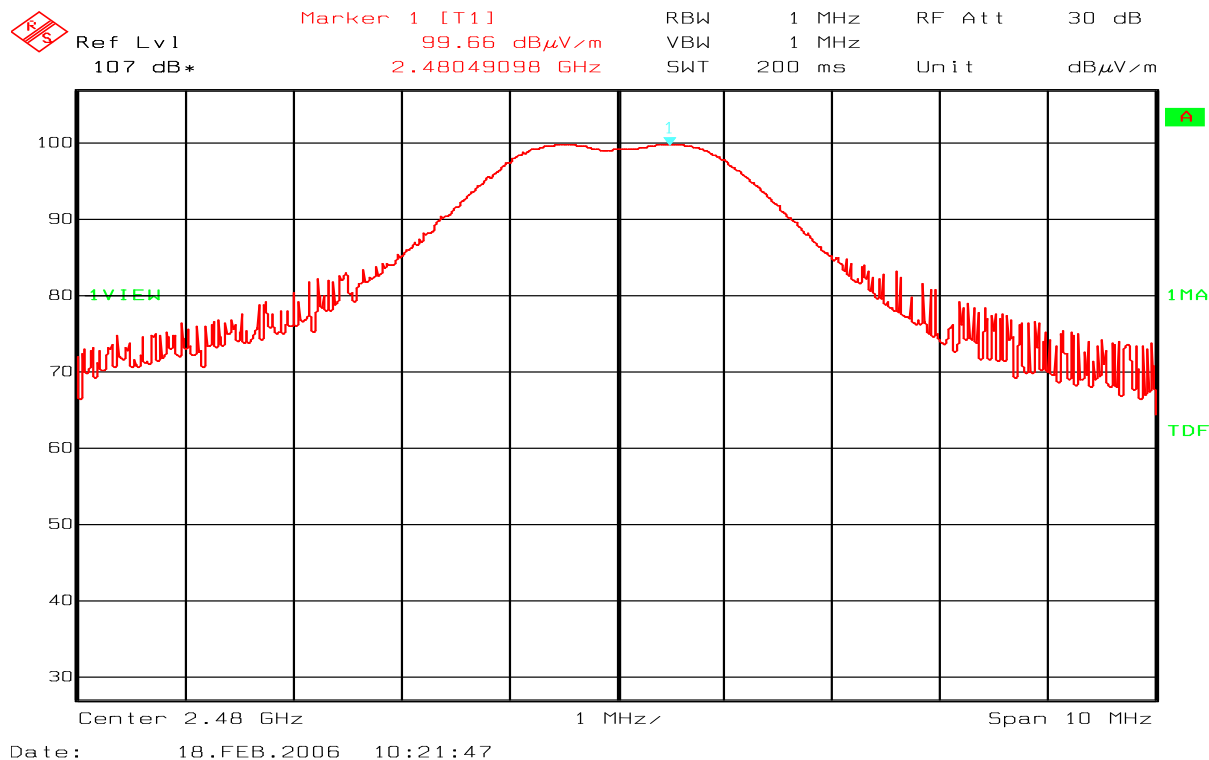
Fig. 9 – 13213-SRB – Ch26 – upper-band – field strength
