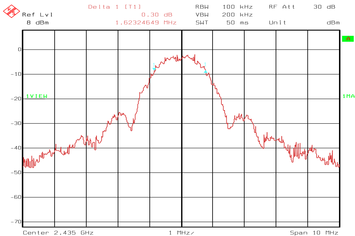
Fig 3 – 13213 –SRB – Ch11 – 6 dB bandwidth – 1.62MHz
