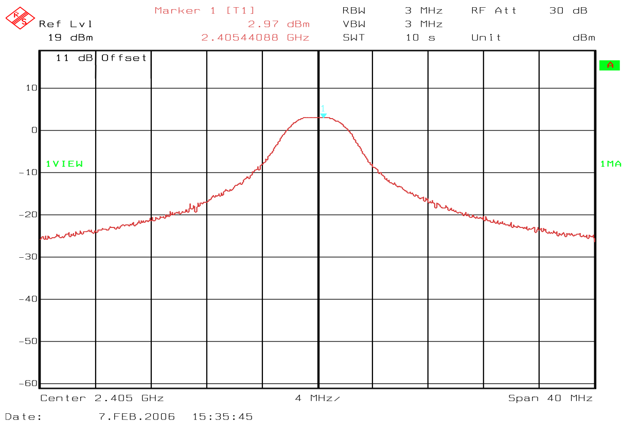
Fig 6 – 13213-SRB – Ch11 – Conducted Peak out-put power
