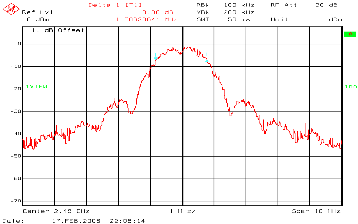
Fig 5 – 13213 –SRB – Ch26 – 6 dB bandwidth – 1.60MHz
