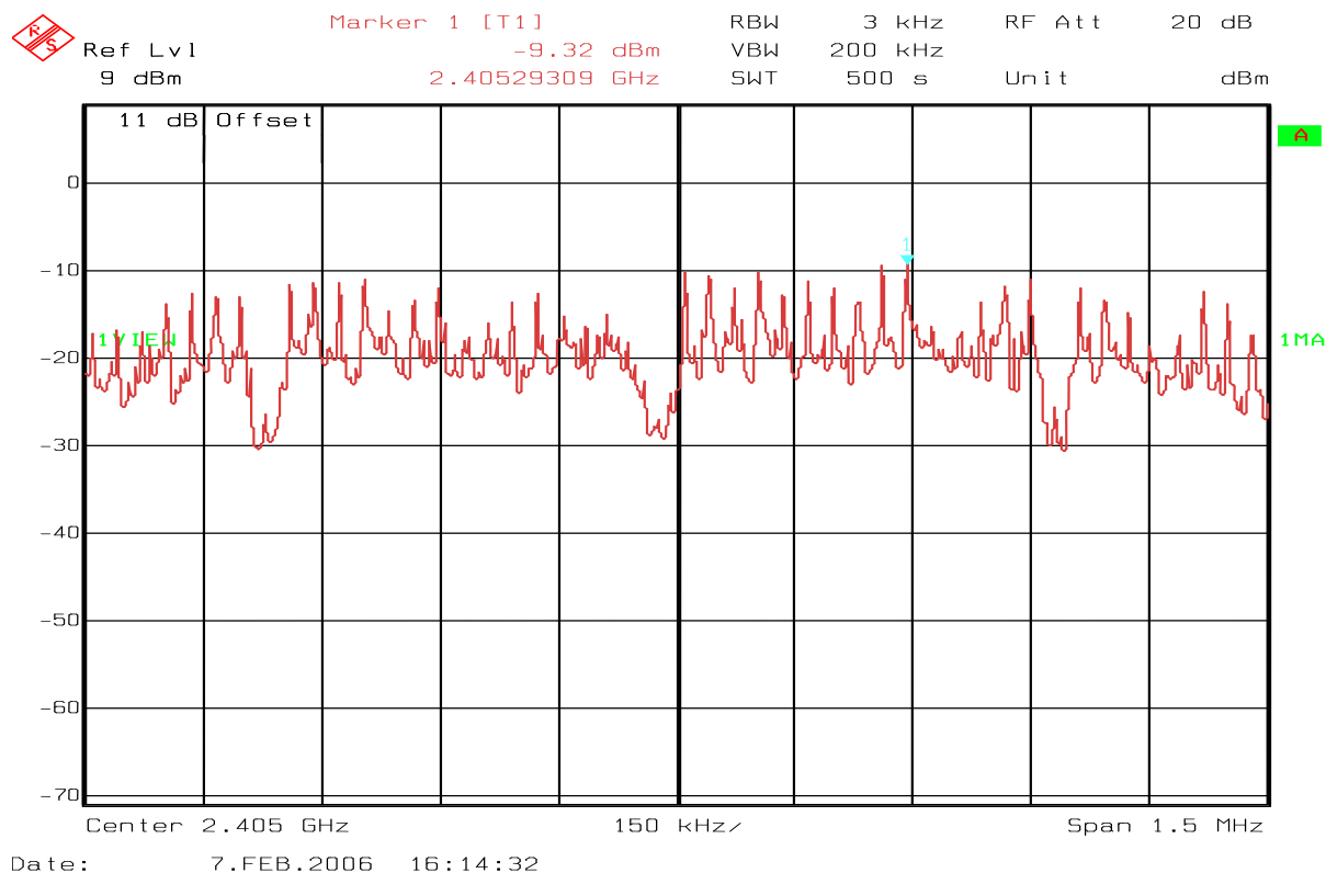
Fig 24- 13213-SRB – Ch11 – Power Density – Conducted measurement
