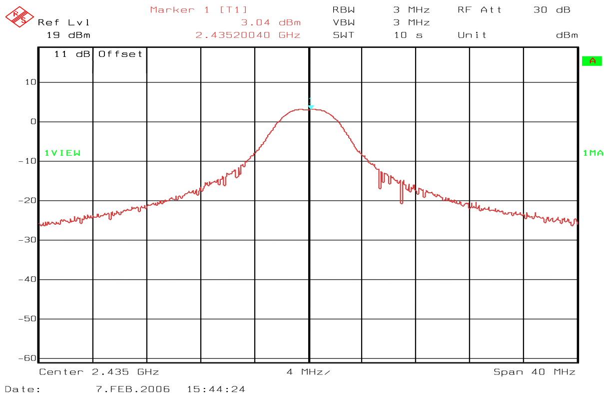
Fig 7 – 13213-SRB – Ch17 – Conducted Peak out-put power
