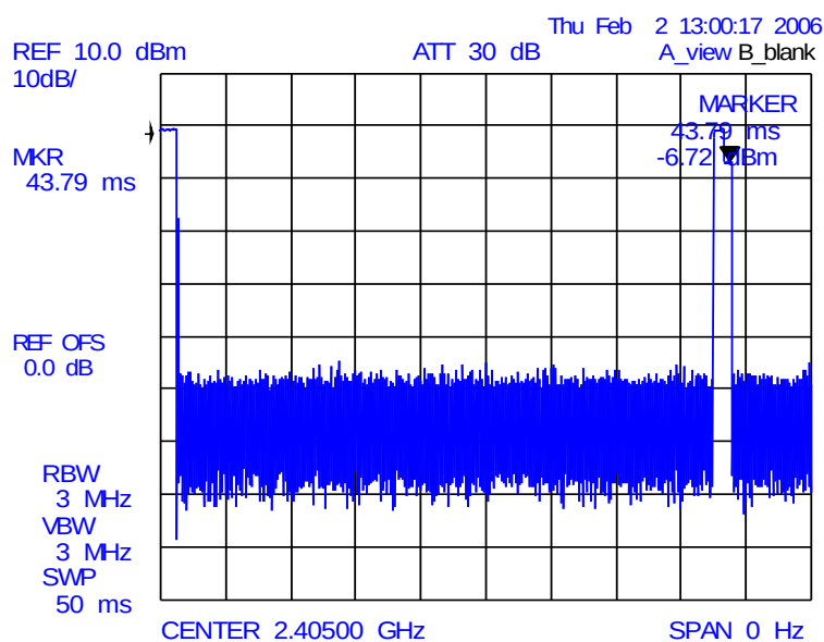
Fig 14– 13213-SRB – Duty Cycle – ON-time
