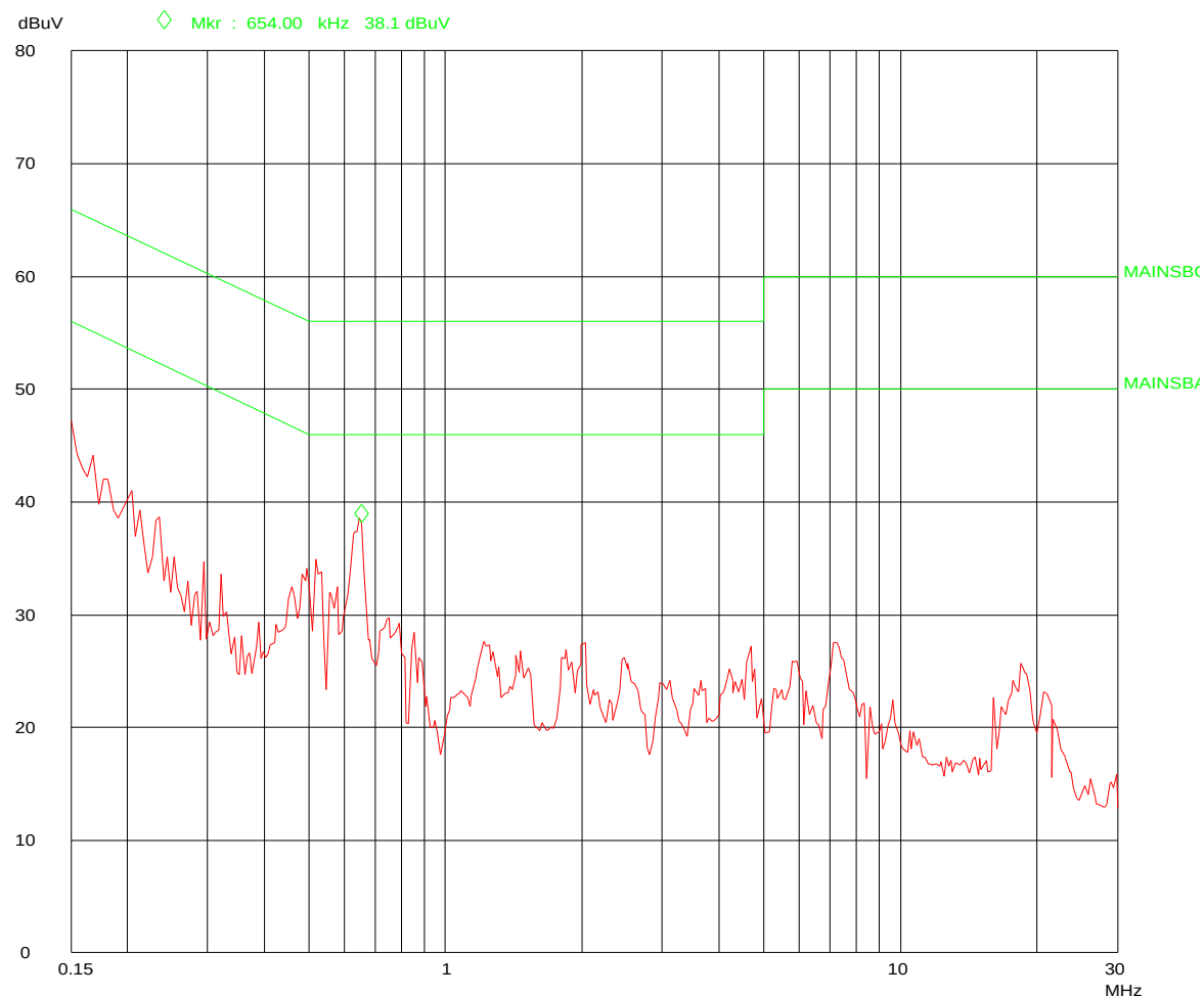
Fig 2 – N polarity – 13213-SRB
