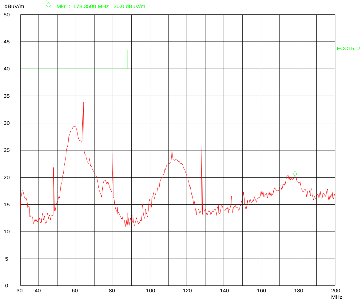
Fig 19 – 13213 –SRB – VP – 30 – 200 MHz
