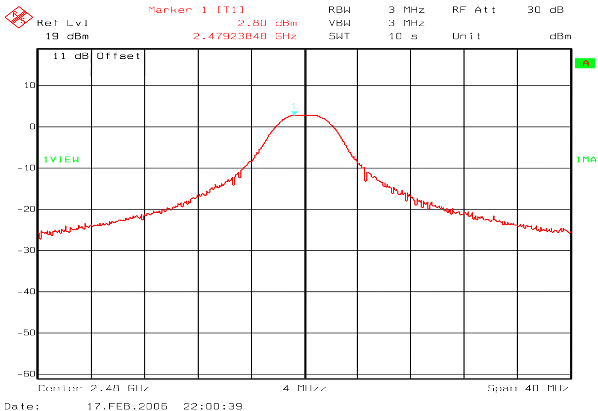
Fig 8 – 13213-SRB – Ch26 – Conducted Peak out-put power
