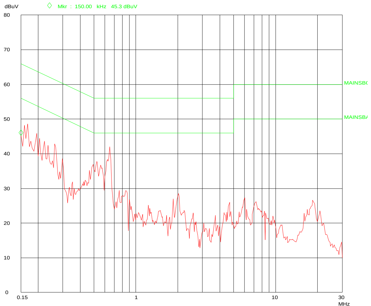
Fig 1 – L1 polarity – 13213-SRB
