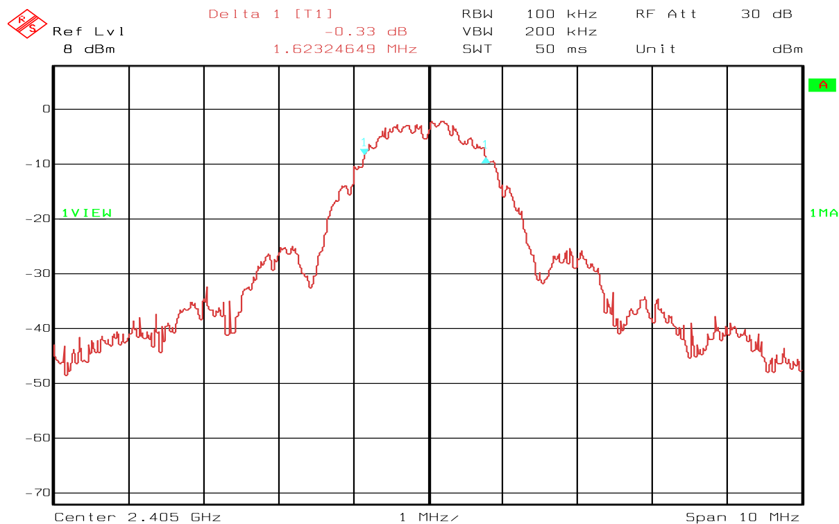
Fig 3 – 13213 –SRB – Ch11 – 6 dB bandwidth – 1.62MHz
