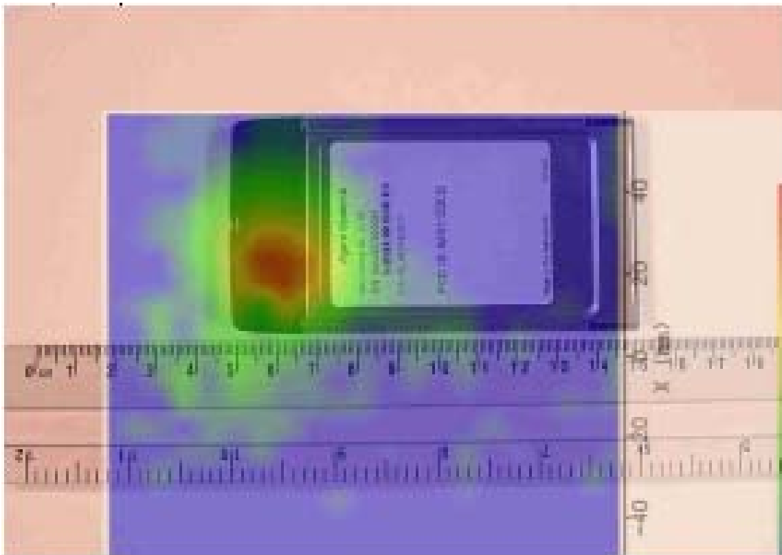
Figure 1: 5 GHz contour plot entire device
