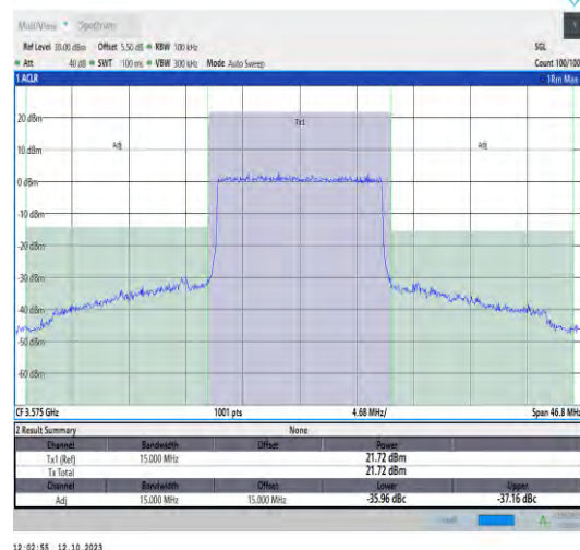
42(3550-3600)-15MHz-QPSK-43340-75RB#0-PASS
