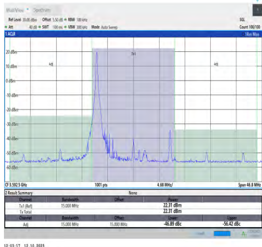
42(3550-3600)-15MHz-QPSK-43515-1RB#0-PASS
