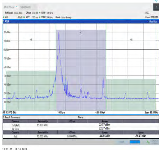
42(3550-3600)-15MHz-QPSK-43165-1RB#0-PASS
