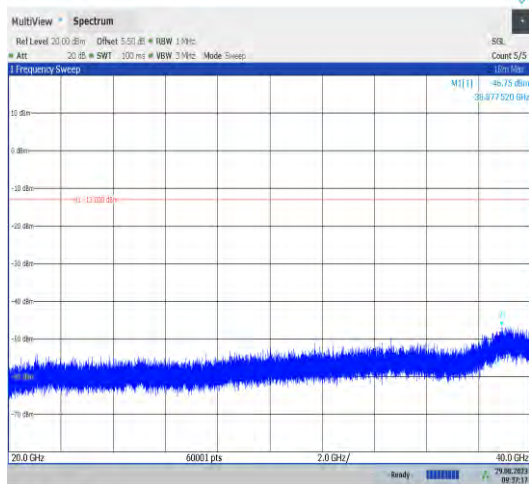
Band42_20MHz_QPSK_43190_1RB#0_20000~40000_20000~40000
