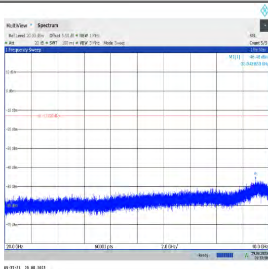
Band42_20MHz_QPSK_43490_1RB#0_20000~40000_20000~40000
