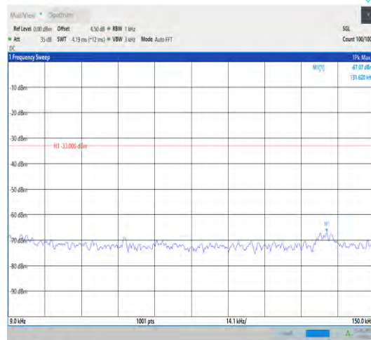
Band42_20MHz_QPSK_43340_1RB#0_0.009~0.15_0.09~0.15
