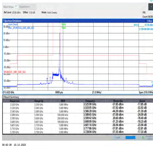
Band22_10MHz_QPSK_43540_1RB#49
