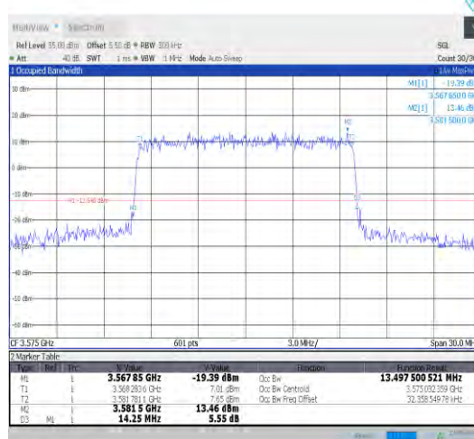
Band42-15MHz-16QAM-43340-75RB#0-PASS
