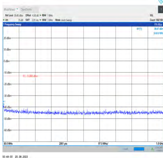
Band42_20MHz_QPSK_43490_1RB#0_30~1000_30~1000
