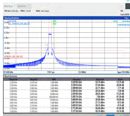
Band42_5MHz_QPSK_43565_25RB#0
