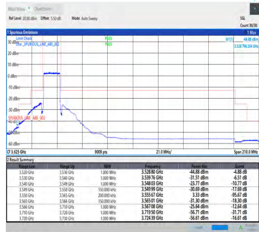
Band22_15MHz_QPSK_43165_75RB#0
