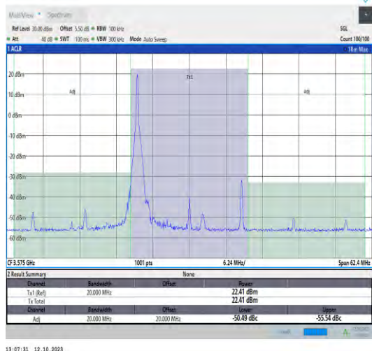
42(3550-3600)-20MHz-QPSK-43340-1RB#0-PASS
