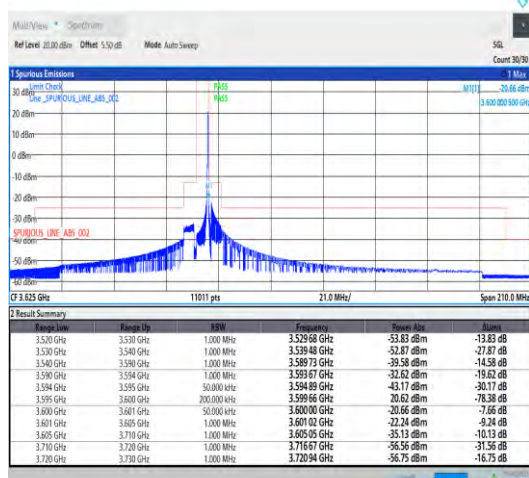
Band42_5MHz_QPSK_43565_1RB#24
