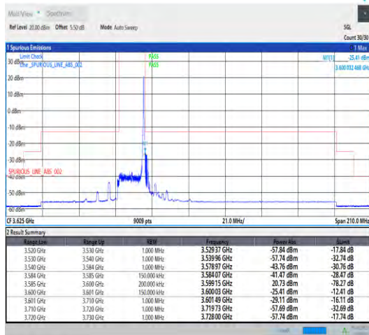
Band22_15MHz_QPSK_43515_1RB#74
