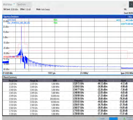
Band42_5MHz_QPSK_43115_1RB#0
