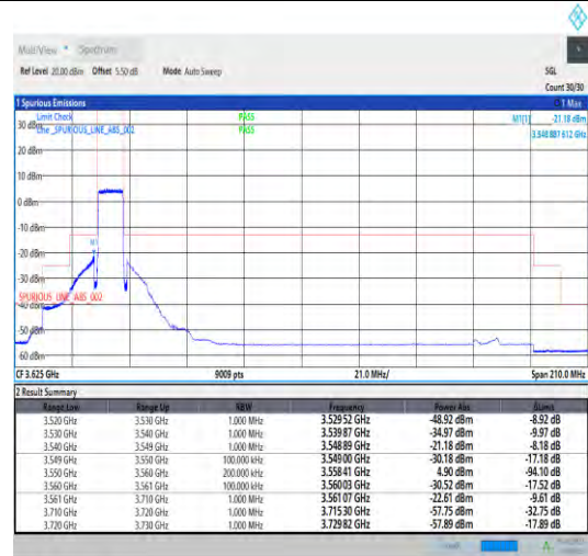
Band22_10MHz_QPSK_43140_50RB#0
