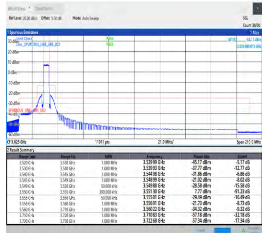
Band42_5MHz_QPSK_43115_25RB#0
