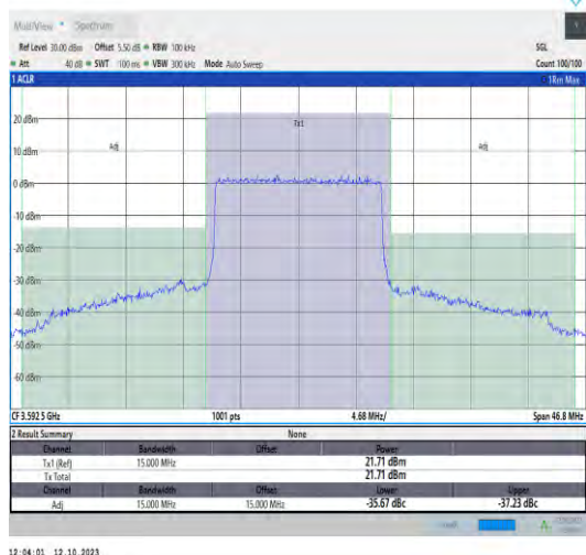
42(3550-3600)-15MHz-QPSK-43515-75RB#0-PASS
