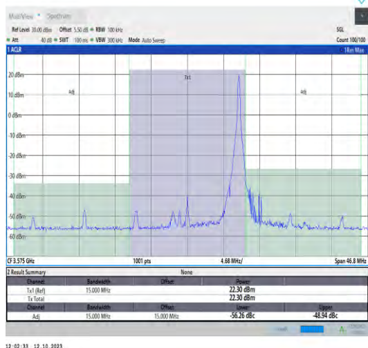
42(3550-3600)-15MHz-QPSK-43340-1RB#74-PASS
