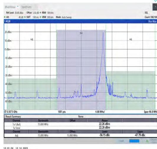
42(3550-3600)-15MHz-QPSK-43165-1RB#74-PASS
