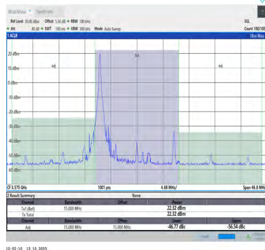
42(3550-3600)-15MHz-QPSK-43340-1RB#0-PASS
