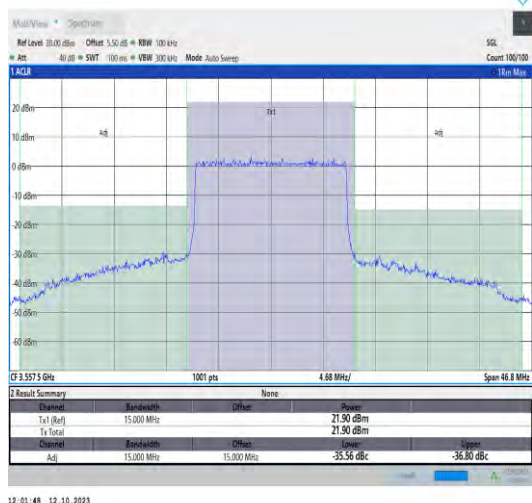
42(3550-3600)-15MHz-QPSK-43165-75RB#0-PASS
