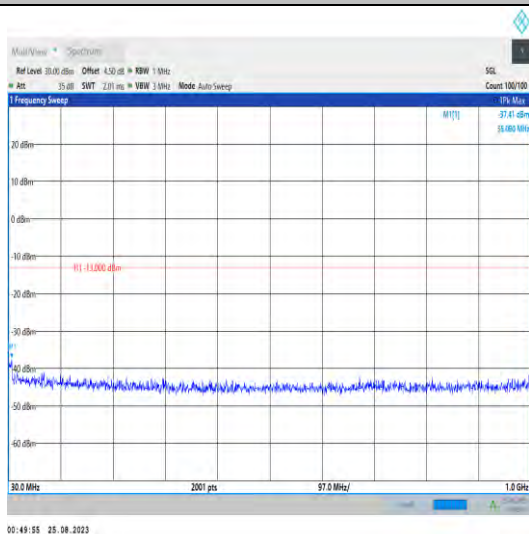
Band42_20MHz_QPSK_43190_1RB#0_30~1000_30~100 0
