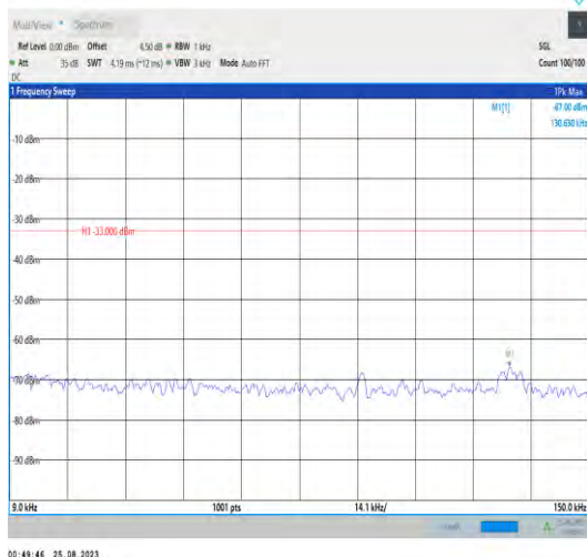
Band42_20MHz_QPSK_43190_1RB#0_0.009~0.15_0.00 9~0.15
