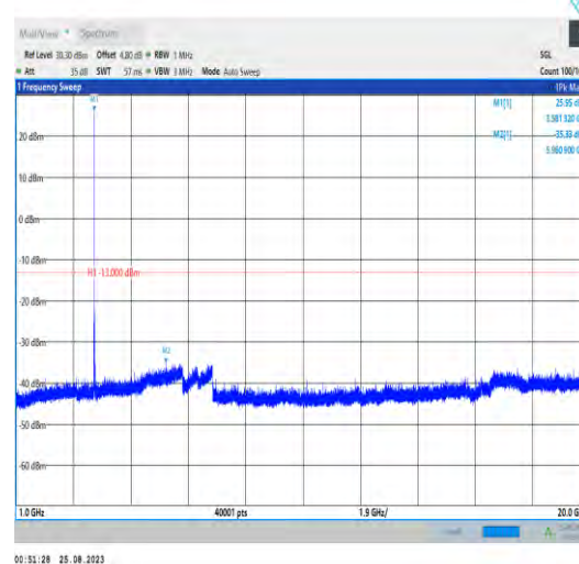
Band42_20MHz_QPSK_43490_1RB#0_1000~20000_1000~20000
