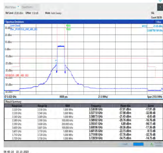
Band22_10MHz_QPSK_43540_50RB#0
