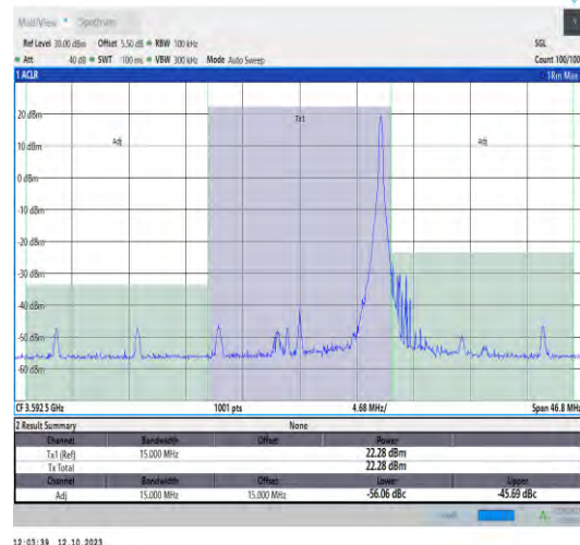
42(3550-3600)-15MHz-QPSK-43515-1RB#74-PASS
