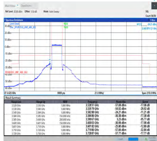
Band22_15MHz_QPSK_43515_75RB#0
