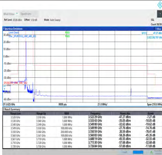
Band22_10MHz_QPSK_43140_1RB#0
