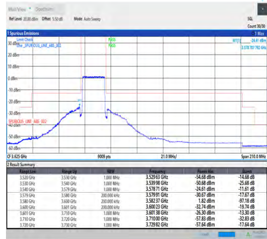
Band22_20MHz_QPSK_43490_100RB#0
