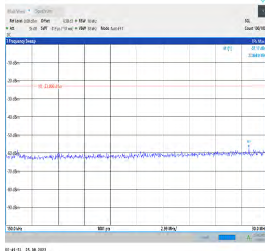
Band42_20MHz_QPSK_43190_1RB#0_0.15~30_0.15~30 30
