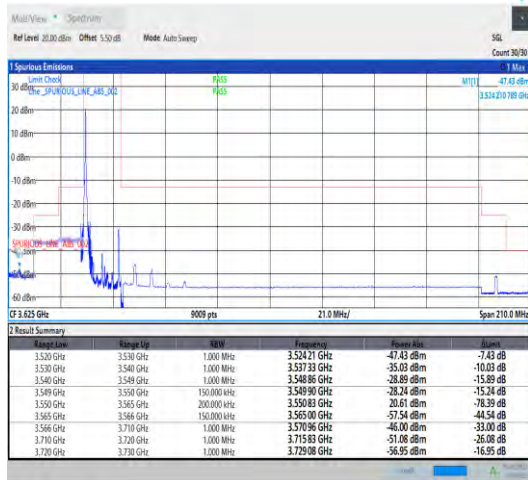
Band22_15MHz_QPSK_43165_1RB#0
