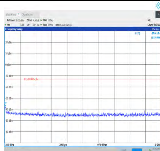
Band42_20MHz_QPSK_43340_1RB#0_20000~40000_20000~40000
