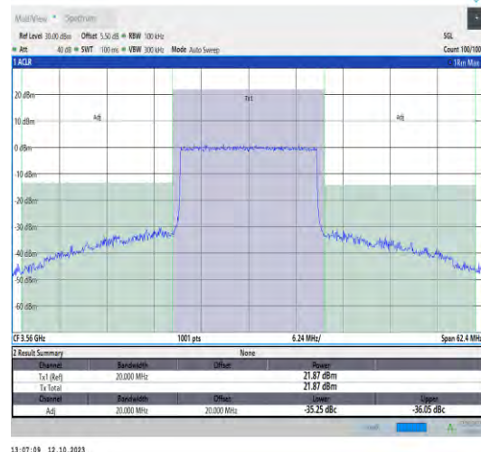
42(3550-3600)-20MHz-QPSK-43190-100RB#0-PASS
