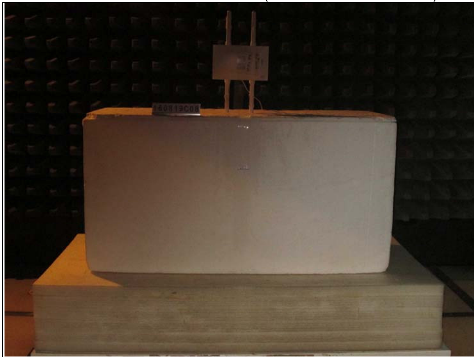
Radiated Emission Test above 1GHz (WLAN mode A & F & BT LE)
