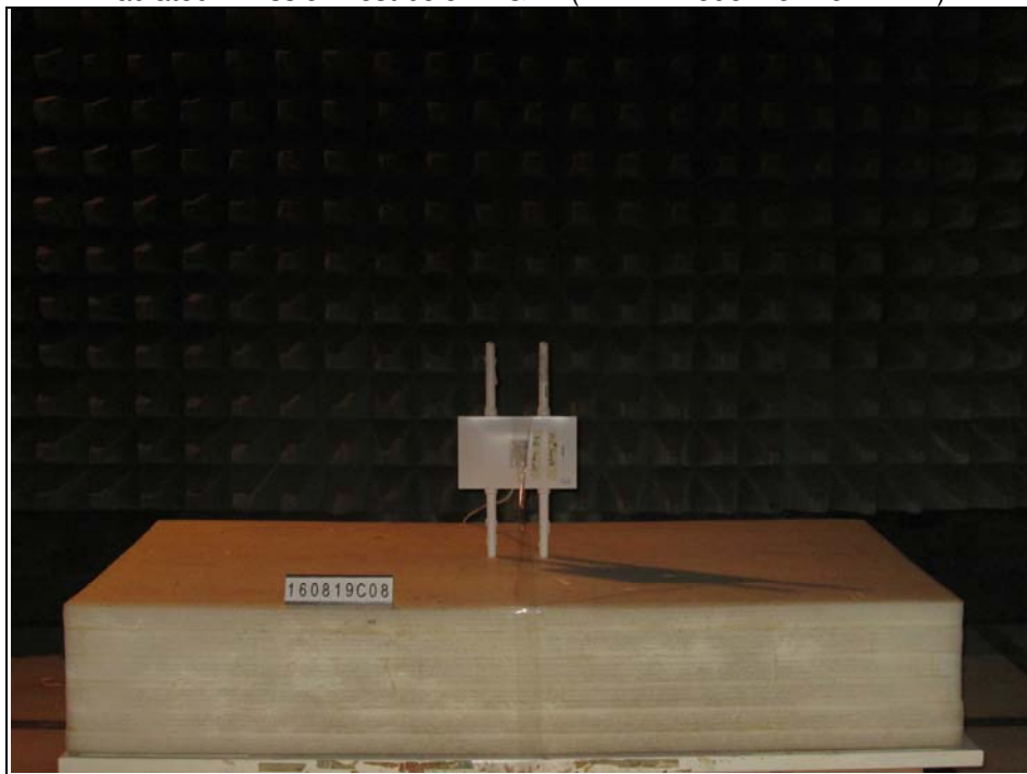
Radiated Emission Test below 1GHz (WLAN mode A & F & BT LE)
