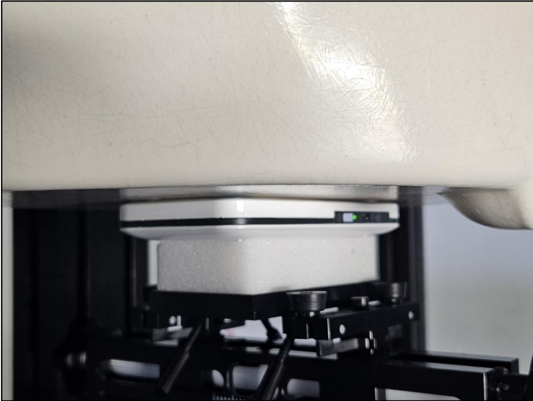
Photo 13: Test position bottom side with 0 mm distance with low-permittivity and low-loss foam front position
