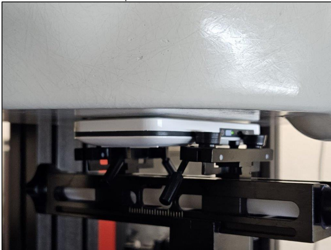
Photo 8: Test position back side with 0 mm distance
