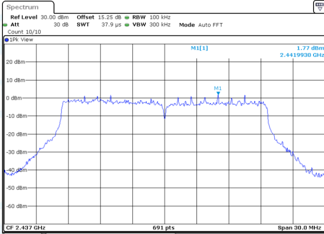
11AX20MIMO-Ant2-2437-0~Reference-PASS
