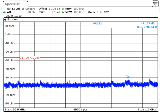
11B-CDD-Ant2-2412-0~Reference-PASS
