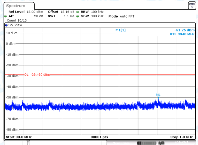
11AX20MIMO-Ant1-2437-0~Reference-PASS
