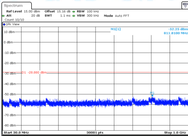
11N20MIMO-Ant1-2437-0~Reference-PASS
