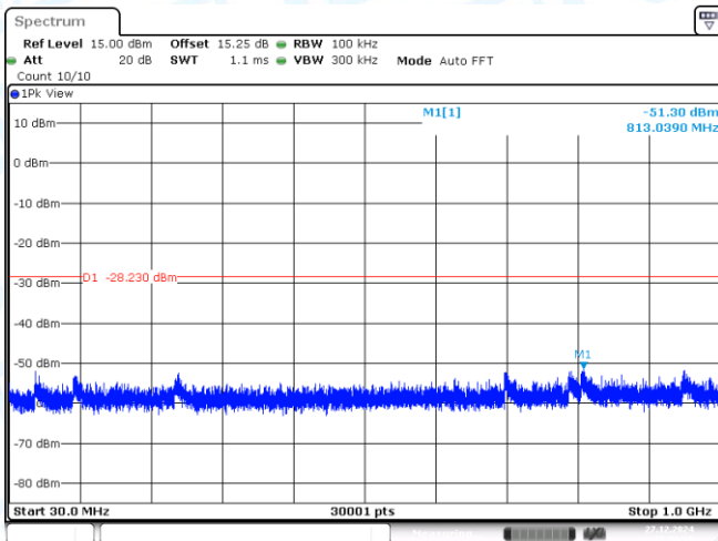
11AX20MIMO-Ant2-2437-0~Reference-PASS
