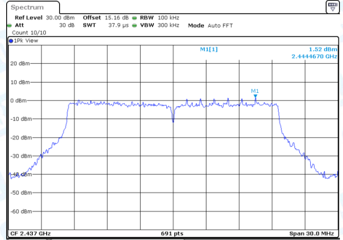
11AX20MIMO-Ant1-2437-0~Reference-PASS
