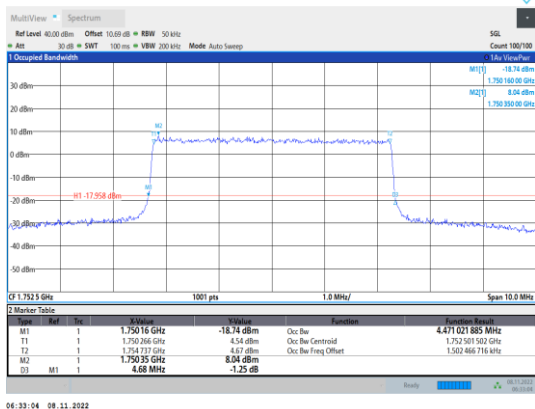
Band4-5MHz-QPSK-20375-25RB#0
