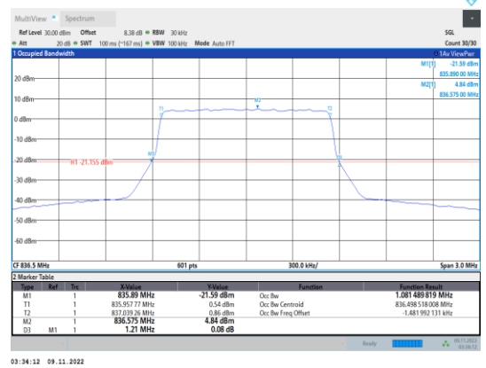
Band5-1.4MHz-16QAM-20525-6RB#0
