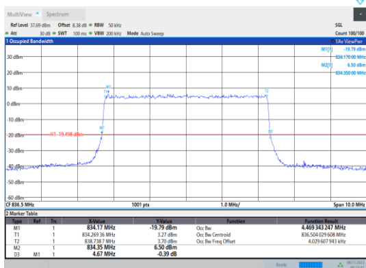
Band5-5MHz-QPSK-20525-25RB#0
