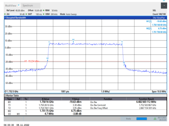
Band4-5MHz-16QAM-20375-25RB#0
