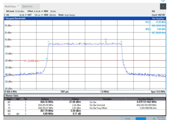
Band5-5MHz-16QAM-20525-25RB#0
