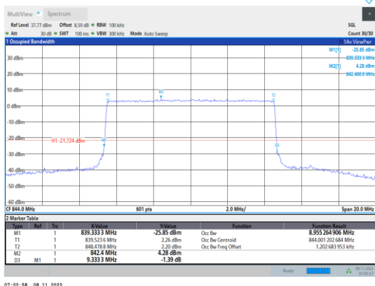
Band5-10MHz-16QAM-20600-50RB#0
