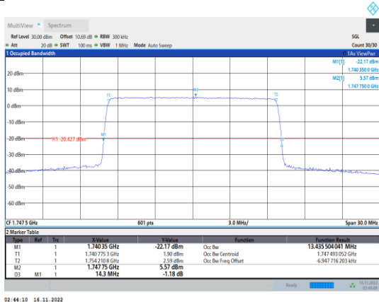
Band4-15MHz-64QAM-20325-75RB#0
