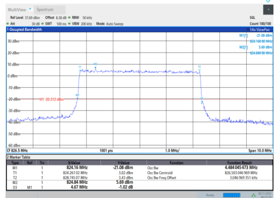
Band5-5MHz-16QAM-20425-25RB#0
