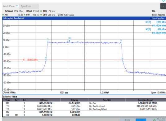
Band5-5MHz-QPSK-20625-25RB#0
