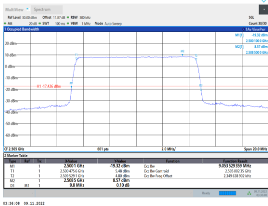
Band7-10MHz-16QAM-20800-50RB#0
