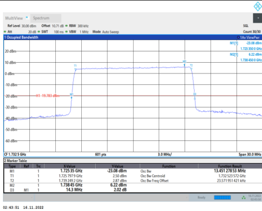
Band4-15MHz-64QAM-20175-75RB#0
