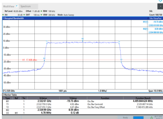
Band7-5MHz-QPSK-21100-25RB#0
