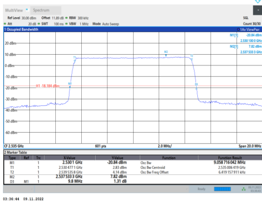
Band7-10MHz-16QAM-21100-50RB#0
