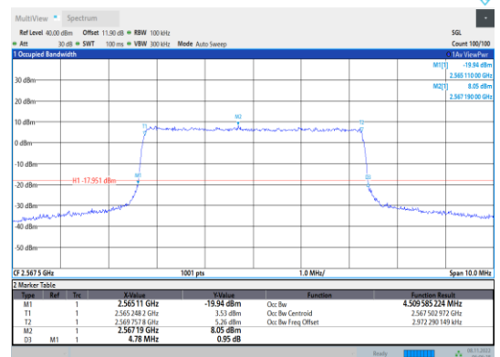
Band7-5MHz-16QAM-21425-25RB#0
