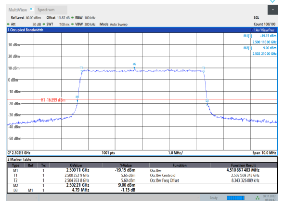
Band7-5MHz-16QAM-20775-25RB#0
