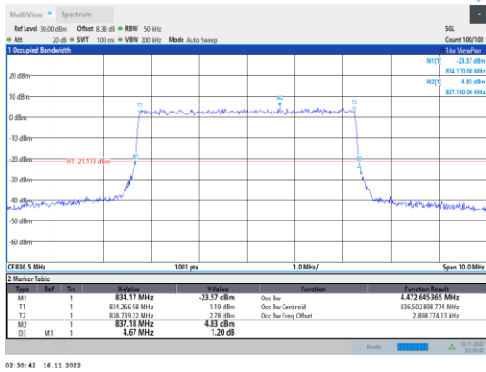
Band5-5MHz-64QAM-20525-25RB#0
