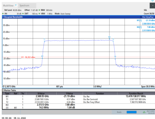
Band7-15MHz-QPSK-20825-75RB#0
