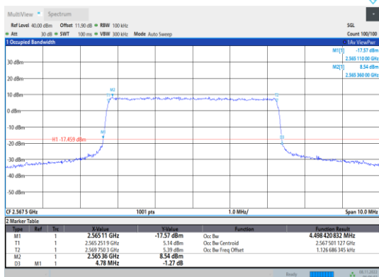
Band7-5MHz-QPSK-21425-25RB#0
