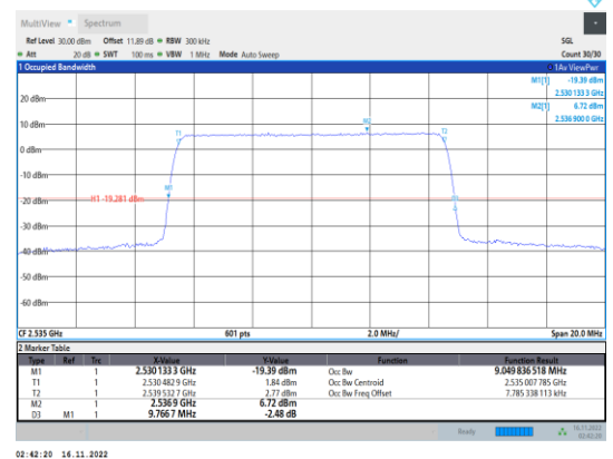
Band7-10MHz-64QAM-21100-50RB#0
