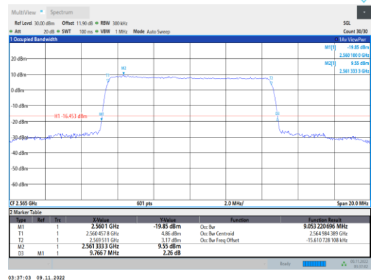
Band7-10MHz-QPSK-21400-50RB#0
