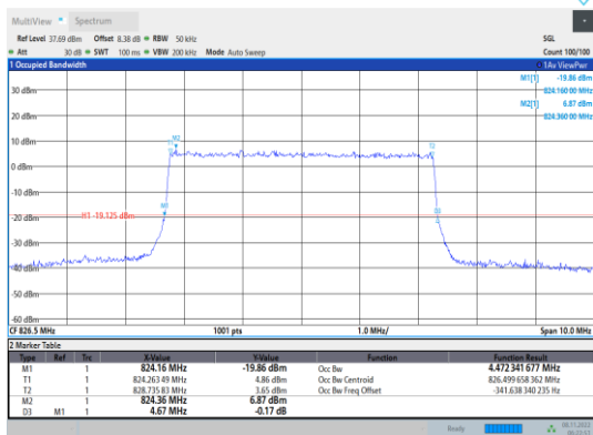
Band5-5MHz-QPSK-20425-25RB#0
