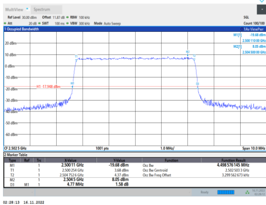
Band7-5MHz-64QAM-20775-25RB#0
