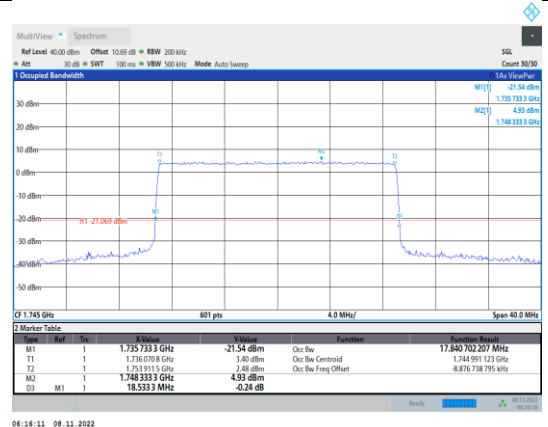
Band4-20MHz-QPSK-20300-100RB#0
