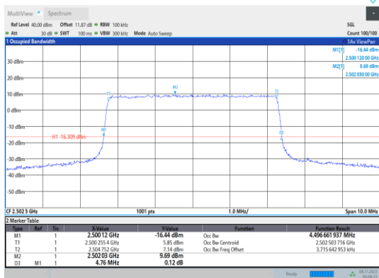
Band7-5MHz-QPSK-20775-25RB#0
