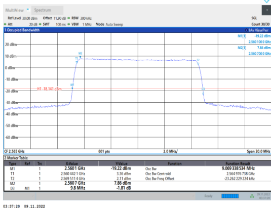
Band7-10MHz-16QAM-21400-50RB#0
