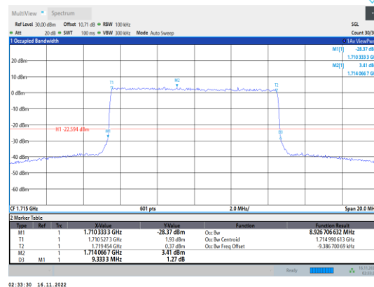
Band4-10MHz-64QAM-20000-50RB#0
