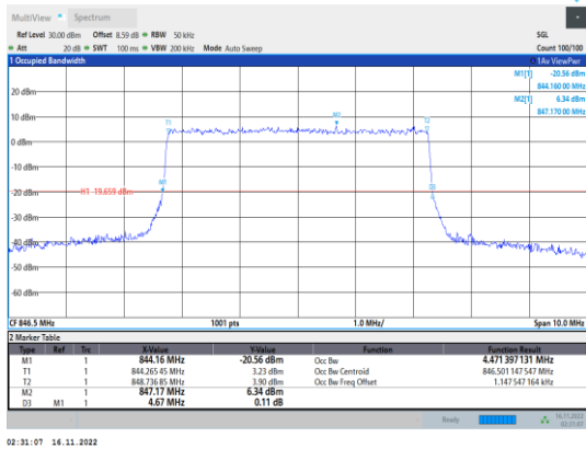
Band5-5MHz-64QAM-20625-25RB#0
