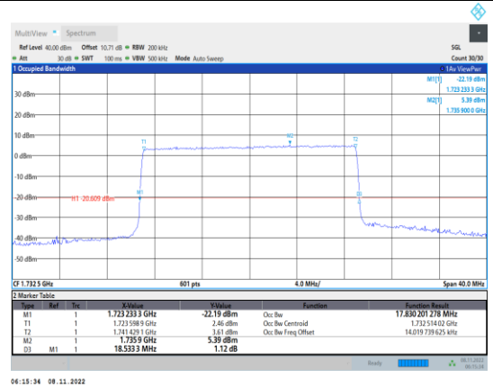
Band4-20MHz-QPSK-20175-100RB#0
