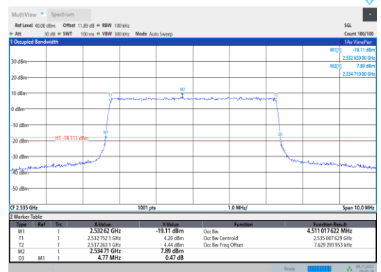
Band7-5MHz-16QAM-21100-25RB#0
