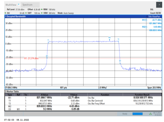
Band5-10MHz-QPSK-20550-50RB#0
