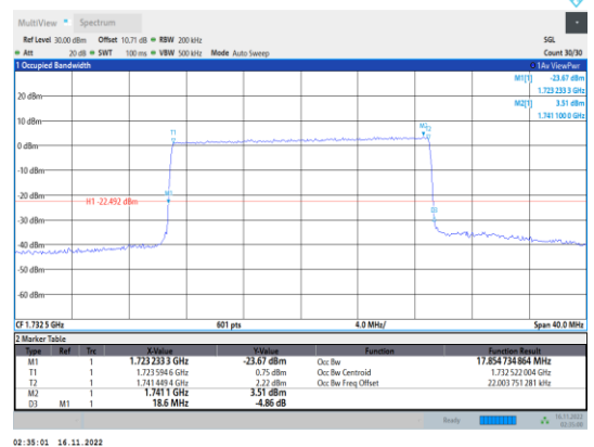
Band4-20MHz-64QAM-20175-100RB#0
