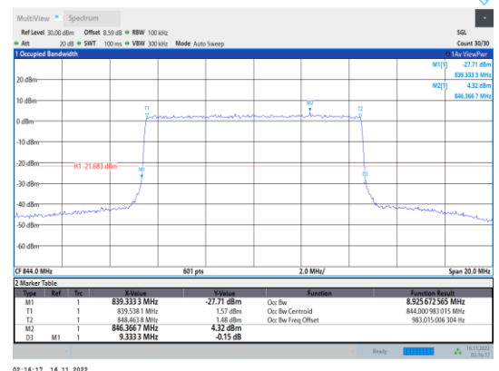
Band5-10MHz-64QAM-20600-50RB#0
