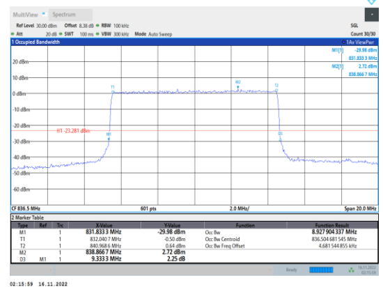
Band5-10MHz-64QAM-20525-50RB#0
