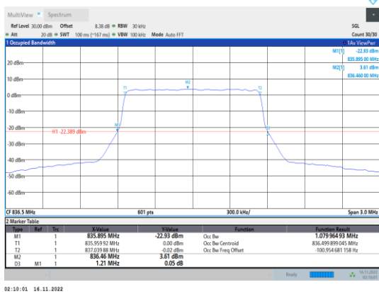
Band5-1.4MHz-64QAM-20525-6RB#0
