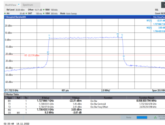
Band4-10MHz-64QAM-20175-50RB#0
