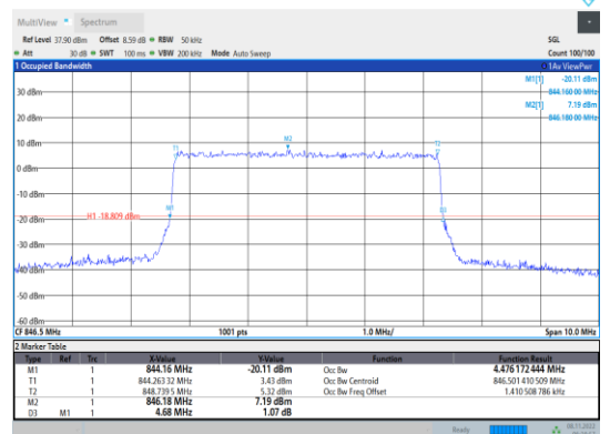
Band5-5MHz-16QAM-20625-25RB#0
