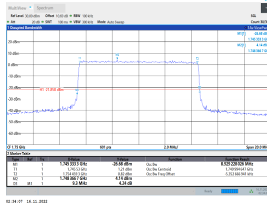
Band4-10MHz-64QAM-20350-50RB#0
