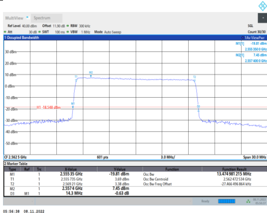
Band7-15MHz-QPSK-21375-75RB#0
