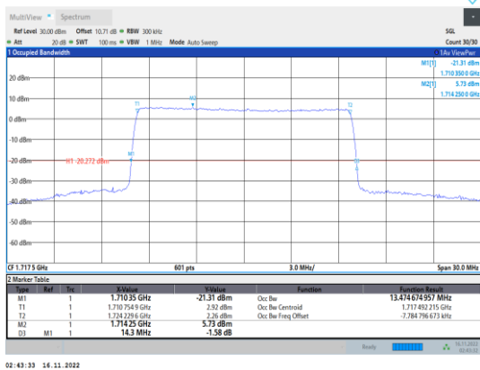
Band4-15MHz-64QAM-20025-75RB#0
