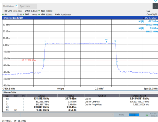
Band5-10MHz-16QAM-20525-50RB#0
