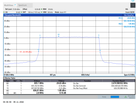
Band5-3MHz-QPSK-20525-15RB#0
