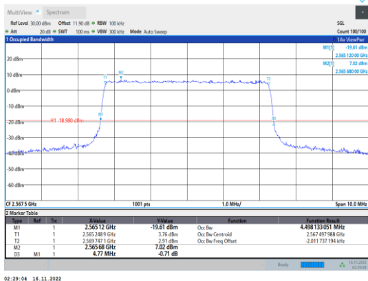
Band7-5MHz-64QAM-21425-25RB#0
