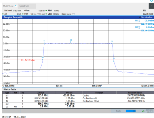
Band5-3MHz-16QAM-20525-15RB#0
