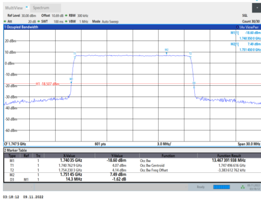
Band4-15MHz-QPSK-20325-75RB#0
