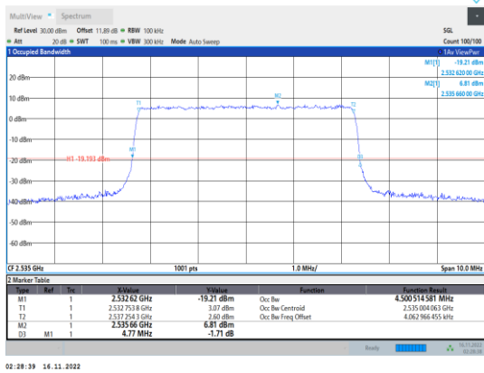
Band7-5MHz-64QAM-21100-25RB#0
