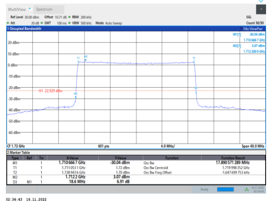
Band4-20MHz-64QAM-20050-100RB#0
