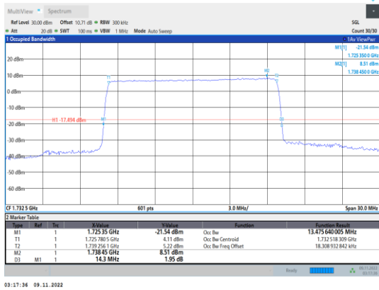
Band4-15MHz-QPSK-20175-75RB#0
