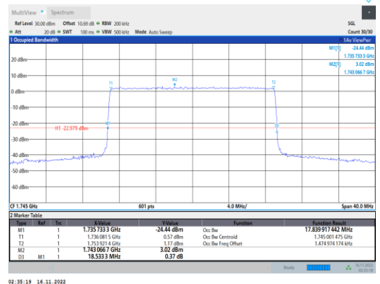
Band4-20MHz-64QAM-20300-100RB#0
