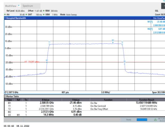
Band7-15MHz-16QAM-20825-75RB#0
