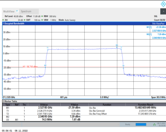
Band7-15MHz-QPSK-21100-75RB#0
