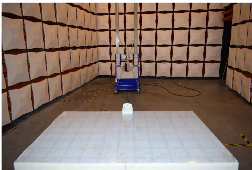
TX 30MHz-1GHz
