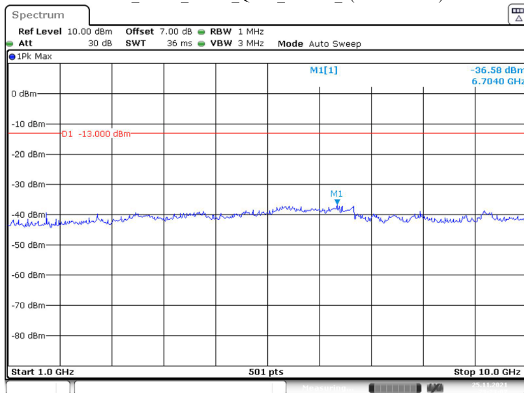
Band 5_3 MHz_Middle_QPSK_RB15#0_2(1GHz-10GHz)
