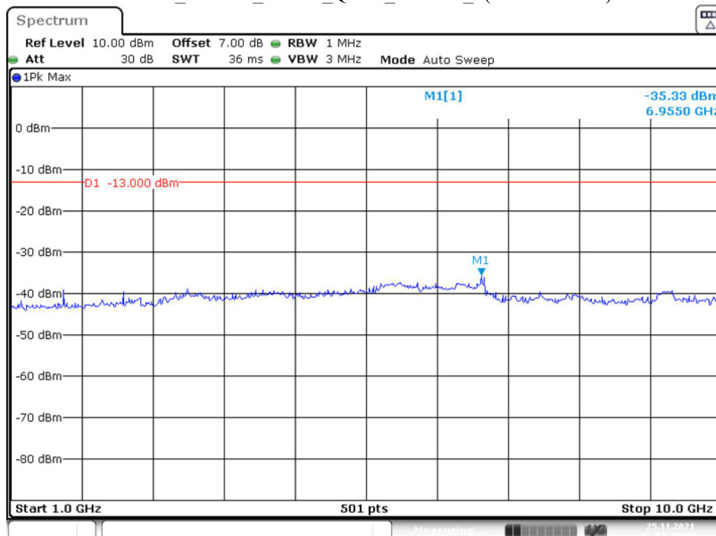
Band 5_10 MHz_Middle_QPSK_RB50#0_2(1GHz-10GHz)
