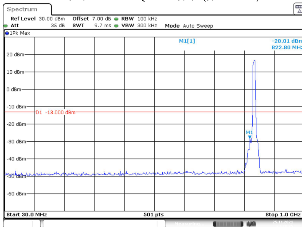
Band 5_10 MHz_Middle_QPSK_RB50#0_1(30MHz-1GHz)
