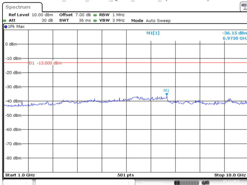
Band 5_5 MHz_Middle_QPSK_RB25#0_2(1GHz-10GHz)
