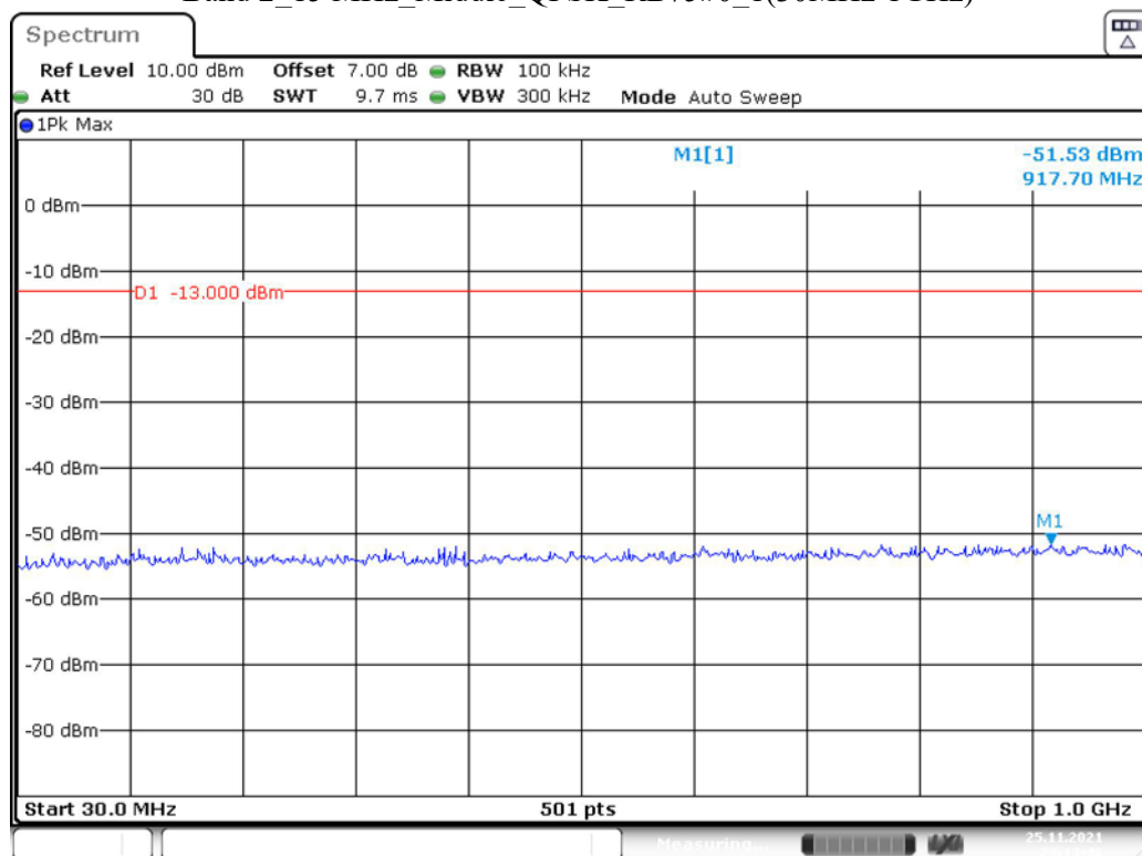
Band 2_15 MHz_Middle_QPSK_RB75#0_1(30MHz-1GHz)
