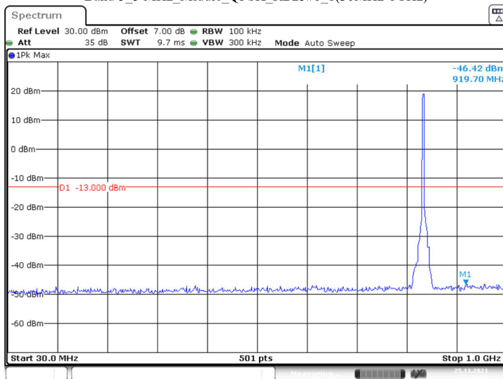
Band 5_5 MHz_Middle_QPSK_RB25#0_1(30MHz-1GHz)
