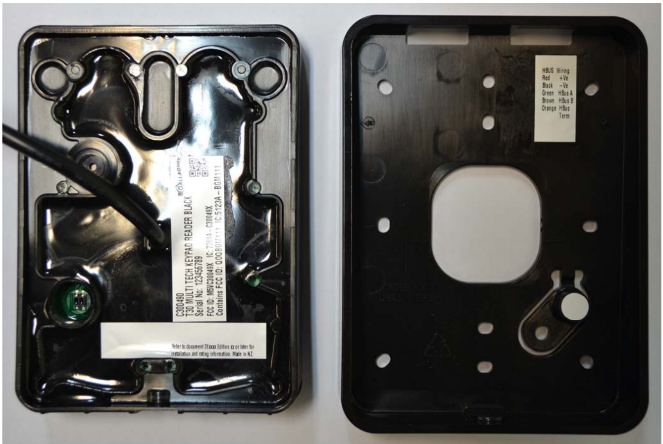
T30 Multi Tech & Mifare - Potted Assembly and Bezel
