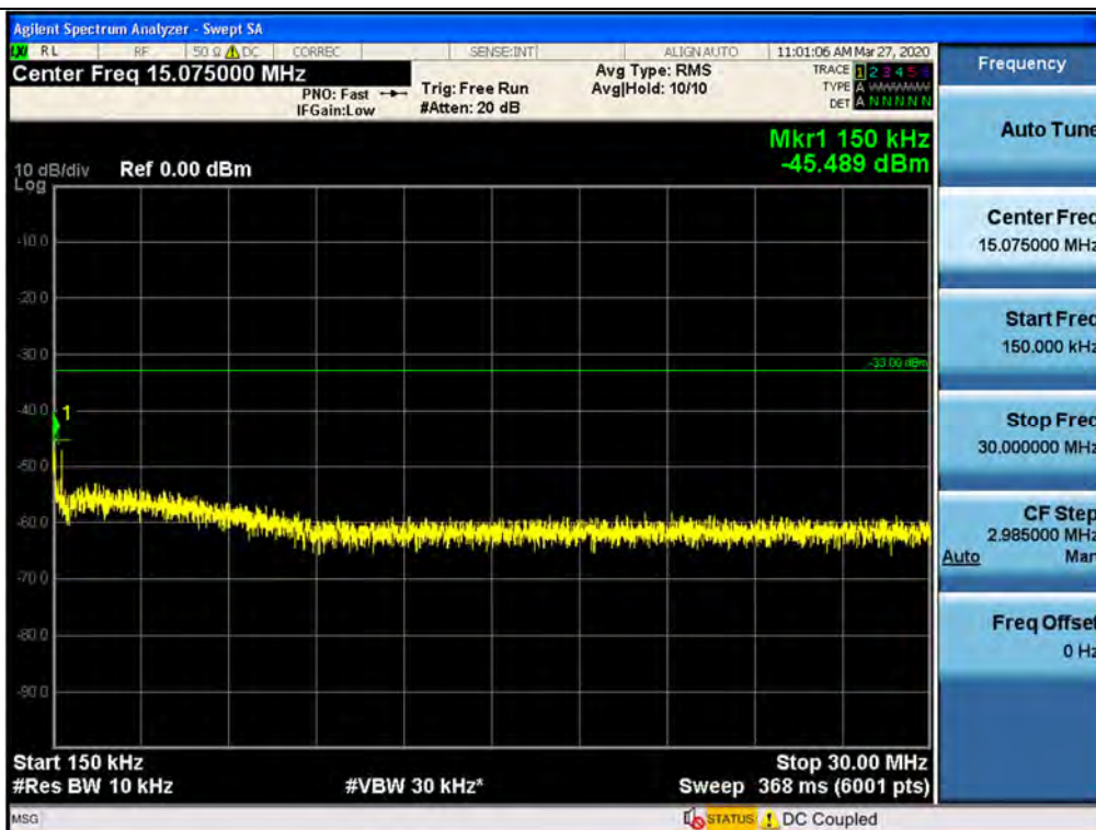
Spurious / AWS / Downlink / LTE 10 MHz / Low / 150 kHz ~ 30 MHz
