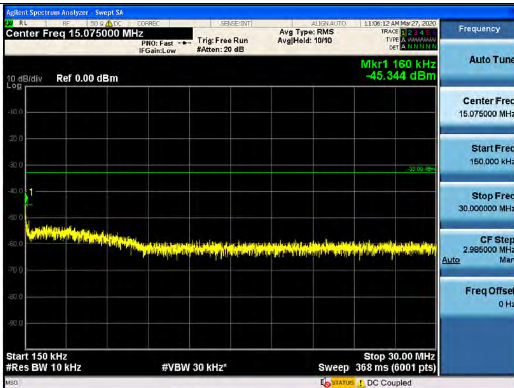
Spurious / AWS / Downlink / LTE 10 MHz / Middle / 150 kHz ~ 30 MHz
