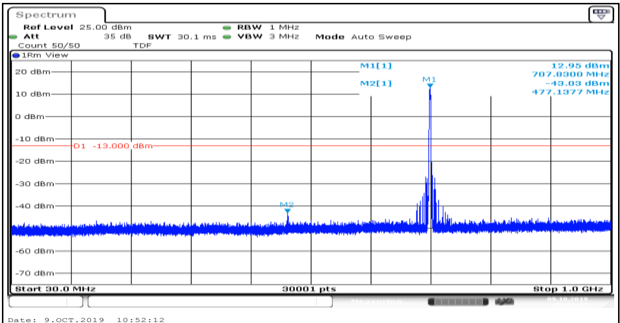
Band12_1.4MHz_QPSK_23095_6
