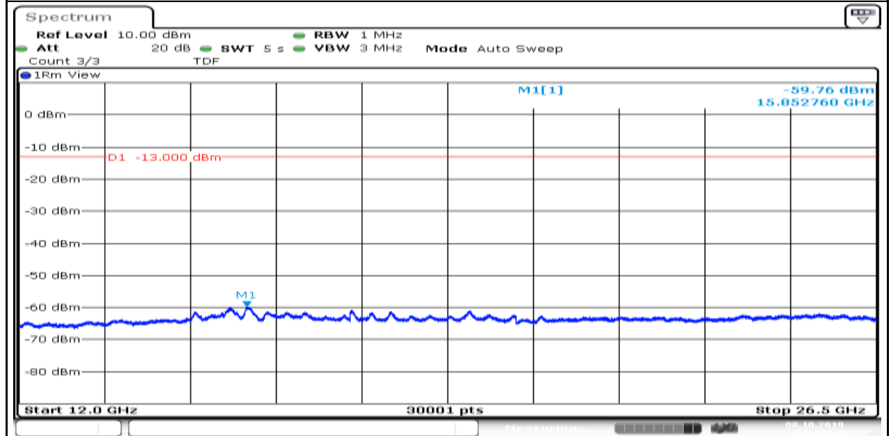
Band5_1.4MHz_QPSK_20643_1
