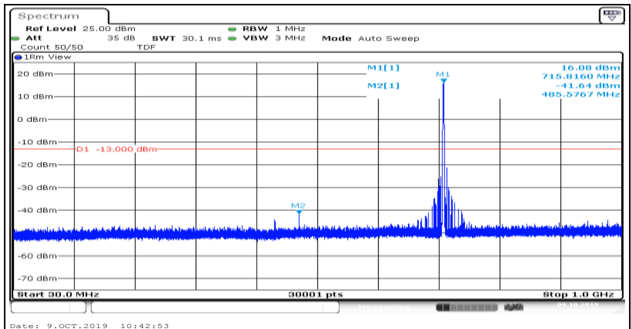
Band12_1.4MHz_16QAM_23173_1
