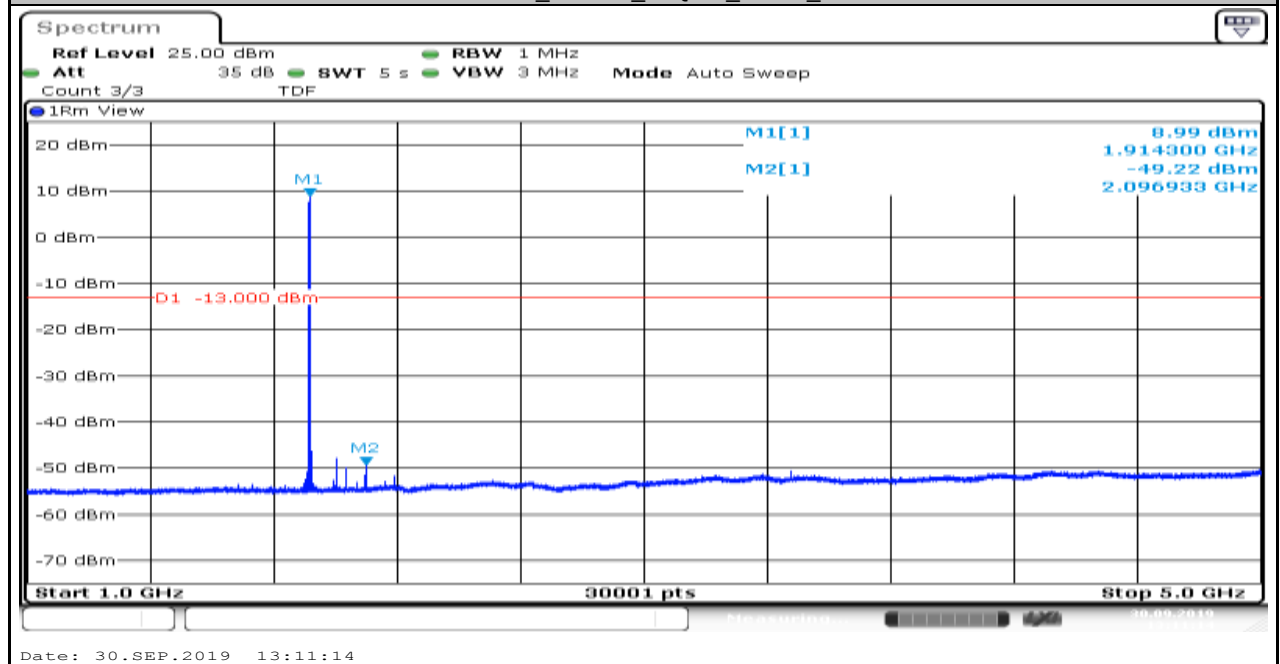
Band25_1.4MHz_16QAM_26683_6
