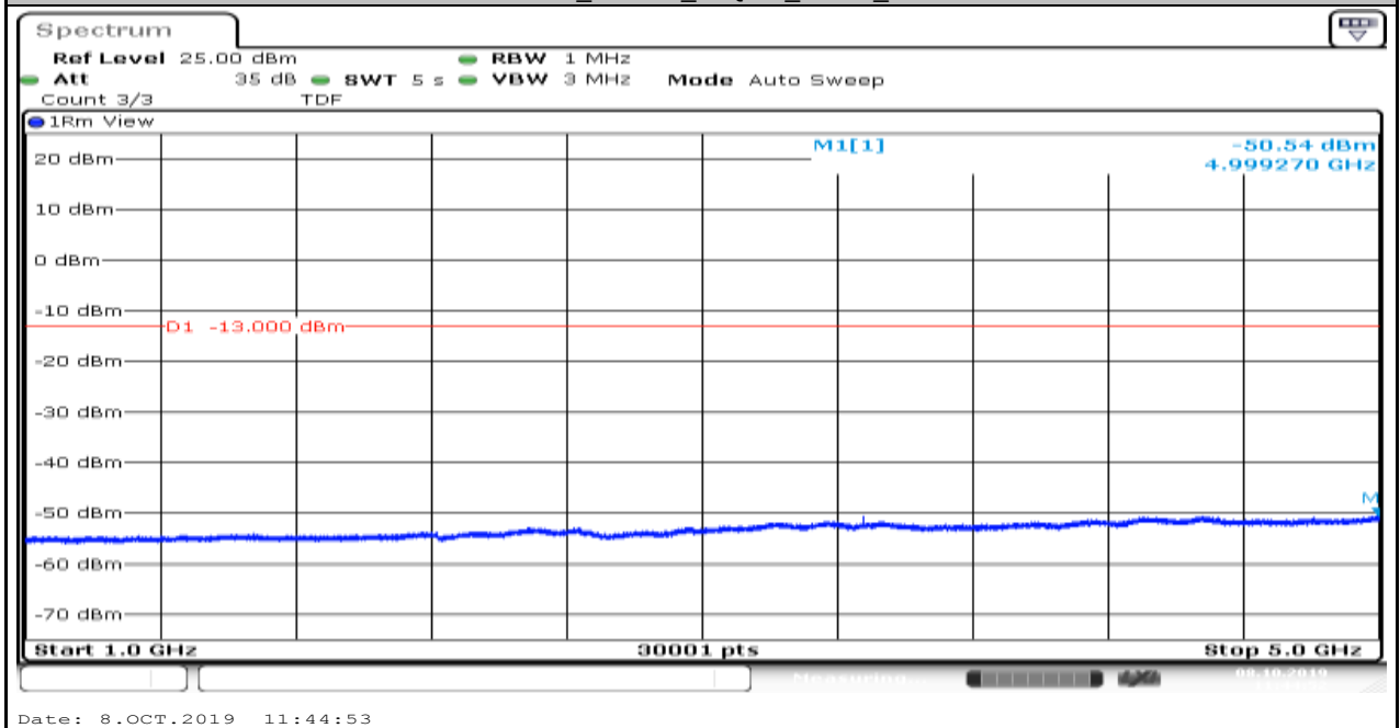
Band5_1.4MHz_16QAM_20525_1
