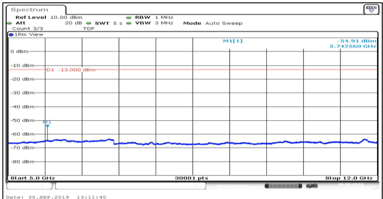
Band25_1.4MHz_16QAM_26683_6
