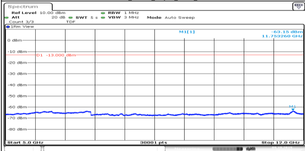
Band12_1.4MHz_16QAM_23095_1
