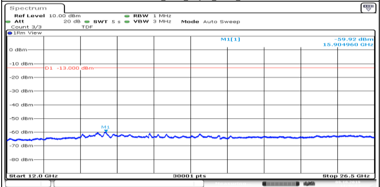
Band13_5MHz_16QAM_23255_1
