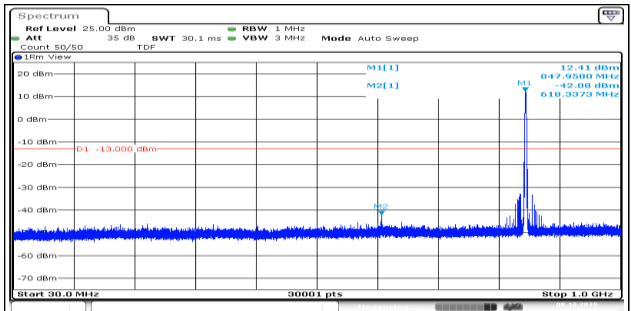
Band5_1.4MHz_QPSK_20643_1
