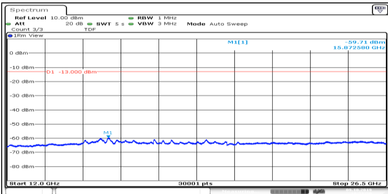
Band12_1.4MHz_16QAM_23095_1
