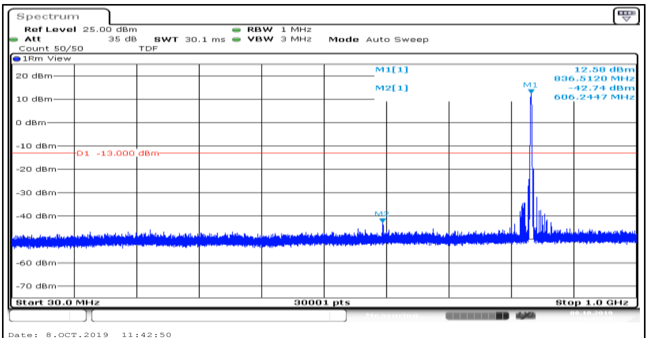
Band5_1.4MHz_QPSK_20525_6
