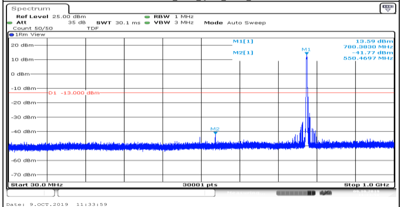
Band13_5MHz_QPSK_23255_1
