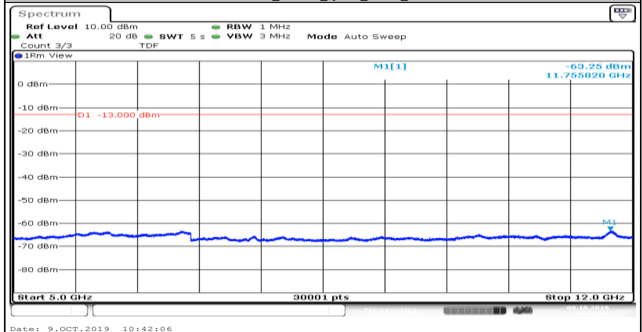
Band12_1.4MHz_16QAM_23017_6
