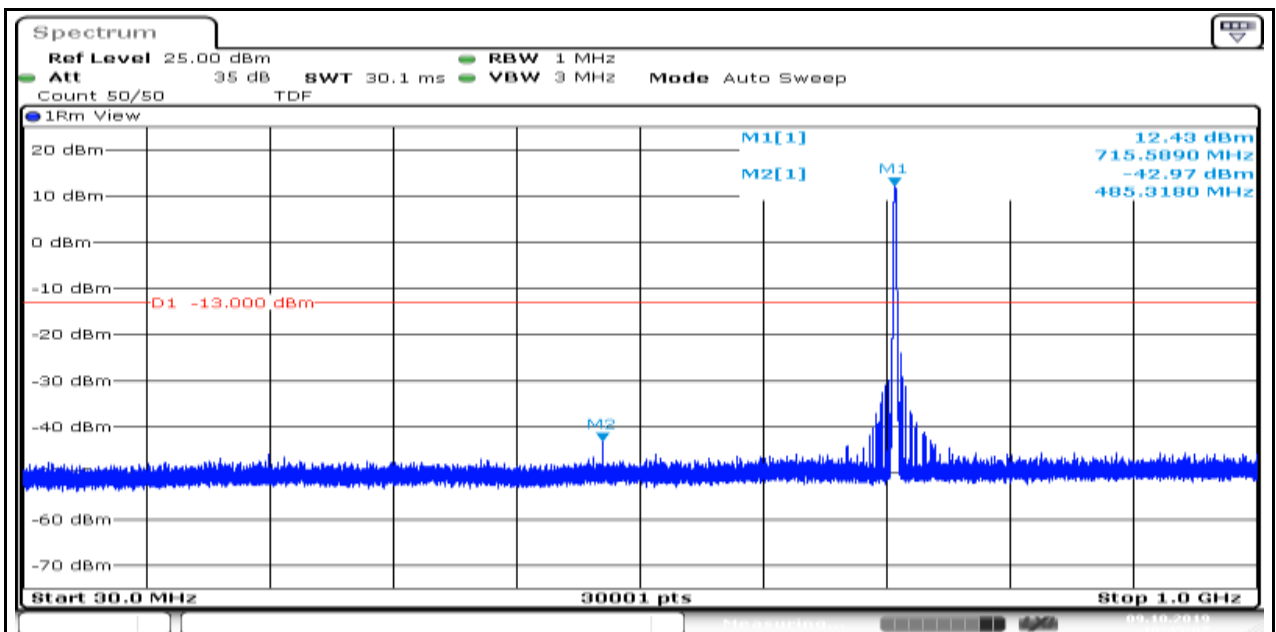
Band12_1.4MHz_QPSK_23173_1
