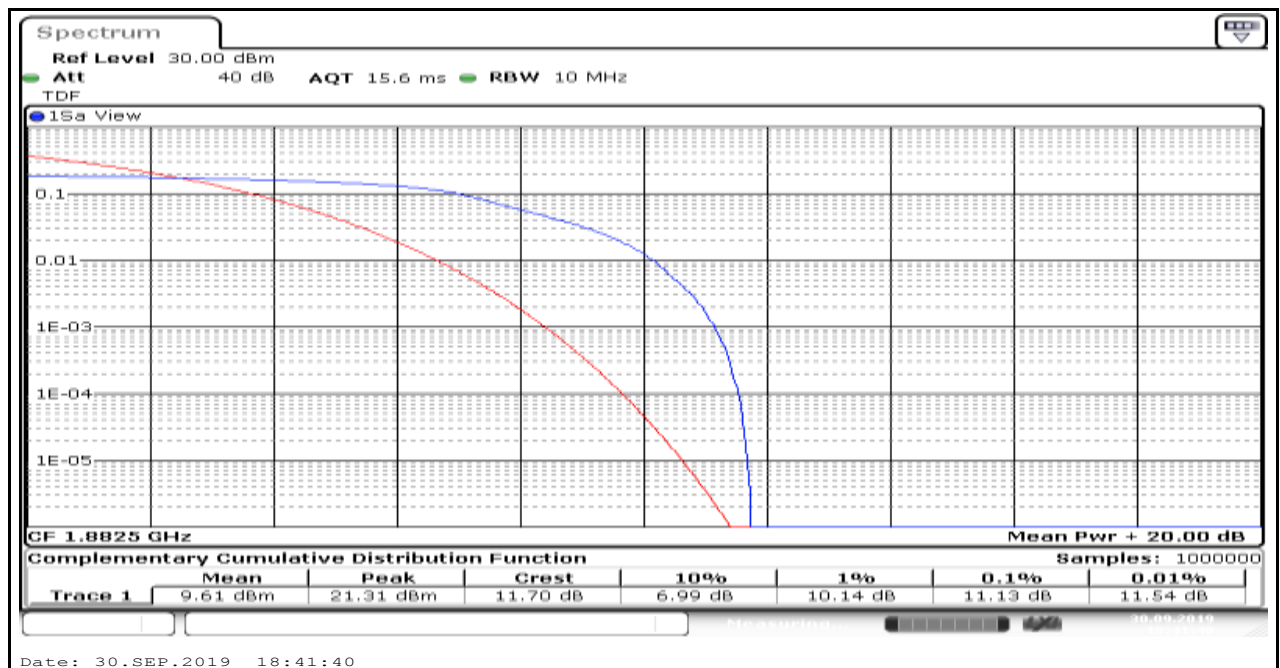
Band25_10MHz_16QAM_26365_6
