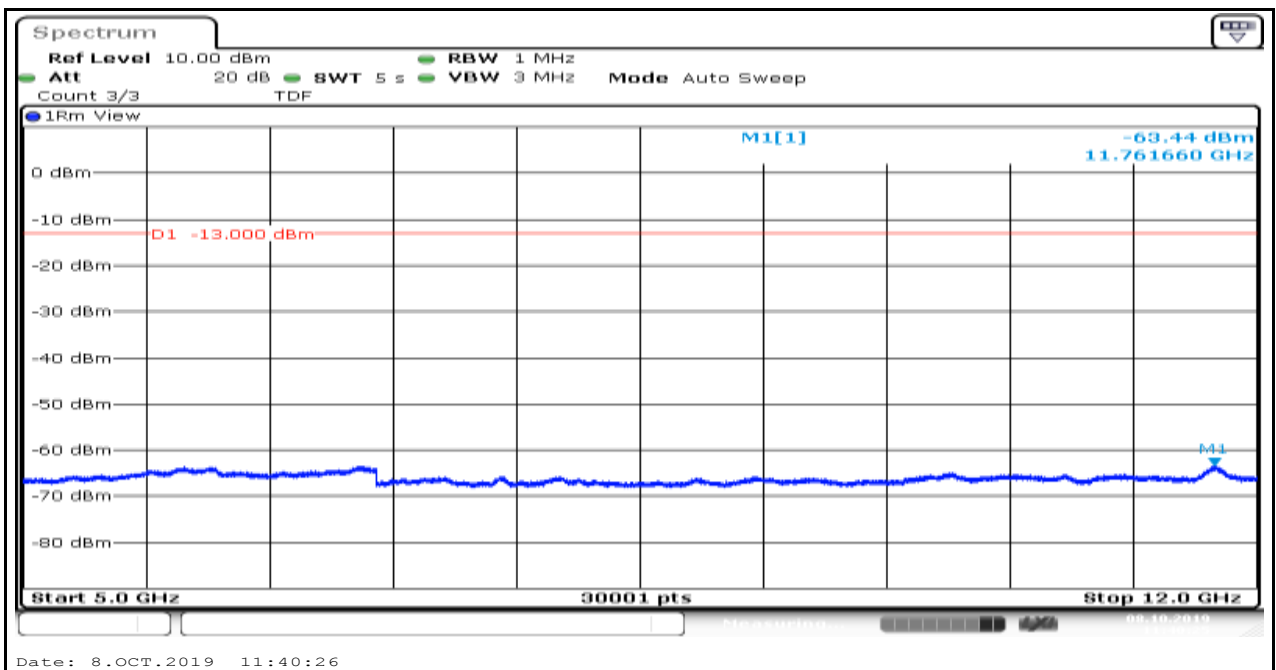
Band5_1.4MHz_QPSK_20525_1
