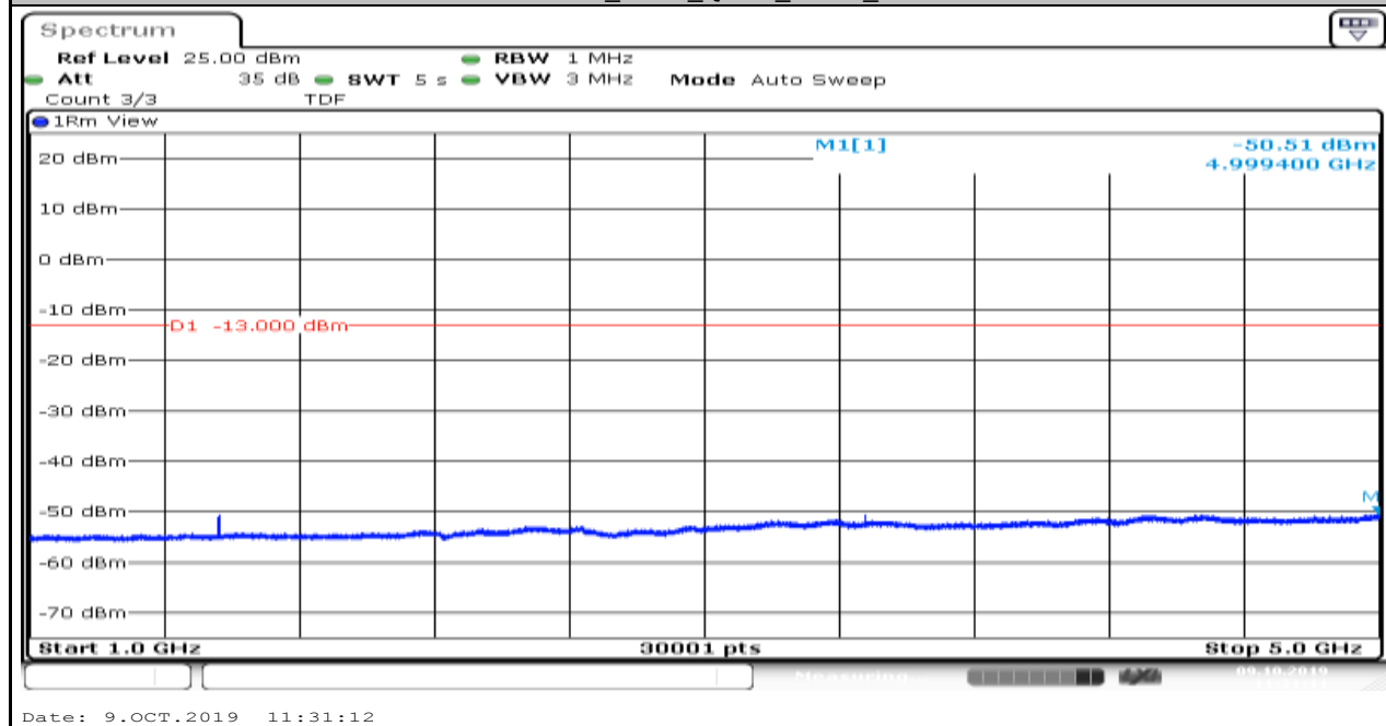
Band13_5MHz_QPSK_23230_1
