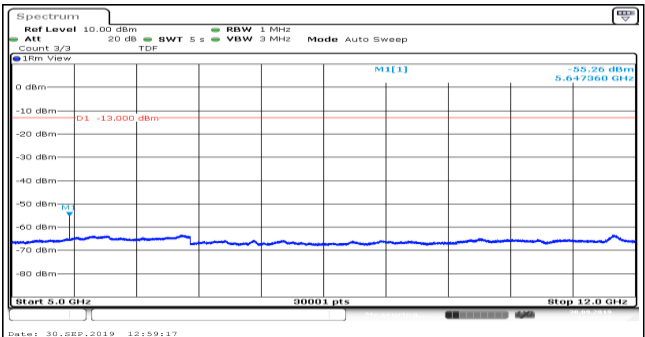
Band25_1.4MHz_QPSK_26365_6
