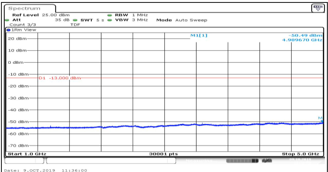
Band13_5MHz_16QAM_23230_6
