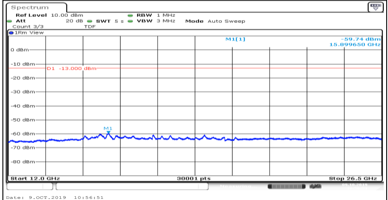
Band12_1.4MHz_QPSK_23017_1
