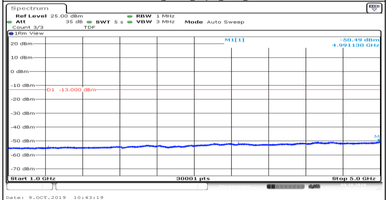
Band12_1.4MHz_16QAM_23173_1
