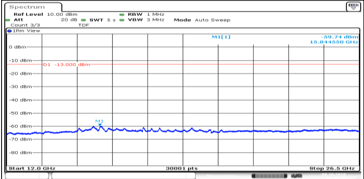
Band5_1.4MHz_16QAM_20525_6
