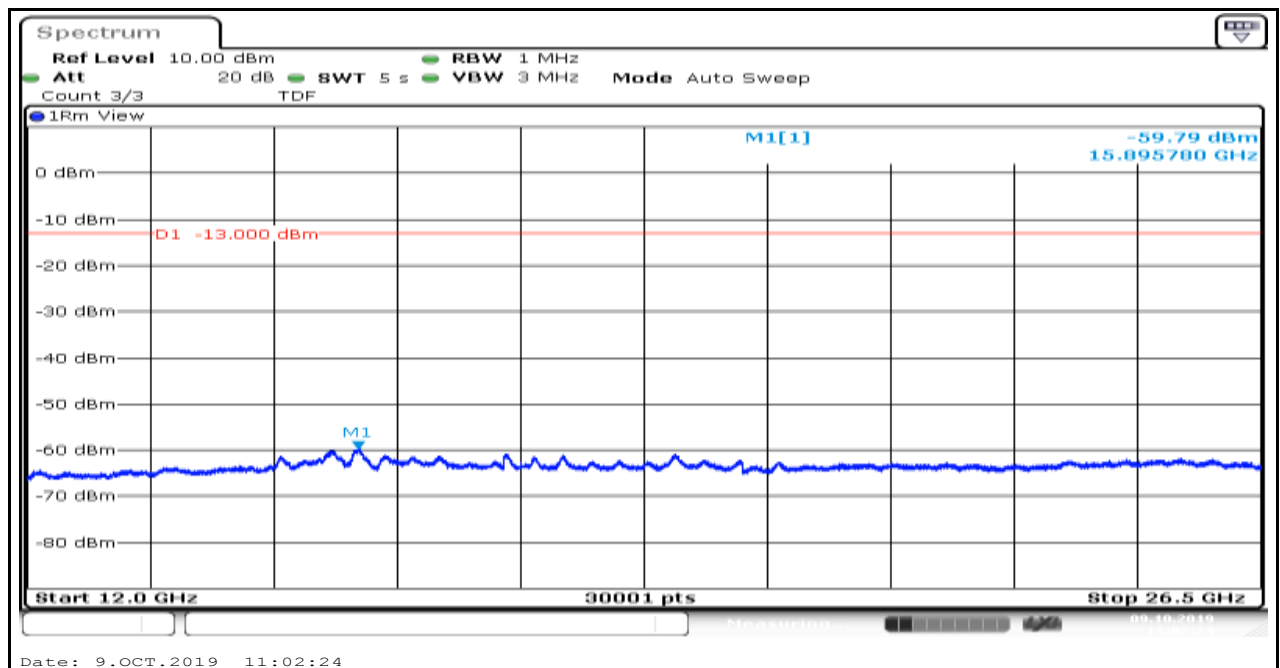
Band12_1.4MHz_16QAM_23017_1
