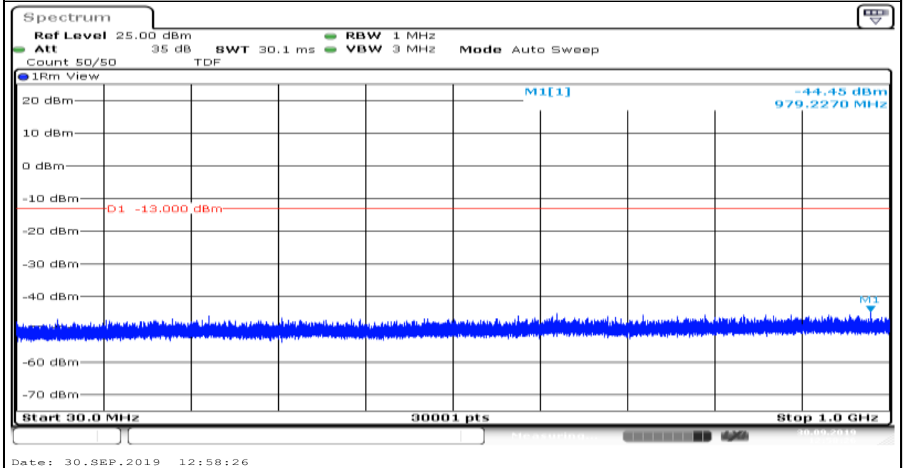
Band25_1.4MHz_QPSK_26683_1
