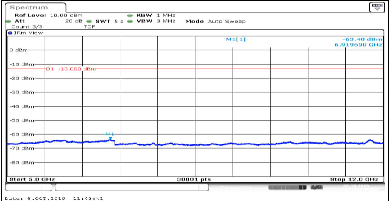
Band5_1.4MHz_QPSK_20643_6
