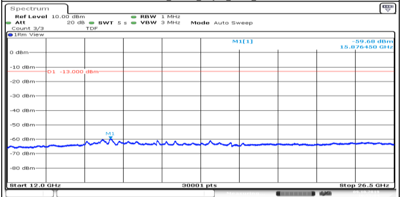
Band12_1.4MHz_16QAM_23095_6
