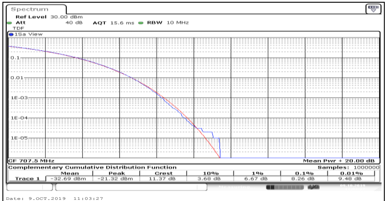
Band12_3MHz_QPSK_23095_6
