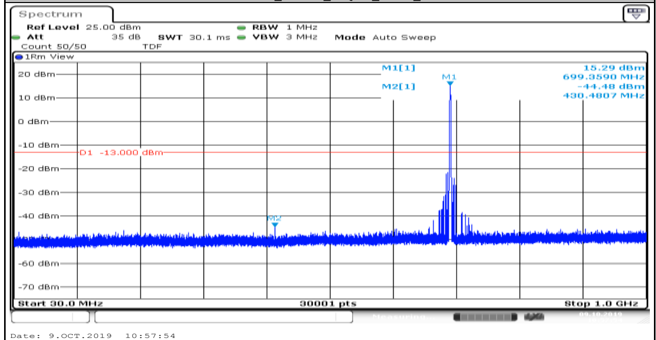
Band12_1.4MHz_16QAM_23017_1
