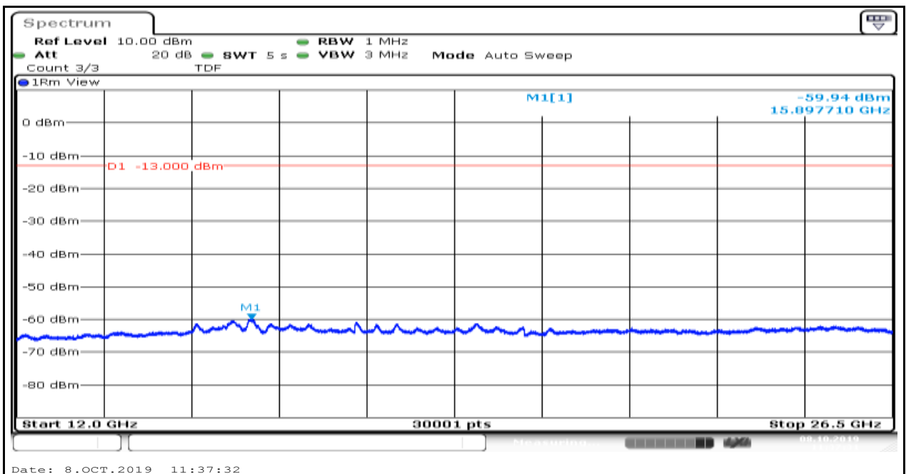
Band5_1.4MHz_QPSK_20643_6
