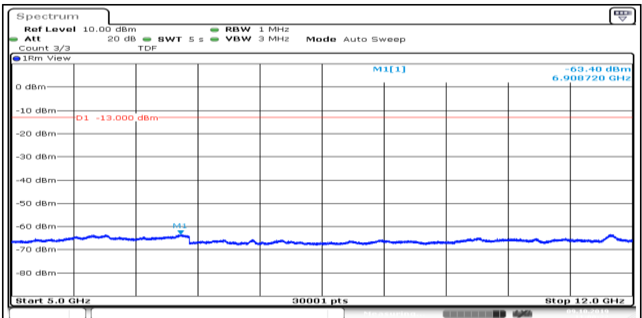
Band12_1.4MHz_QPSK_23017_6
