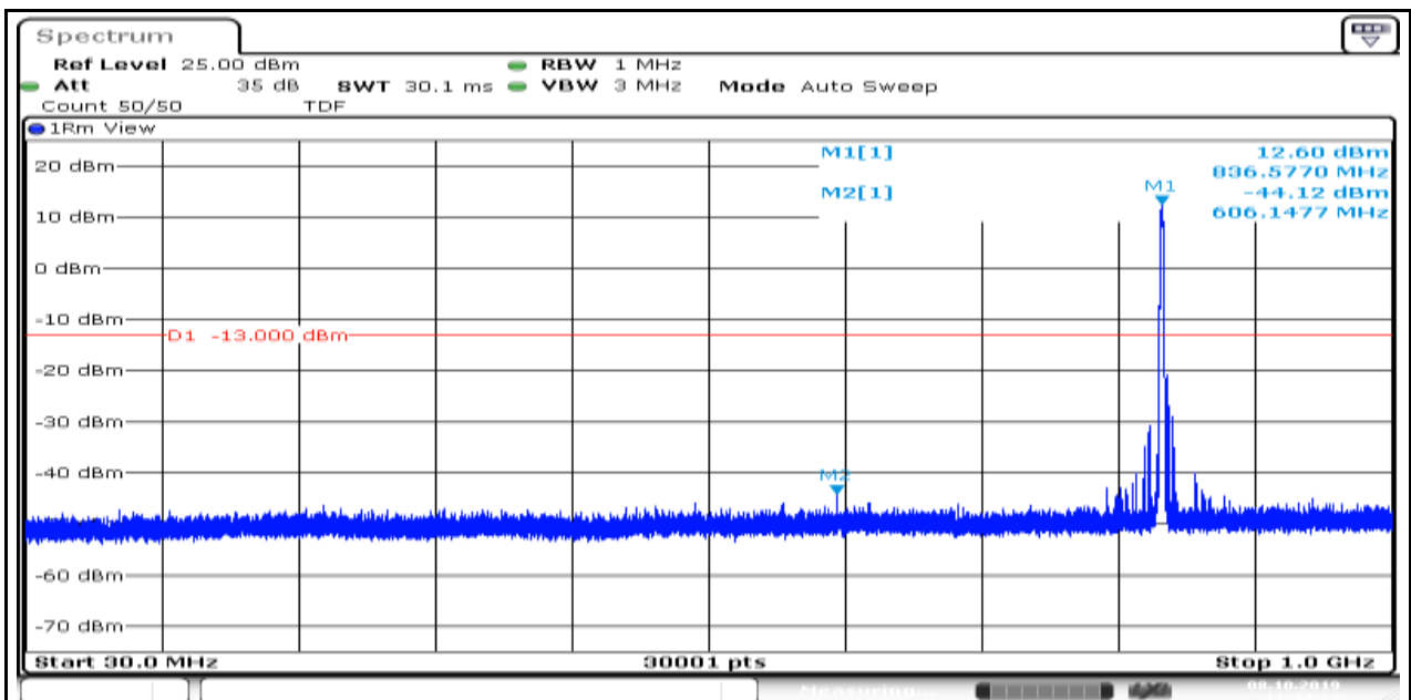
Band5_1.4MHz_16QAM_20525_6
