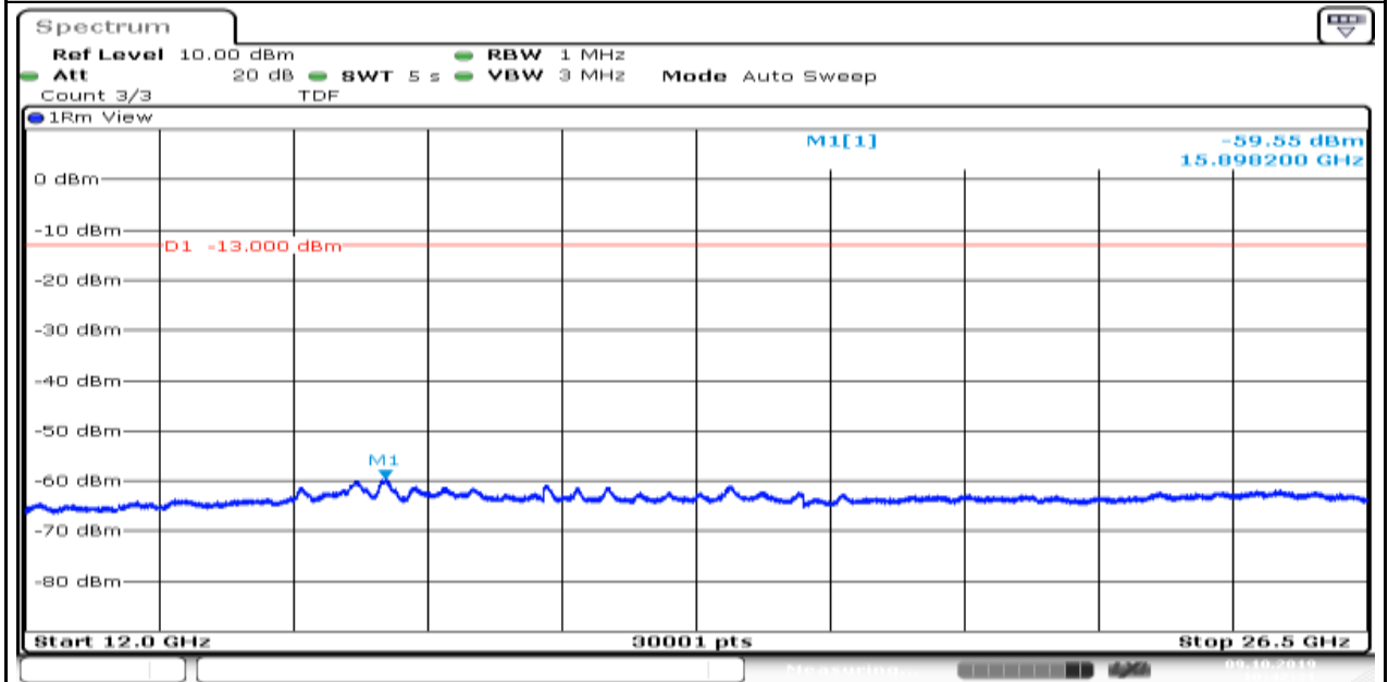
Band12_1.4MHz_QPSK_23173_1
