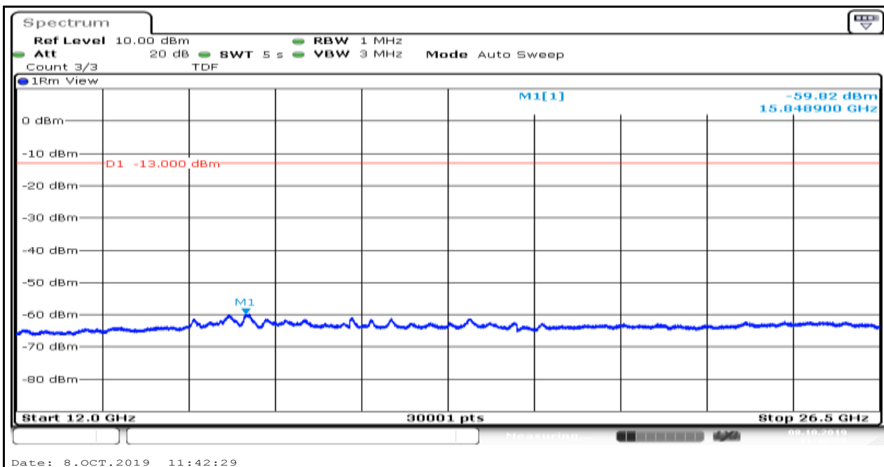
Band5_1.4MHz_16QAM_20525_1
