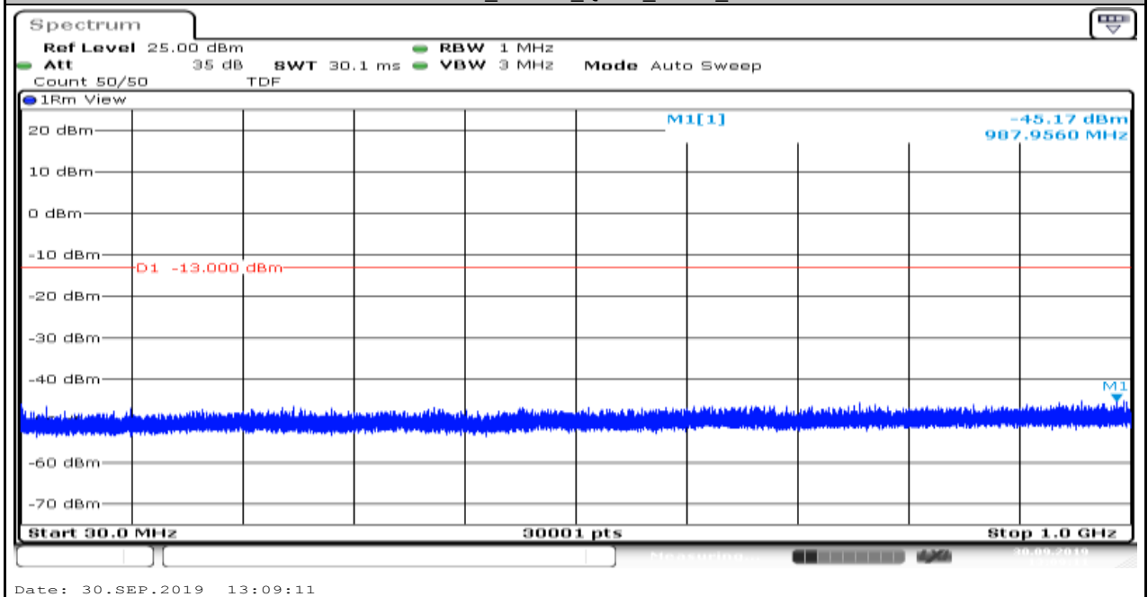
Band25_1.4MHz_QPSK_26683_1
