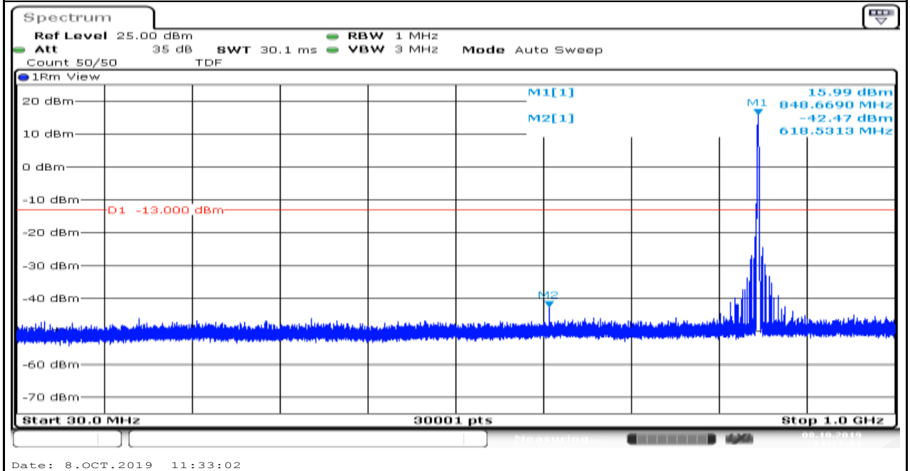
Band5_1.4MHz_QPSK_20643_6
