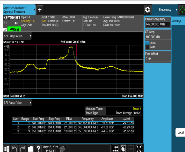
Band5-1.4MHz-QPSK-20643-1RB#5
