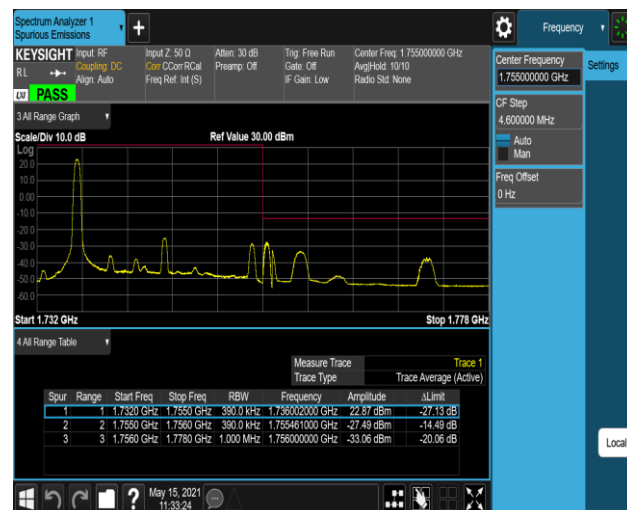
Band4-20MHz-16QAM-20300-100RB#0
