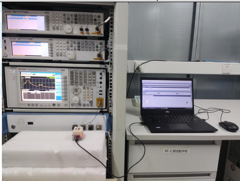
Conducted RF Test Setup
