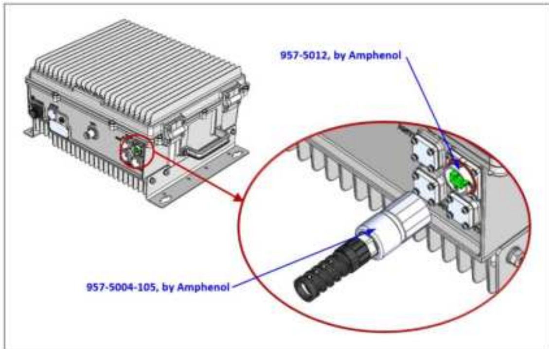
Figure 4.10 –Optical Connector
