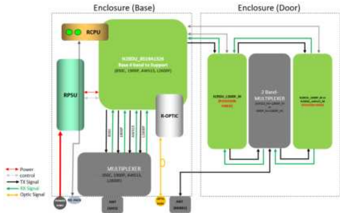
Figure 3.2 – N2ROU Block Diagram (4 bands(SISO) + 2 bands(MIMO))
