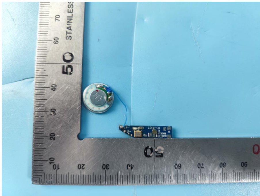
INTERNAL PHOTO OF SAMPLE PCB(R)
