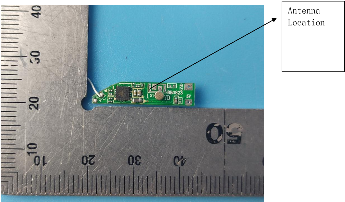
INTERNAL PHOTO OF SAMPLE PCB(L)
