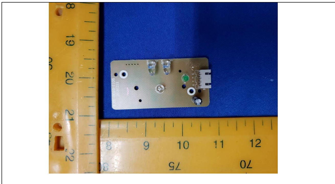
Details of: PCB for charging base
