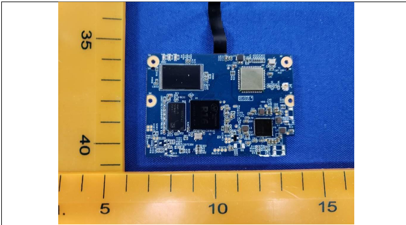
Details of: Camera PCB view
