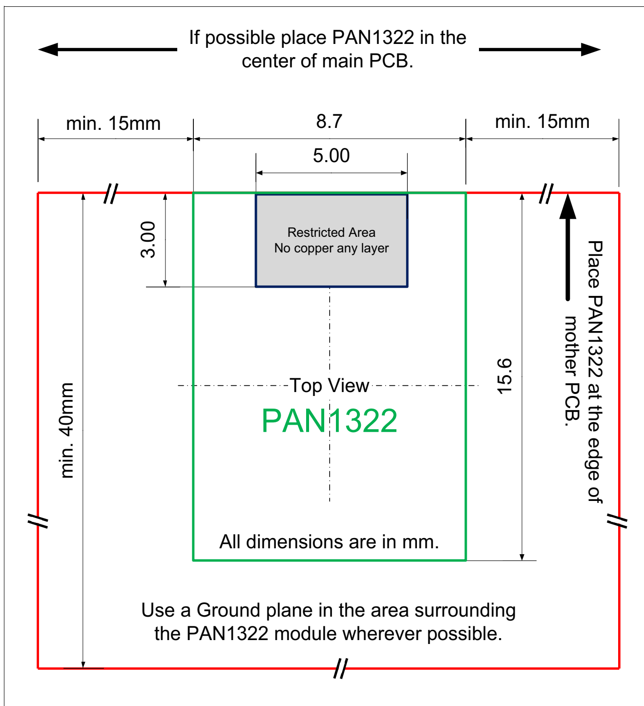
Figure 14 Cutout Drawing
