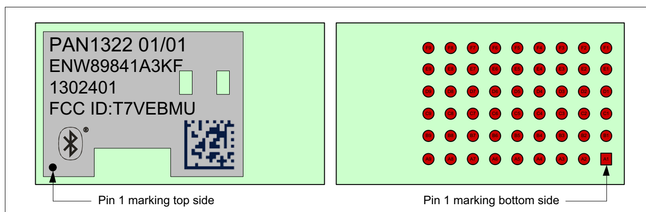
Figure 15 Pin Marking
