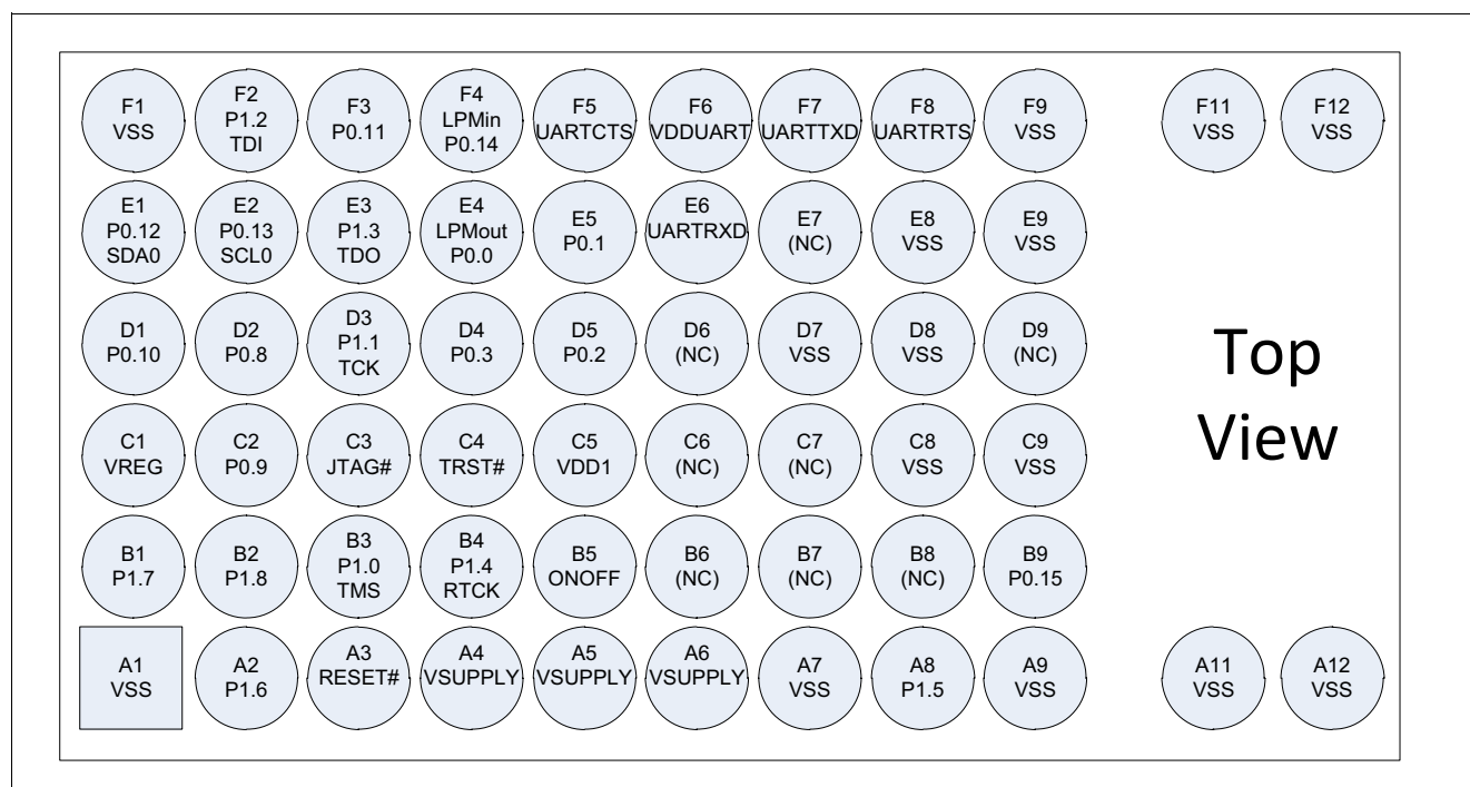
Figure 2 Pin Configuration for PAN1322-SPP in Top View (footprint)
