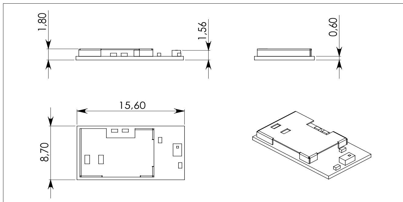
Figure 7 Production Package
