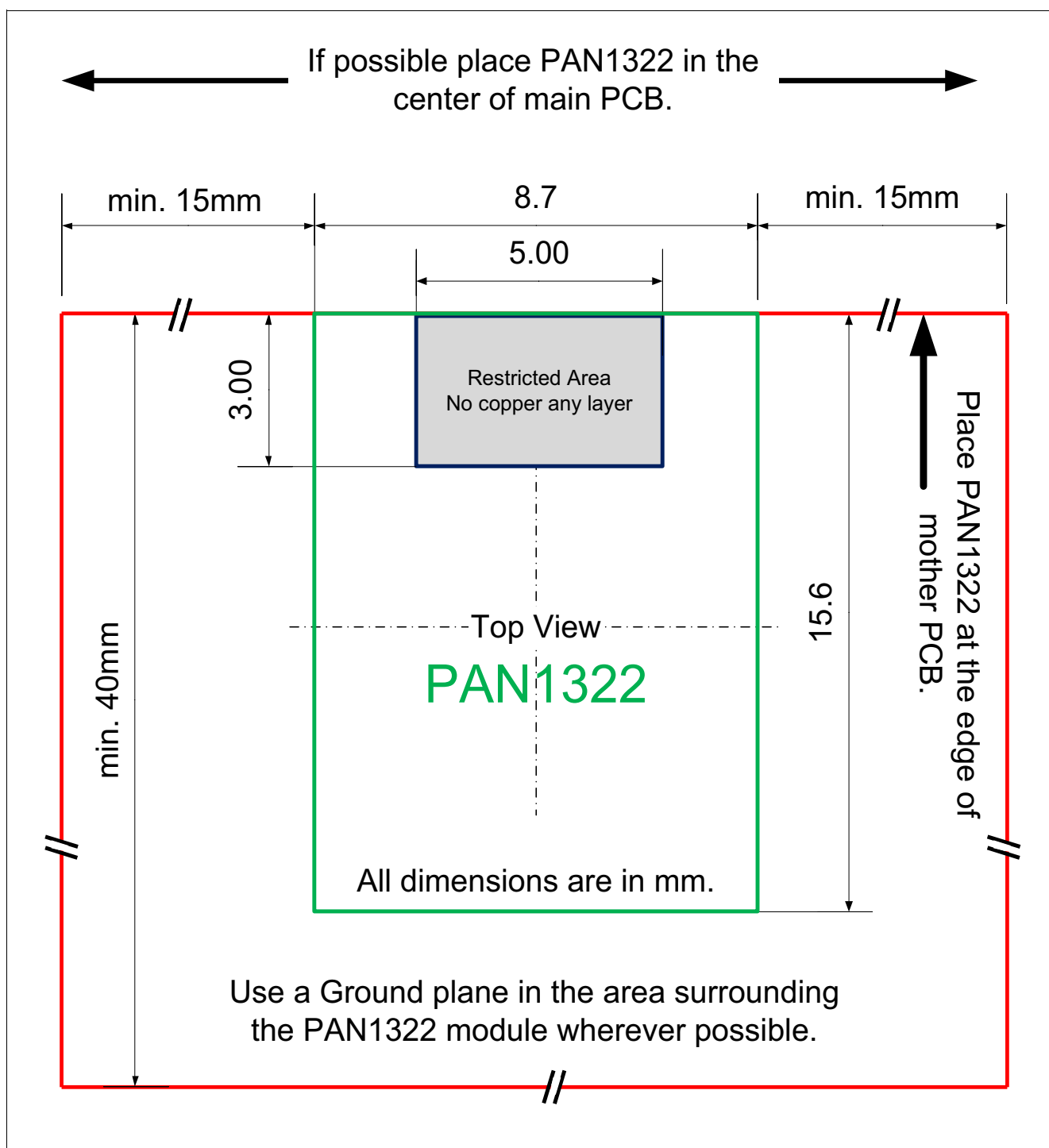
Figure 10 Cutout Drawing
