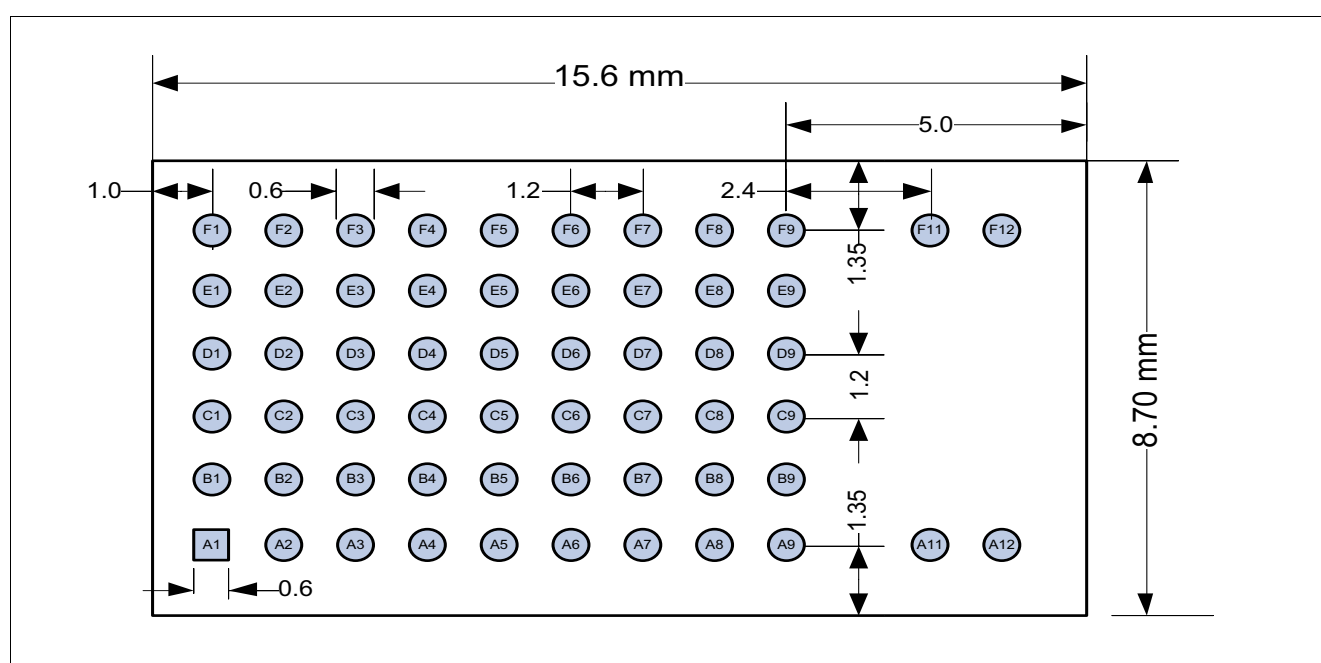
Figure 13 Pad Layout on the Module (top view)
