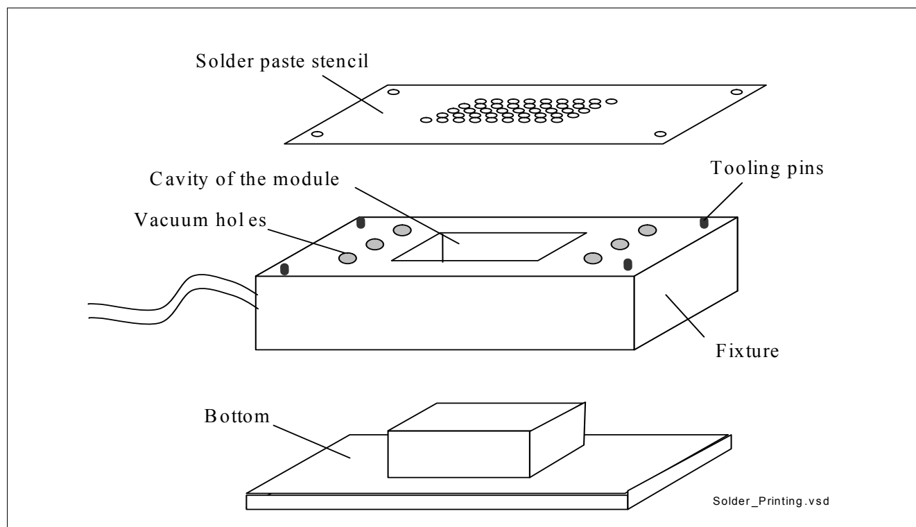
Figure 19 Solder Printing
