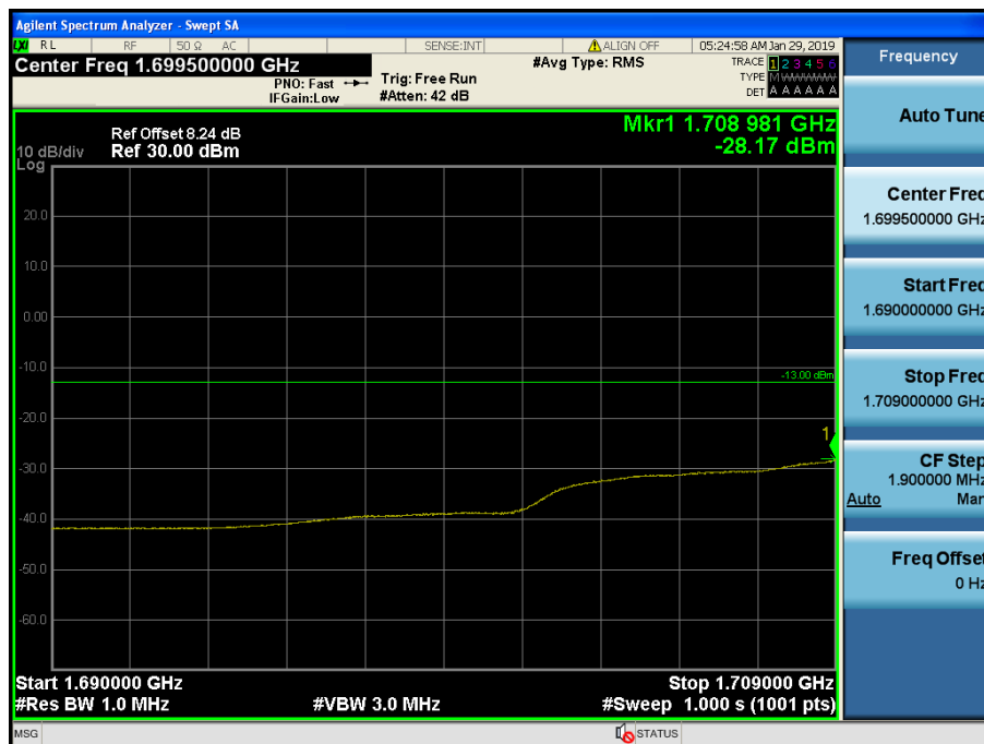
LTE Band 66 / 20MHz / QPSK - RB Size/Offset (50/0)
