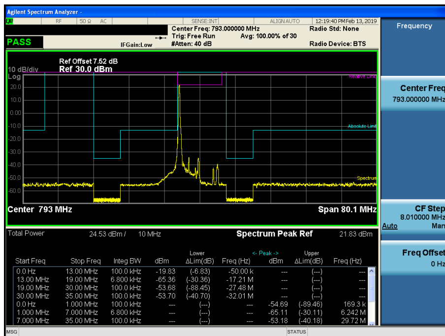
LTE Band 14 / 5MHz / QPSK - RB Size/Offset (1/0)
