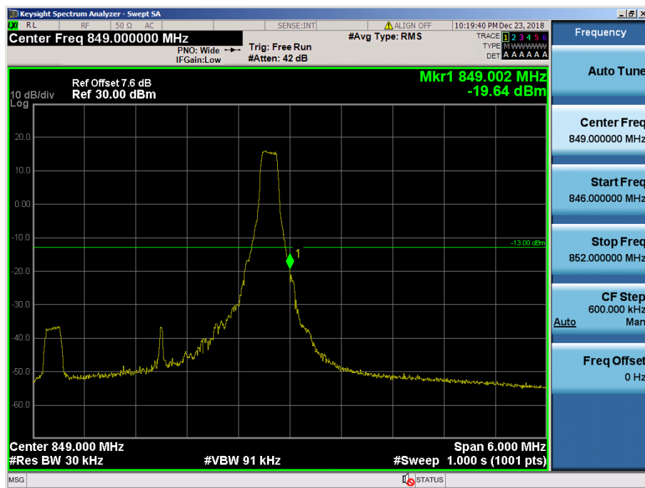
LTE Band 5 / 3MHz / 16QAM - RB Size/Offset (1/7)
