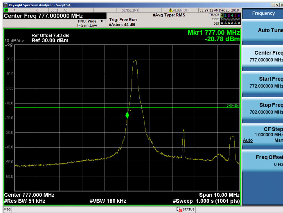
LTE Band 13 / 5MHz / QPSK Offset/Size (1/0)
