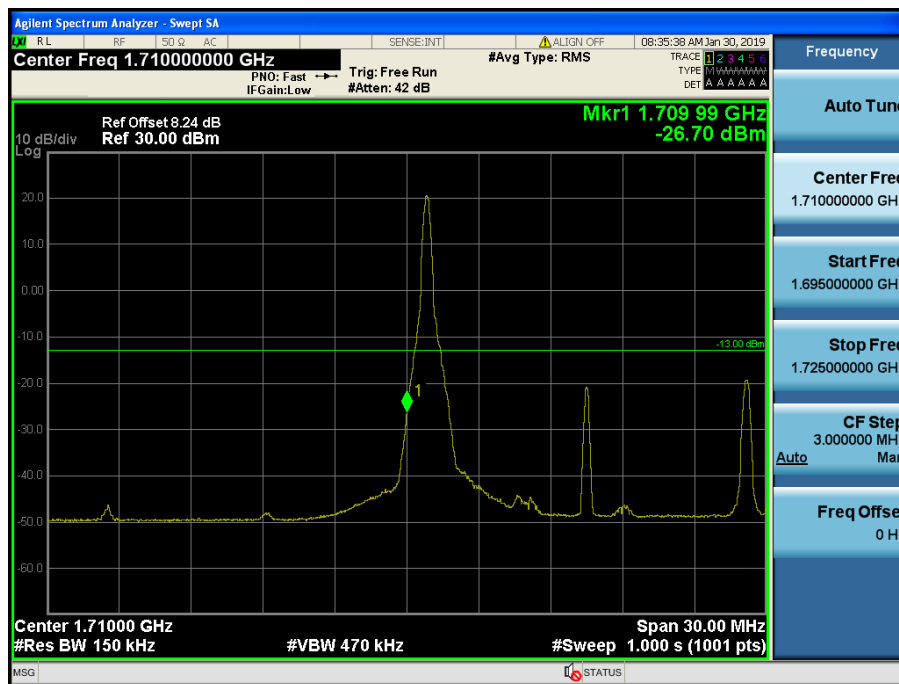
LTE Band 66 / 15MHz / 16QAM - RB Size/Offset (1/0)
