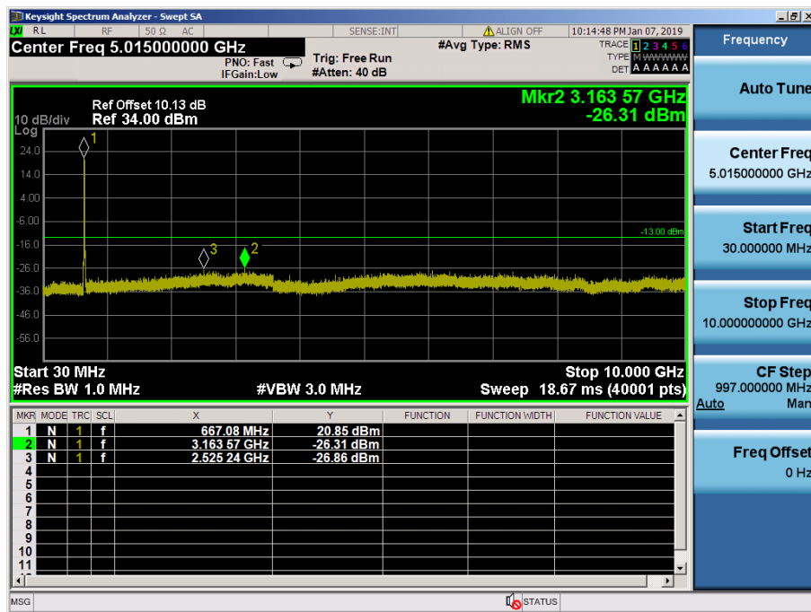
LTE Band 71 / 15MHz / 16QAM - RB Size/Offset (75/0) – Low Channel
