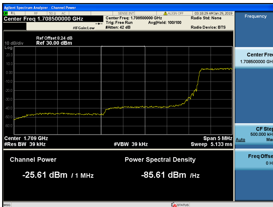
LTE Band 66 / 5MHz / QPSK Offset/Size (12/0)
