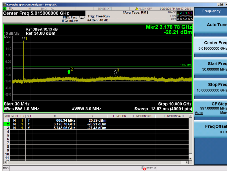
LTE Band 71 / 5MHz / 16QAM - RB Size/Offset (12/6) – Low Channel
