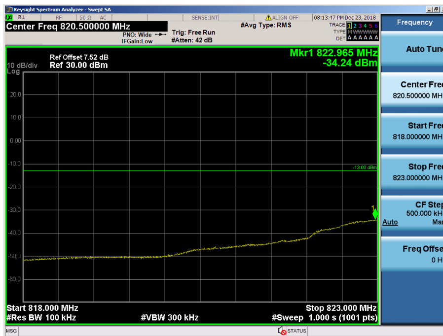
LTE Band 5 / 5MHz / QPSK Size/Offset (12/0)
