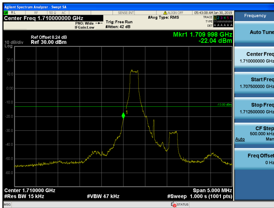
LTE Band 66 / 1.4MHz / 16QAM - RB Size/Offset (1/0)
