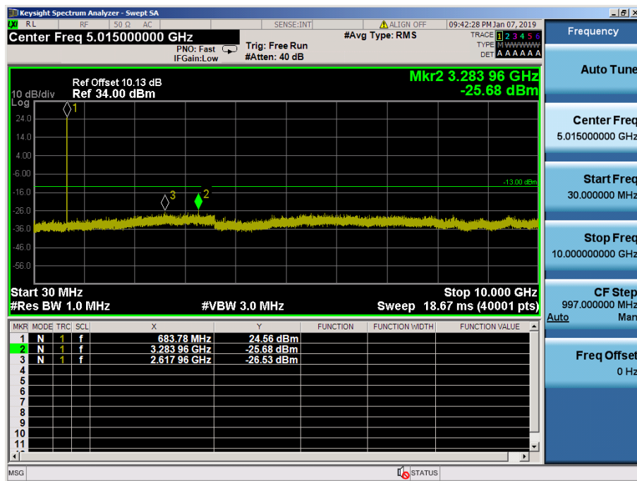
LTE Band 71 / 10MHz / 16QAM - RB Size/Offset (25/25) – Mid Channel
