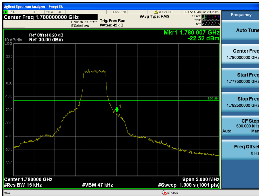
LTE Band 66 / 1.4MHz / QPSK - RB Size/Offset (3/3)
