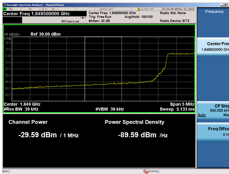
LTE Band 2 / 5MHz / 16QAM Size/Offset (12/0)
