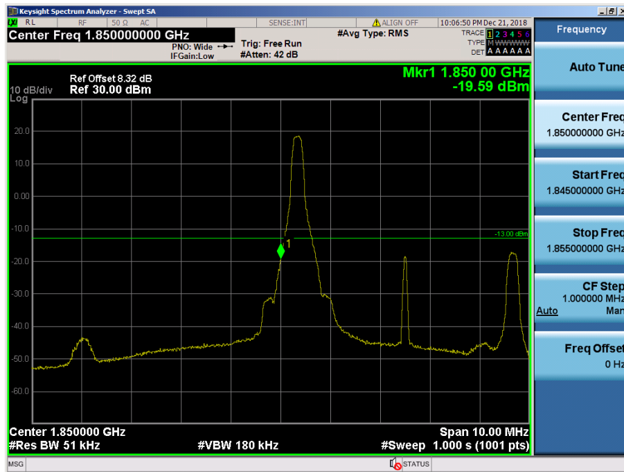
LTE Band 2 / 5MHz / QPSK Size/offset (1/0)
